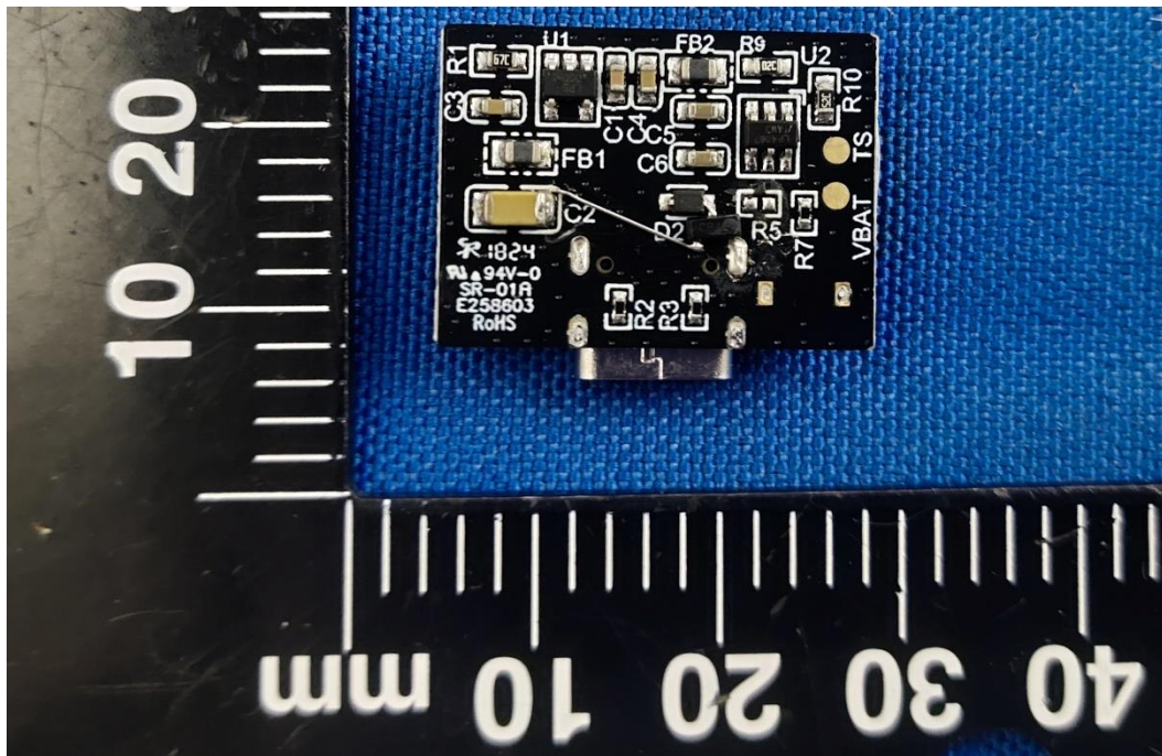
SECONDARY BOARD 1 REAR VIEW
