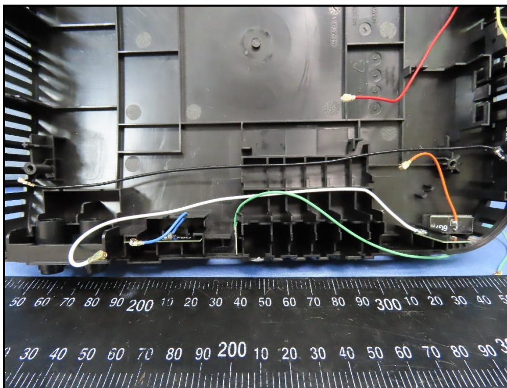
DB2 antenna
