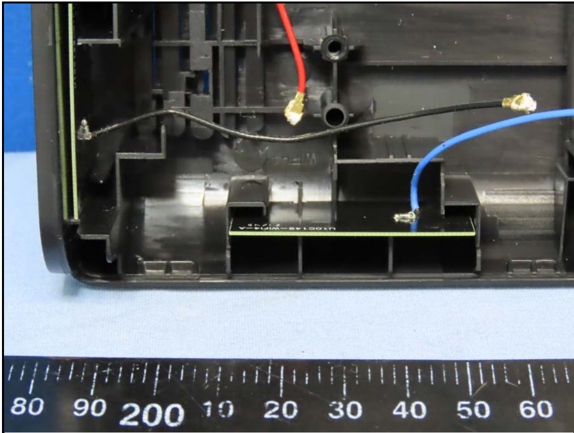
Antenna WIFI 3
