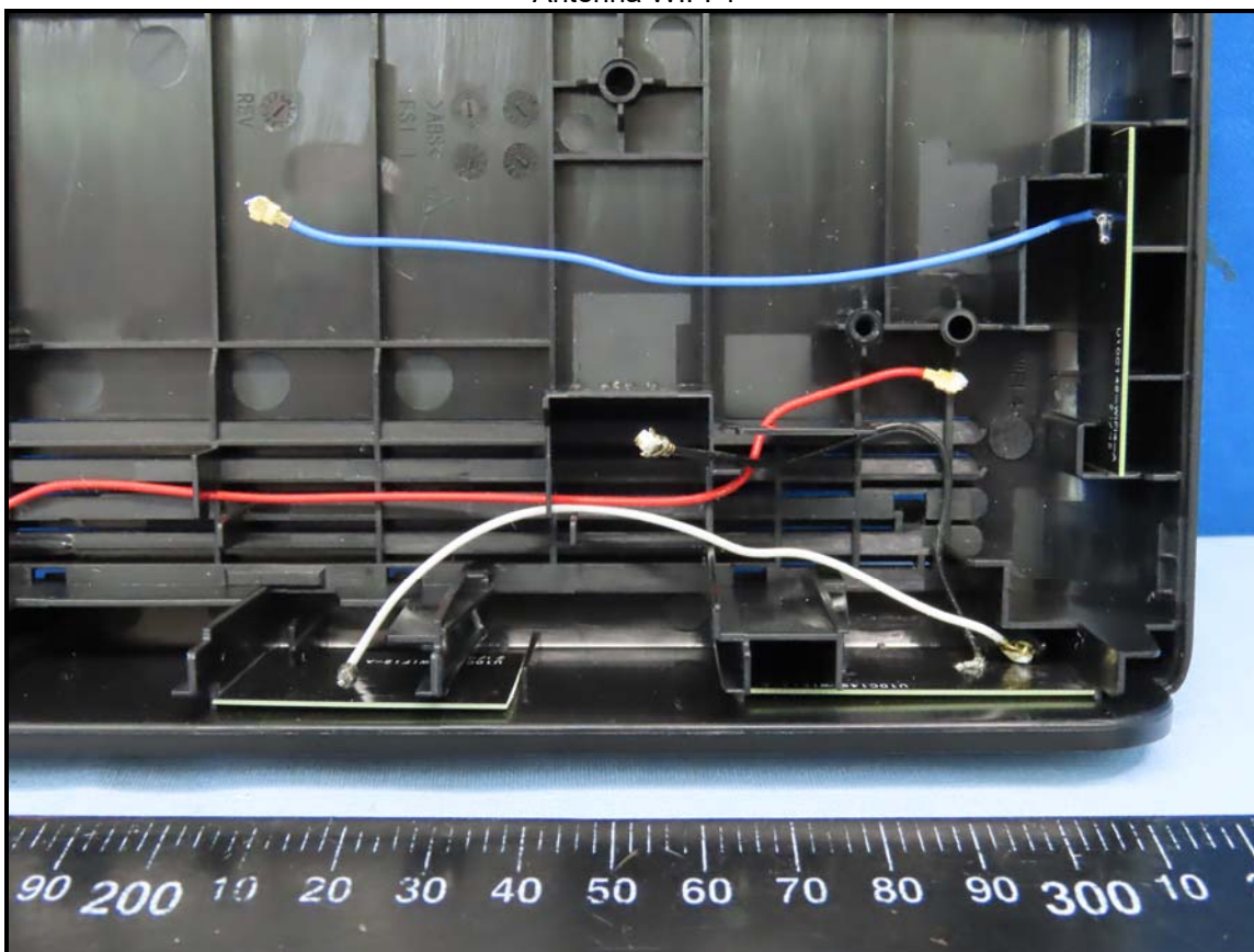
Antenna WIFI 4
