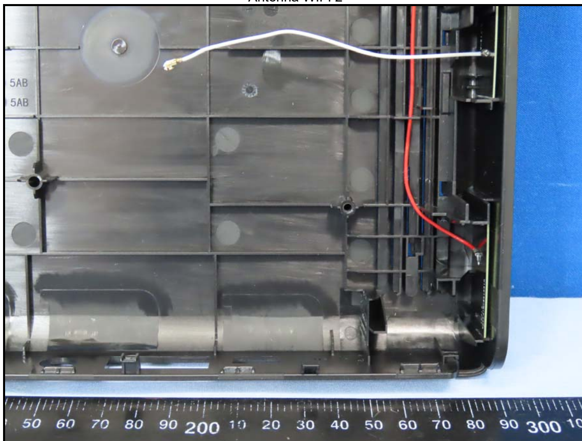
Antenna WIFI 2
