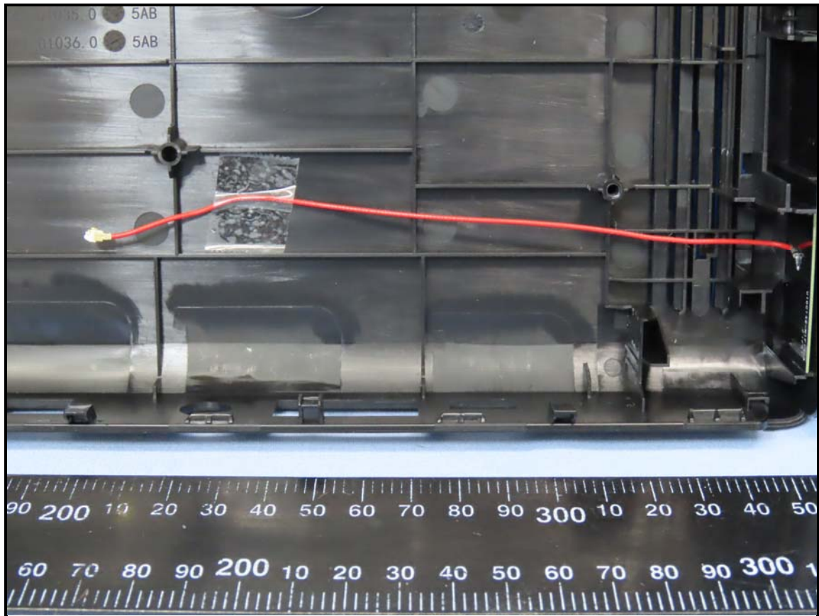
Antenna WIFI 1
