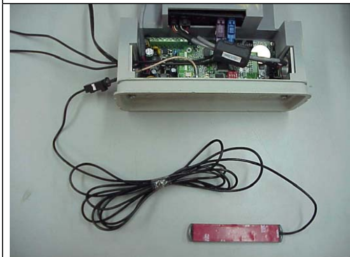
External connector and antenna.
