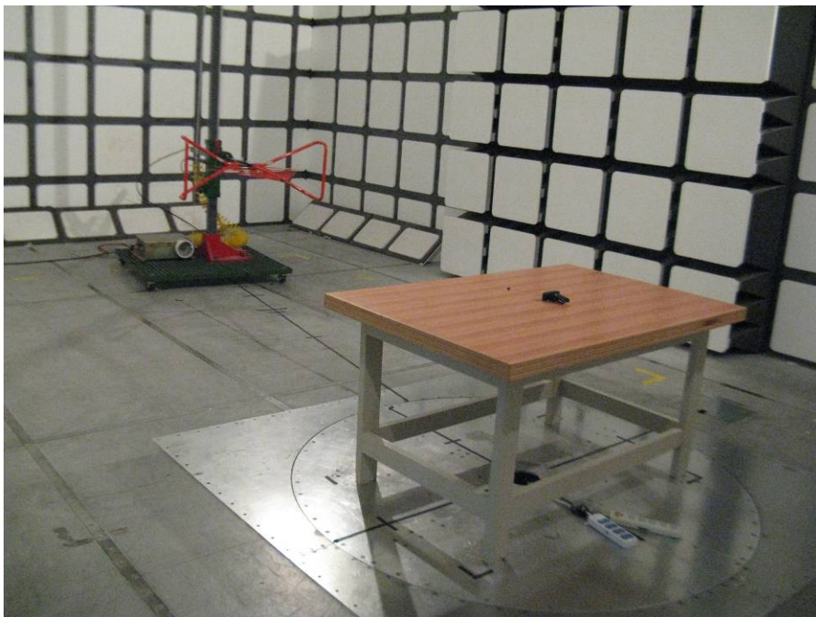
Radiated Emissions - Lie View
