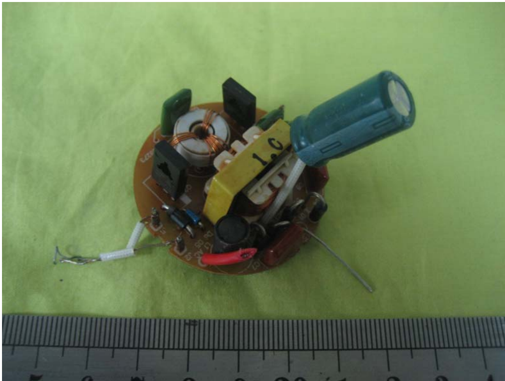
Internal photo of EU-23W -1
