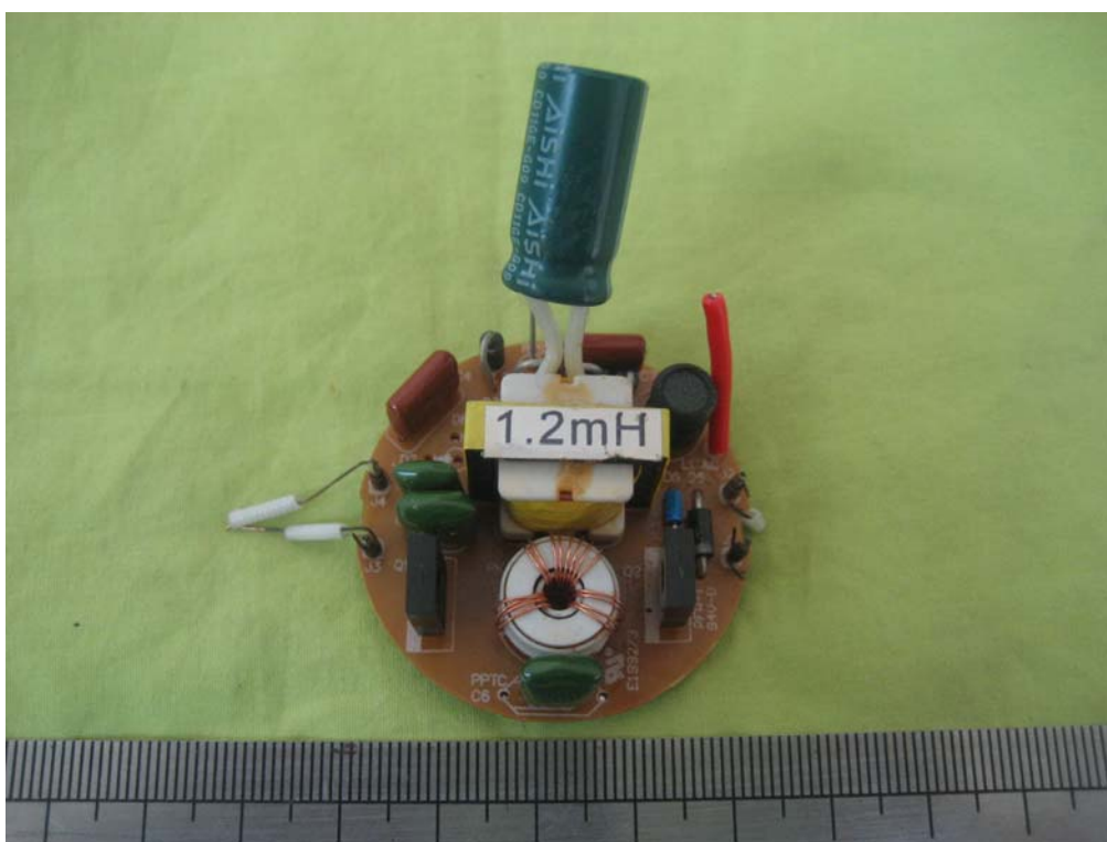
Internal photo of EU-19W - 1
