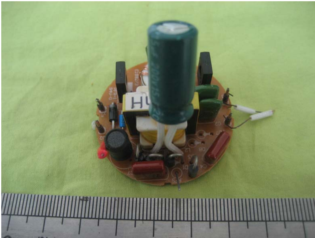
Internal photo of EU-19W – 2
