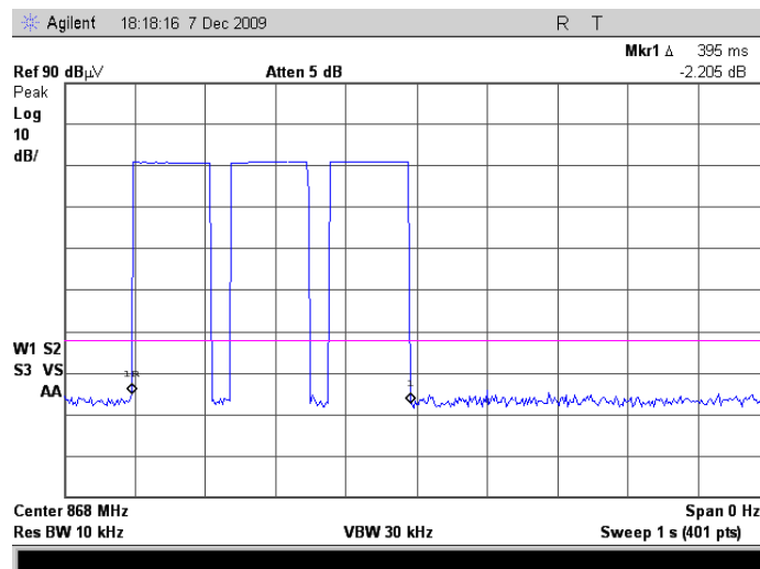
Plot 7.1.3 Transmitter shut down test result – burst duration
