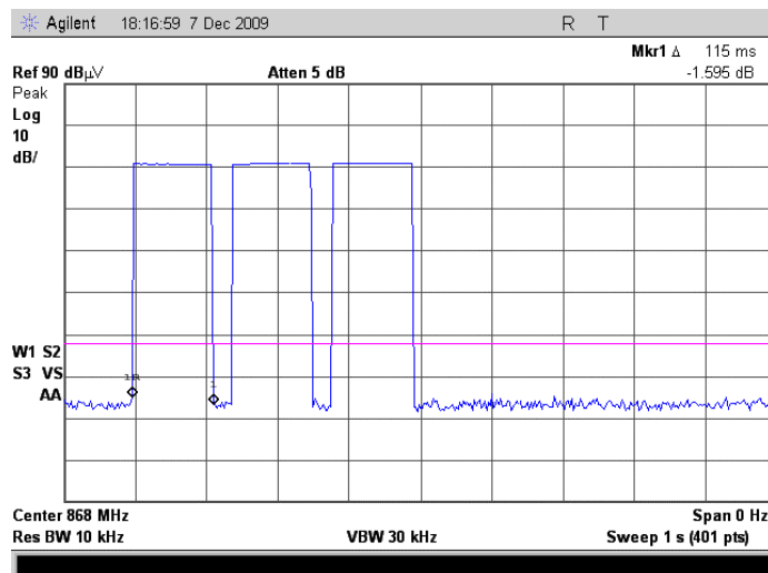
Plot 7.1.2 Transmitter shut down test result – pulse duration
