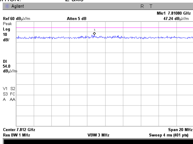
Plot 7.2.20 Radiated emission measurements at the ninth harmonic frequency
