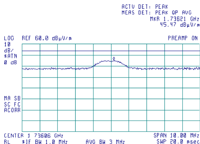
Plot 7.2.14 Radiated emission measurements at the second harmonic frequency
