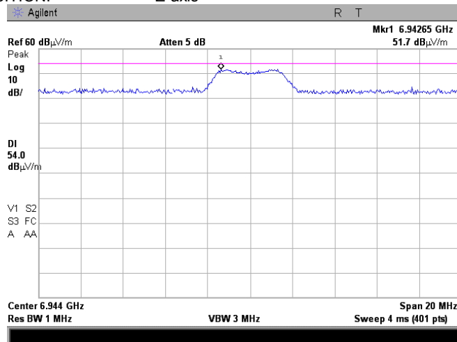
Plot 7.2.18 Radiated emission measurements at the eighth harmonic frequency
