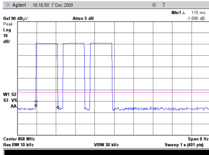
Plot 7.2.23 Transmission pulse duration
