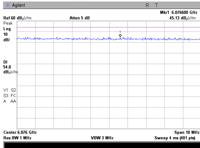
Plot 7.2.16 Radiated emission measurements at the seventh harmonic frequency
