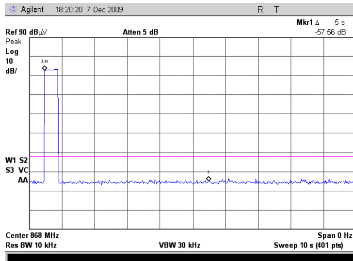
Plot 7.2.26 Transmission pulse period
