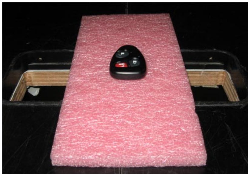
Photograph 6.1.2 EUT in "Y-axis" orthogonal position
