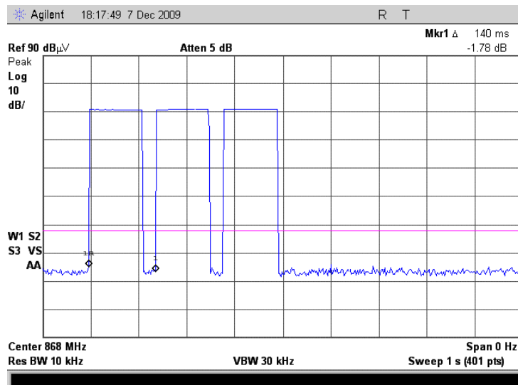
Plot 7.2.24 Transmission pulse period
