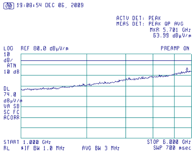
Plot 8.1.6 Radiated emission measurements from 1000 to 6000 MHz, horizontal antenna polarization
