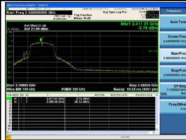
802.11n-20M CH01 (2412MHz)
