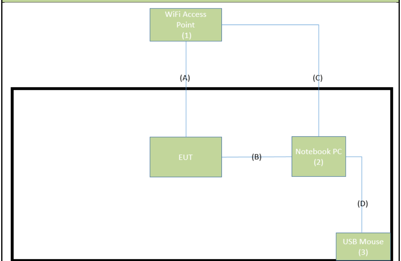
Connection Diagram (Adapter Mode)
