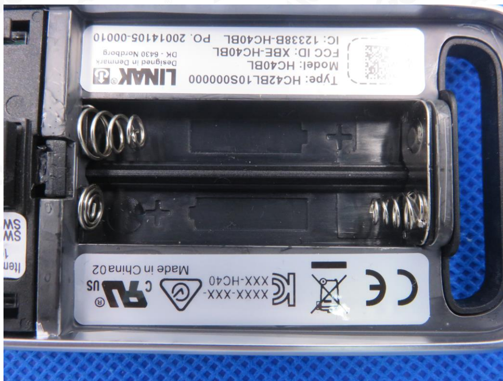
Fig.40 -battery compartment view (type: HC42BL10S000000)
