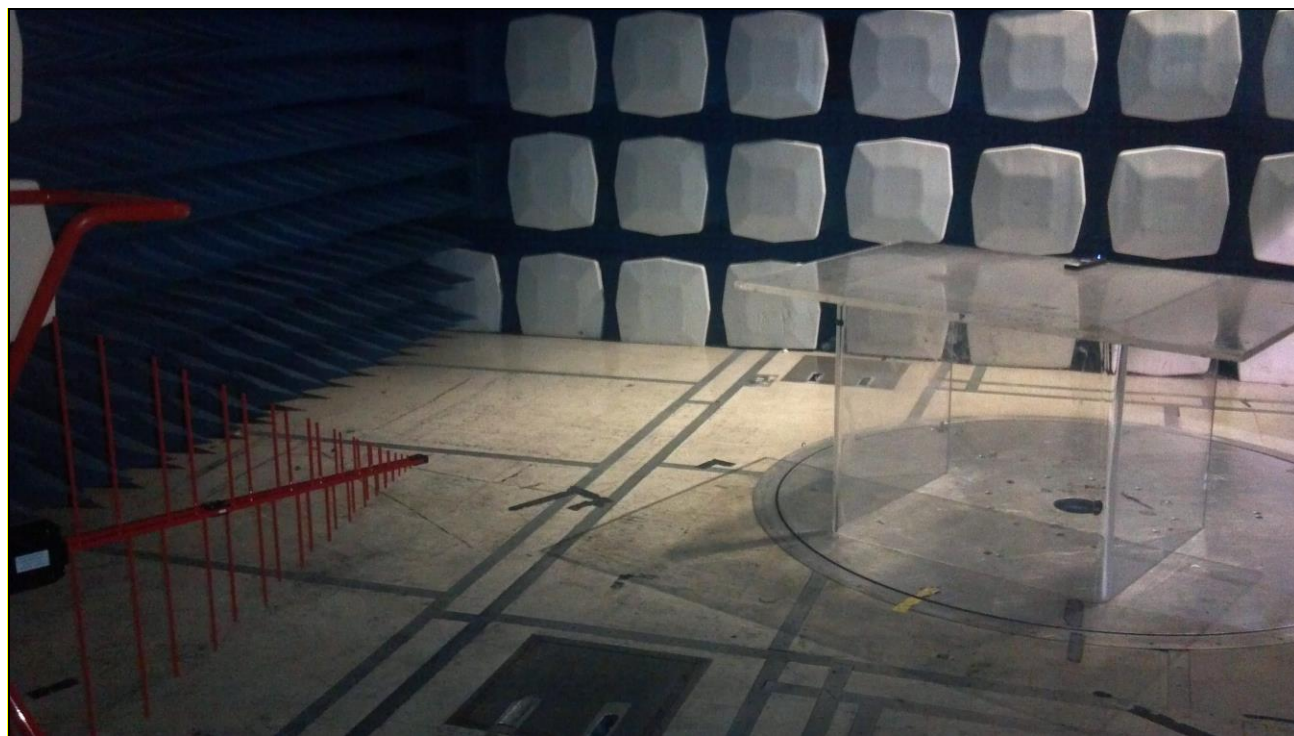
Photograph 2. Radiated Emissions Limits, Test Setup
