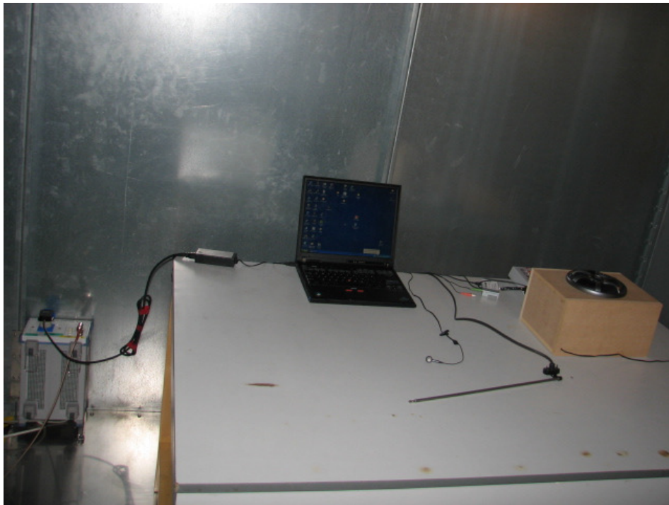
Setup for conducted emission (Streaming music mode)
