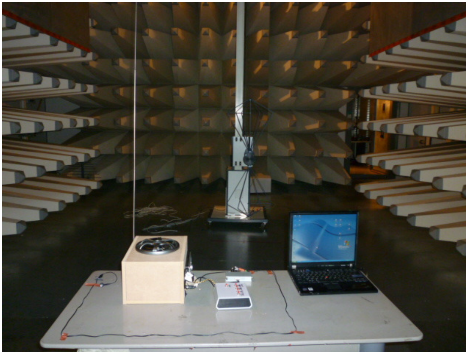
Setup for radiated emission (PC linked Mode)
