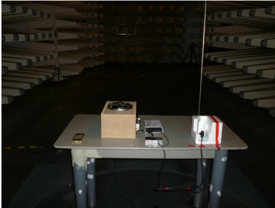
Setup for radiated emission (Streaming music mode)
