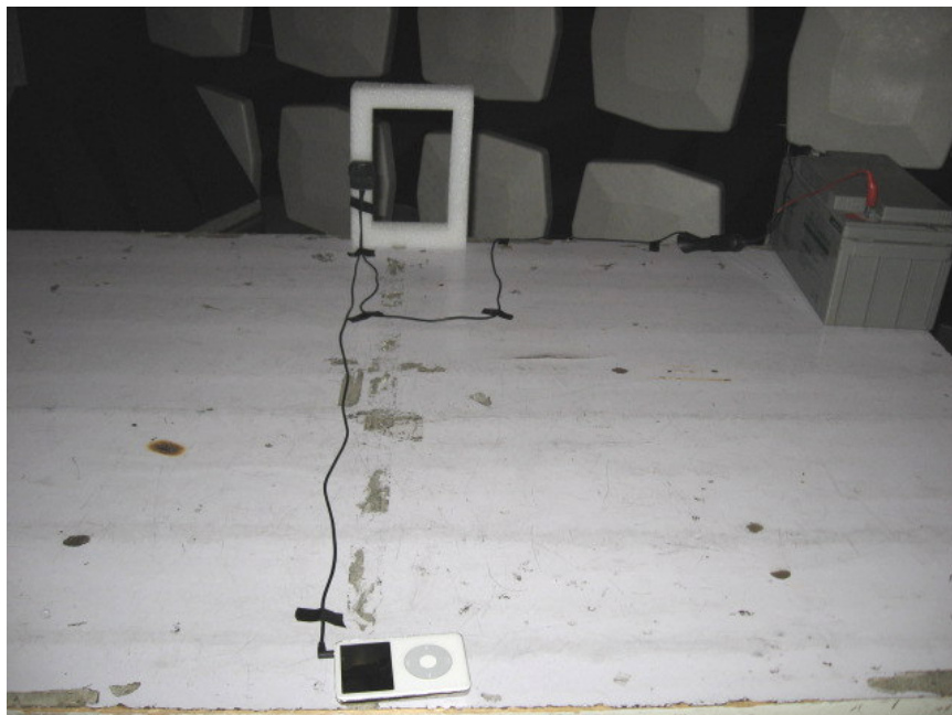
Final test setup photograph
