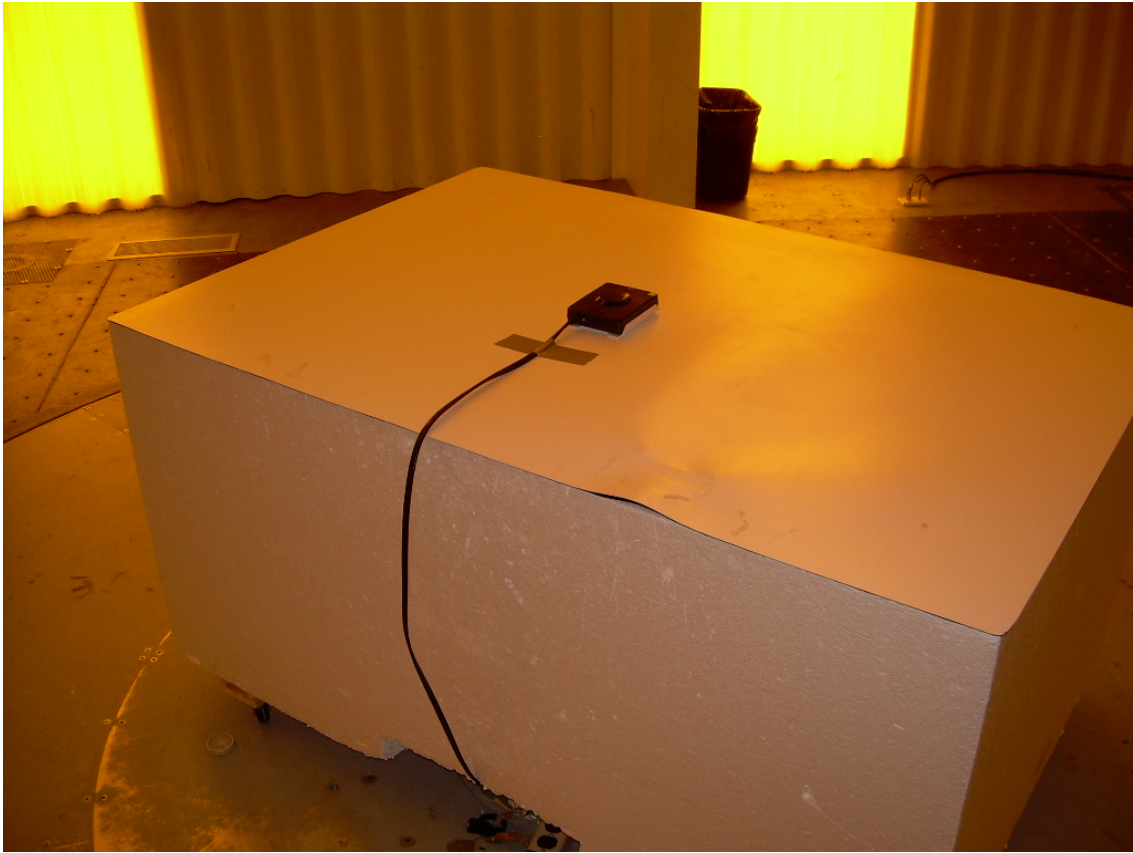
Back View Radiated Disturbance Worst Case Configuration - Horizontal Placement
