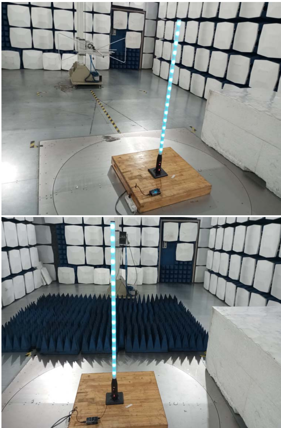
Radiated emission test view
