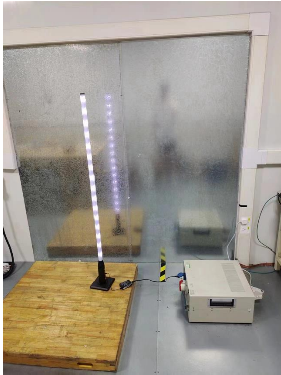
Conducted Emission Test Setup:
