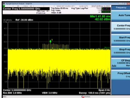
Radar 2
