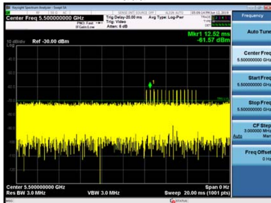
Radar 4
