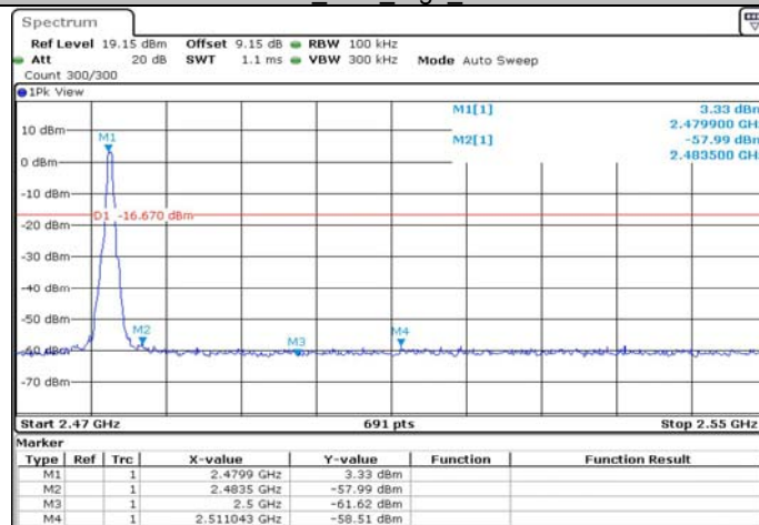
DH1_Ant1_High_2480
