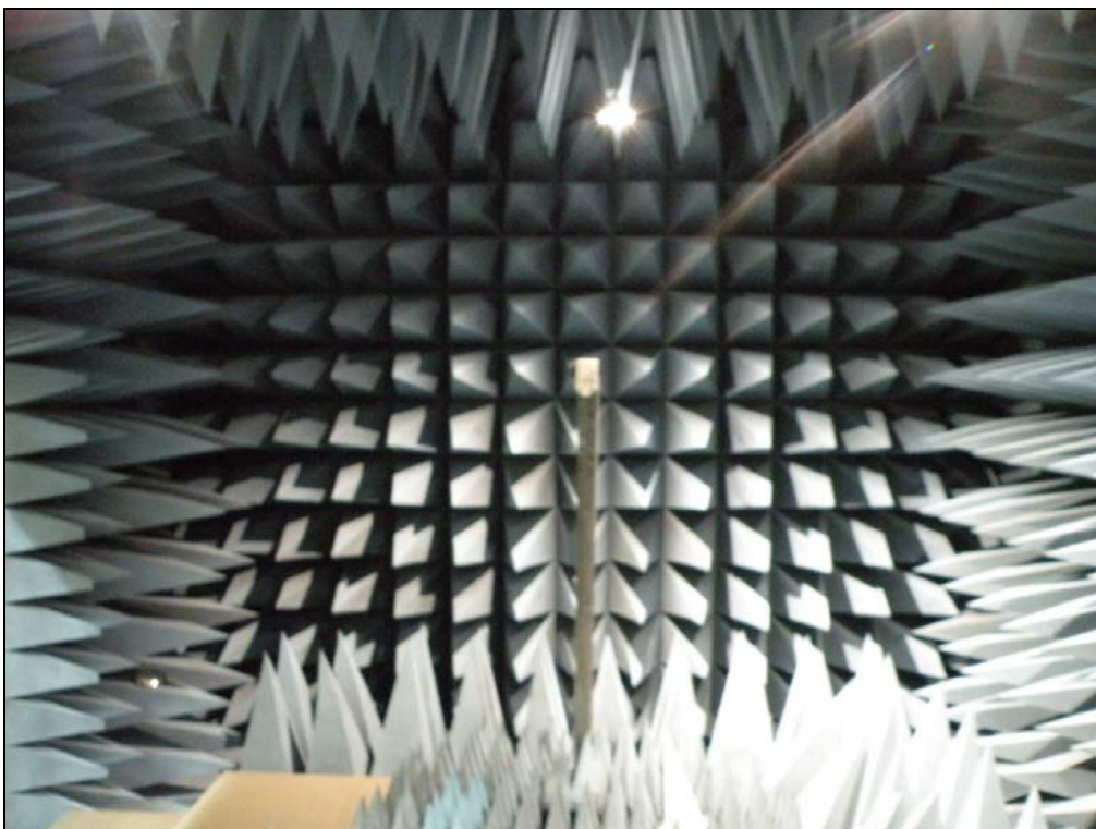
- Effective Radiated Power test -
