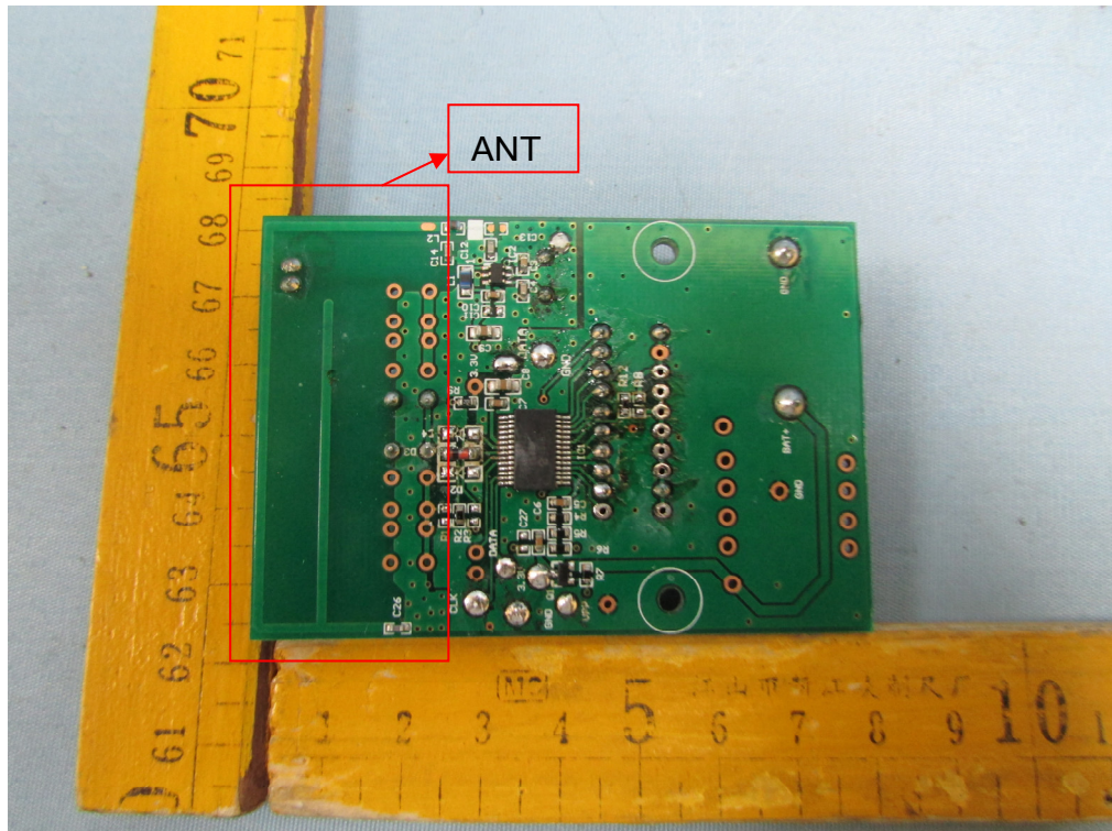
Model P220-2- Internal View
