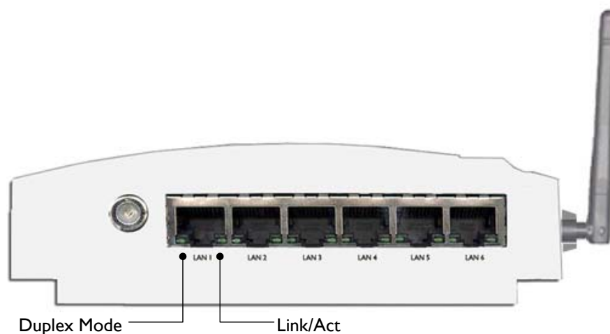
FIGURE 4: FRONT VIEW OF AT-IMG616WCRF
