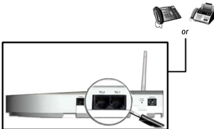
FIGURE 9: TELEPHONE PORTS CONNECTION
