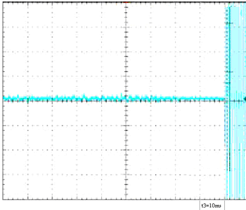
Transmitter Frequency Behaviour @ 12.5 KHz Channel Separation--Off to On
