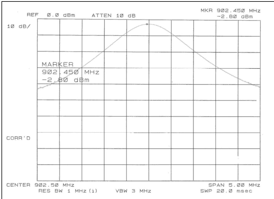
Figure 24 Maximum Peak Output Power Graph – Low Channel
