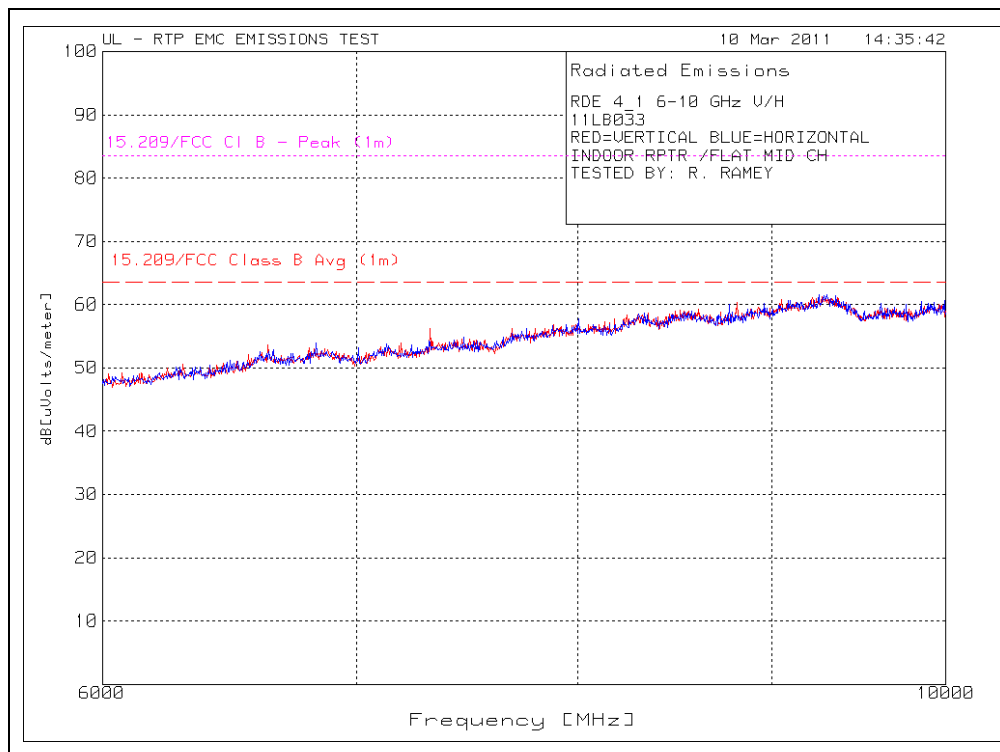
Figure 9B Radiated Spurious Emissions, Middle Channel (Flat-Orientation)
