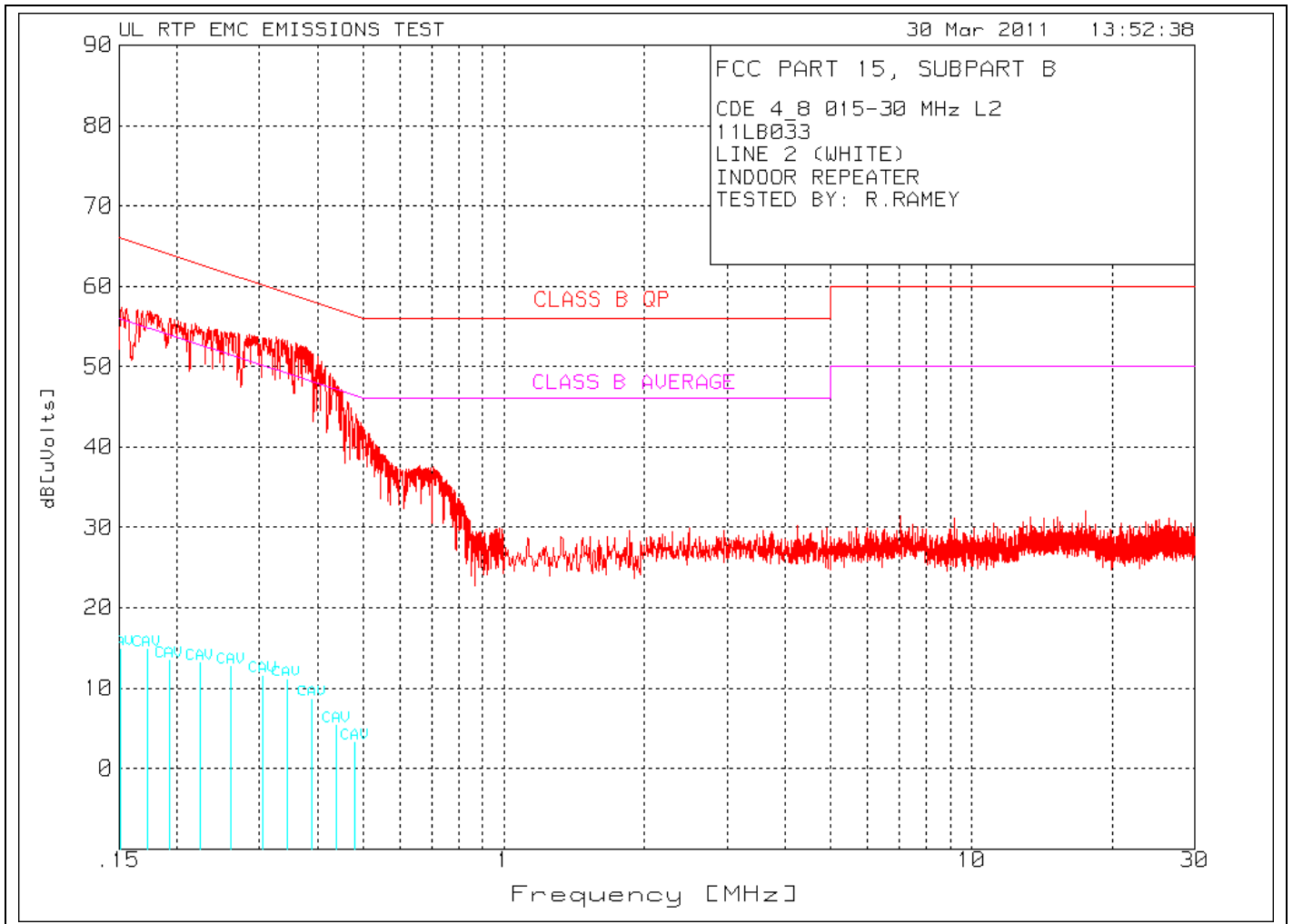
Figure 43 Conducted Emissions Graph – Neutral Conductor
