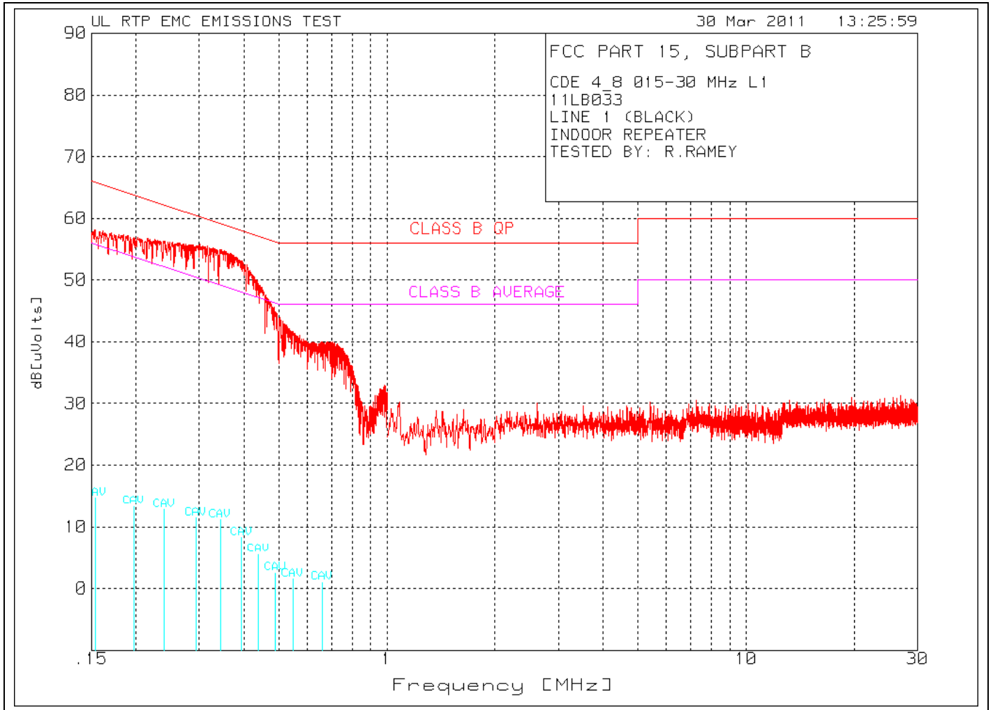
Figure 39 Conducted Emissions Graph – Line Conductor
