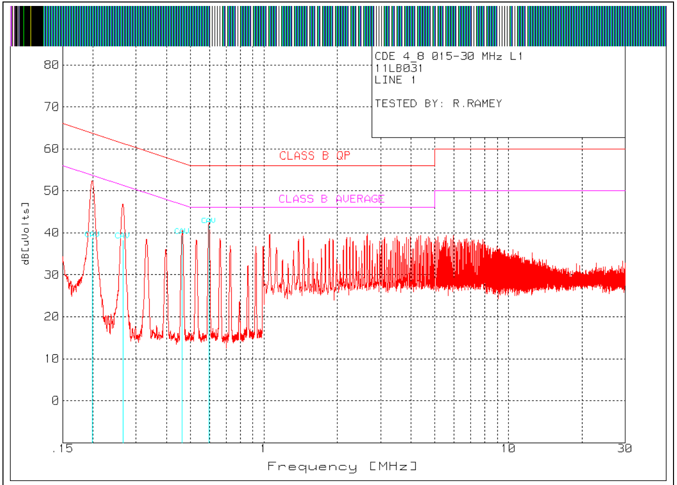
Figure 38 Conducted Emissions Graph – Line Conductor
