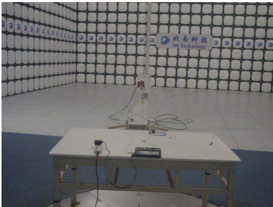
Set-up for radiated emission test (Above 1GHz)
