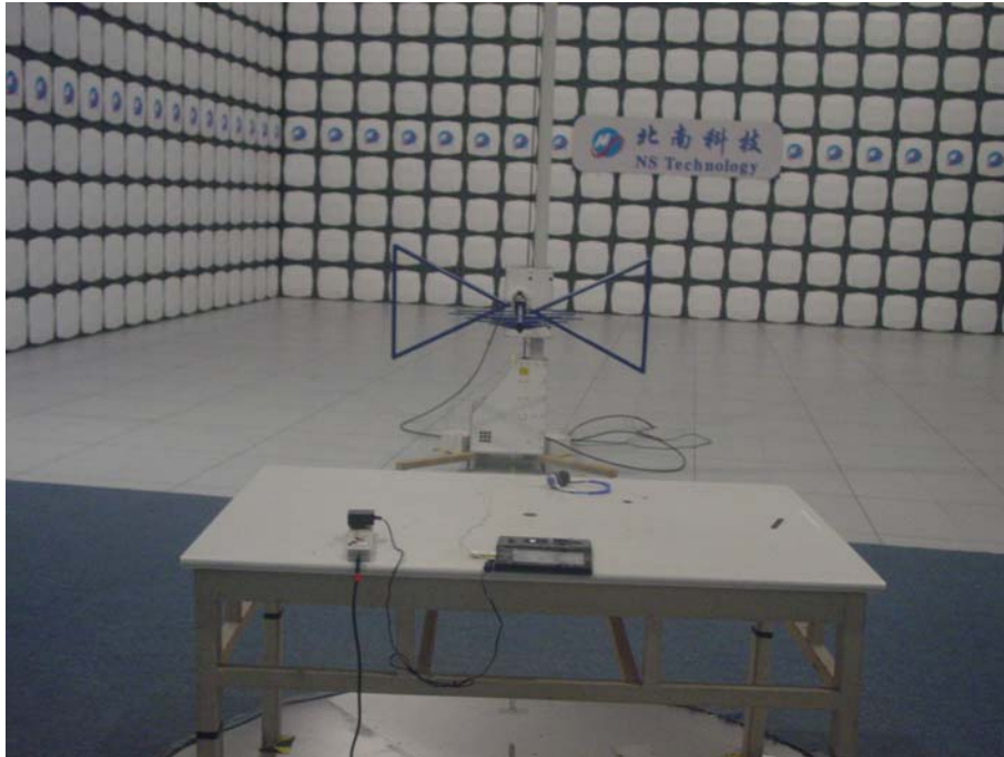
Set-up for radiated emission test (30MHz~1GHz)
