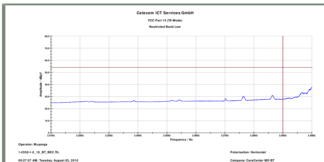
Plot 1: Lower Restricted Band / GFSK (radiated)
