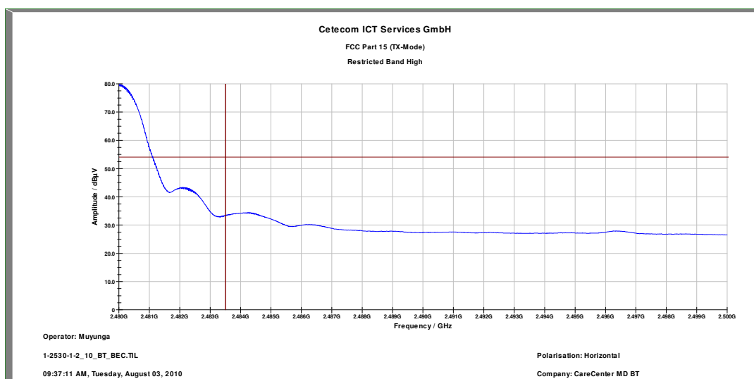
Plot 2: Upper Restricted Band / GFSK (radiated)
