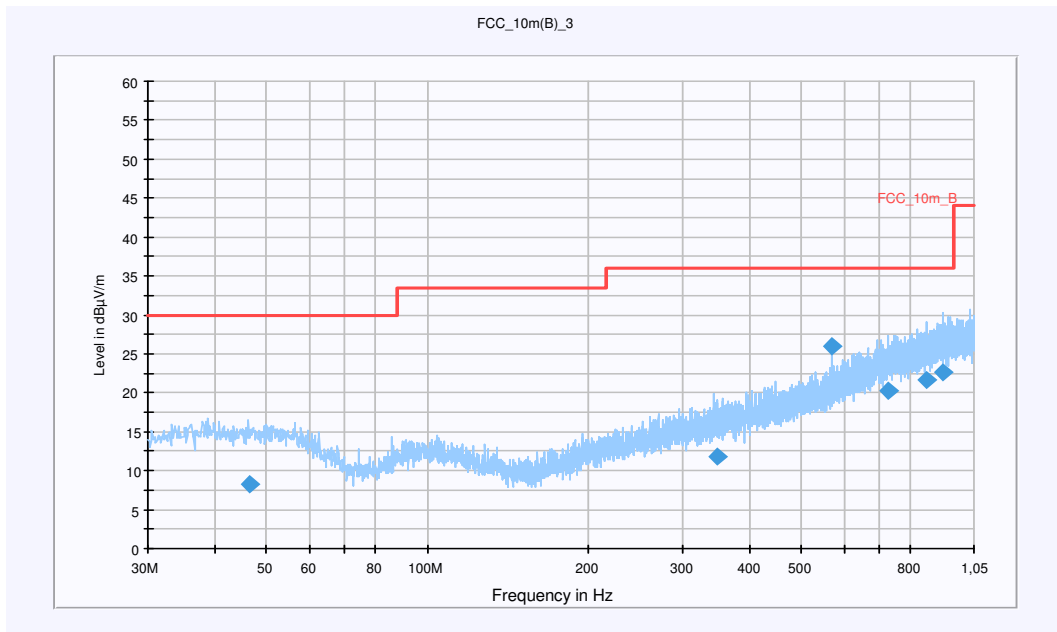
Plot 1: 30 MHz to 1 GHz / Channel 00 (horizontal/vertical)
