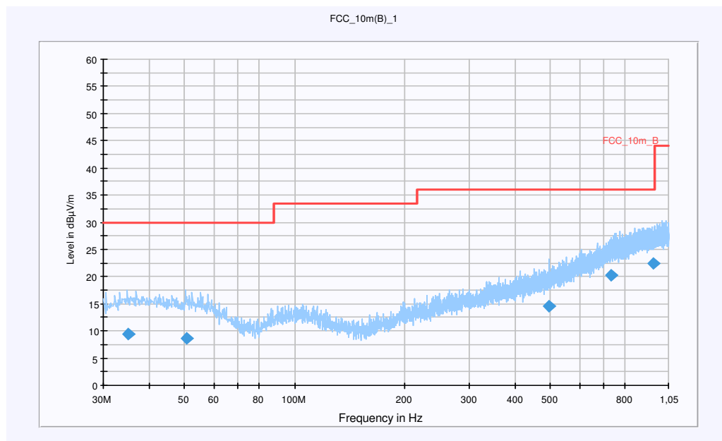
Plot 1: 30 MHz to 1 GHz / Idle-mode (horizontal/vertical)
