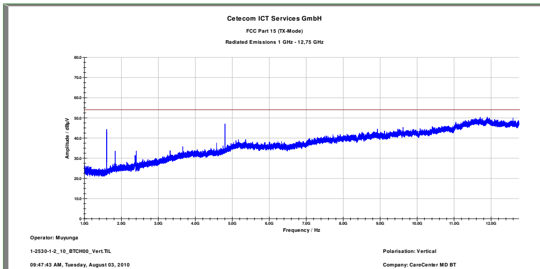
Plot 2: 1 GHz to 12.75 GHz / Channel 00 (horizontal/vertical)
