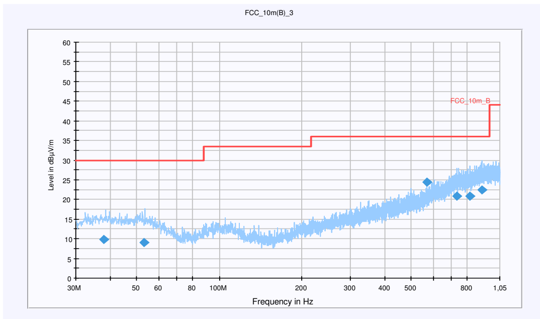
Plot 6: 30 MHz to 1 GHz / Channel 78 (horizontal/vertical)
