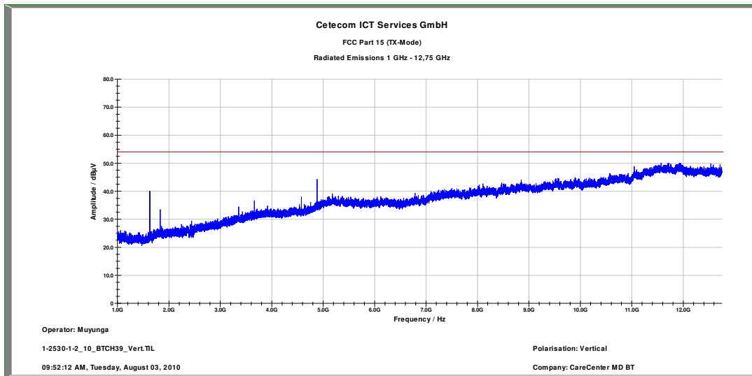
Plot 5: 1 GHz to 12.75 GHz / Channel 39 (horizontal/vertical)
