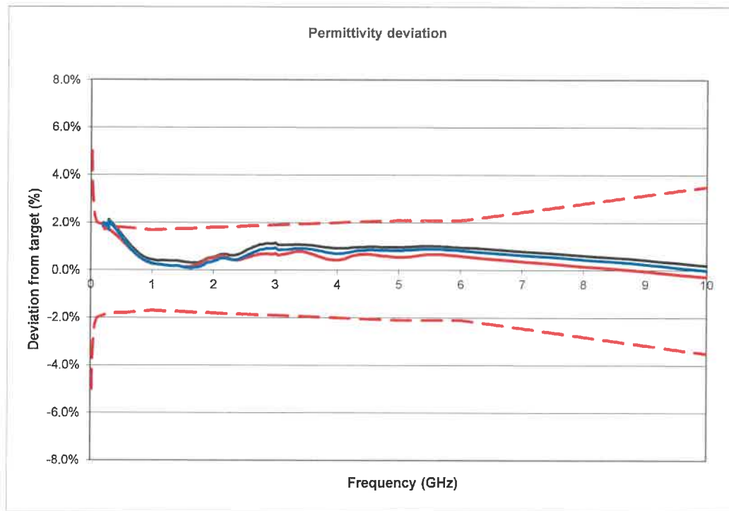
Fig. 3.1 Ethanol permittivity deviation from target, 200 MHz – 10 GHz
