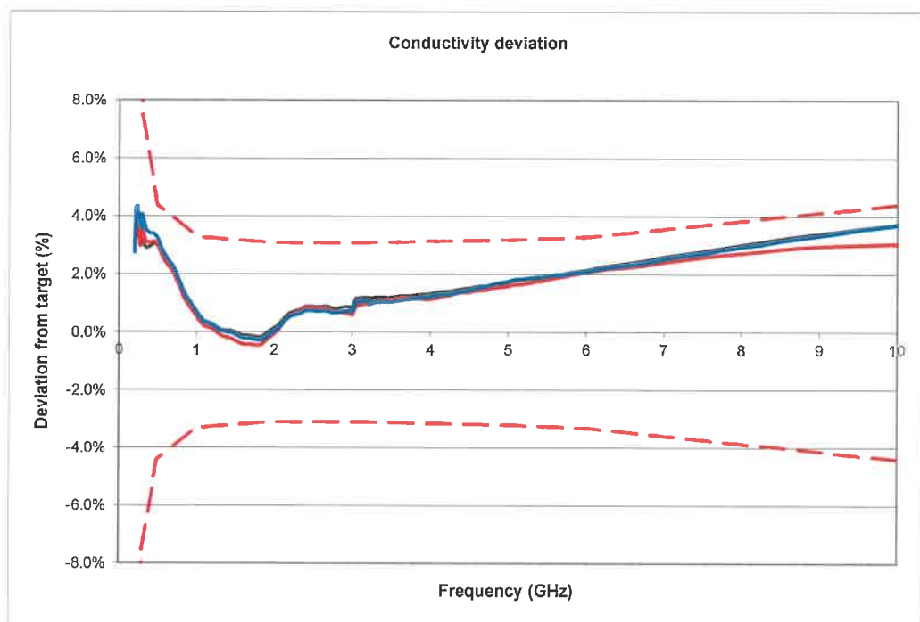
Fig. 3.2 Ethanol conductivity deviation from target, 200 MHz – 10 GHz
