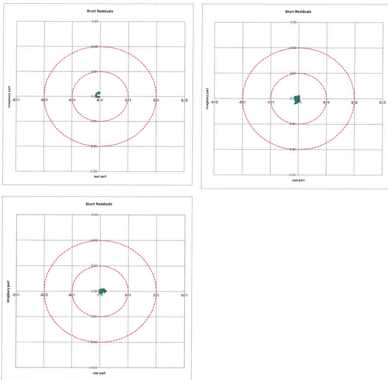
Fig. 2.2a-c Complex representation of the residuals of the shorts, 200 MHz - 20 GHz, after calibrations a)-b) in the top and c) in the bottom
