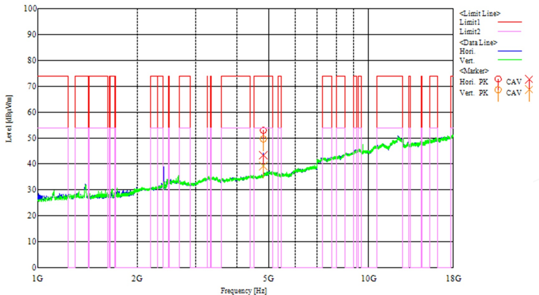
[Chart (2402MHz, 1Mbps, X-plane)]
