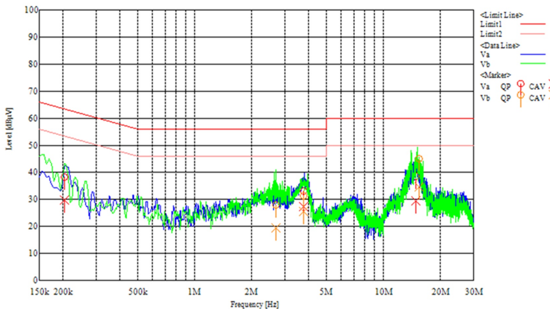
[Chart (2480MHz, 1Mbps)]
