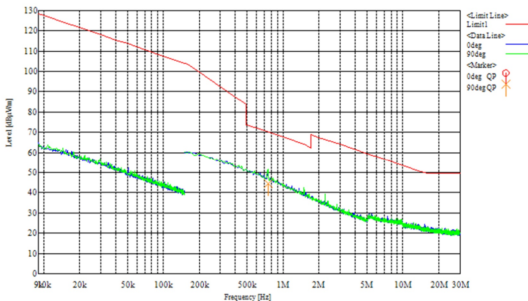
[Chart (2442MHz, 1Mbps, Y-plane)]
