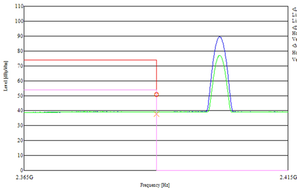
[Chart (2402MHz, 1Mbps, X-plane)]
