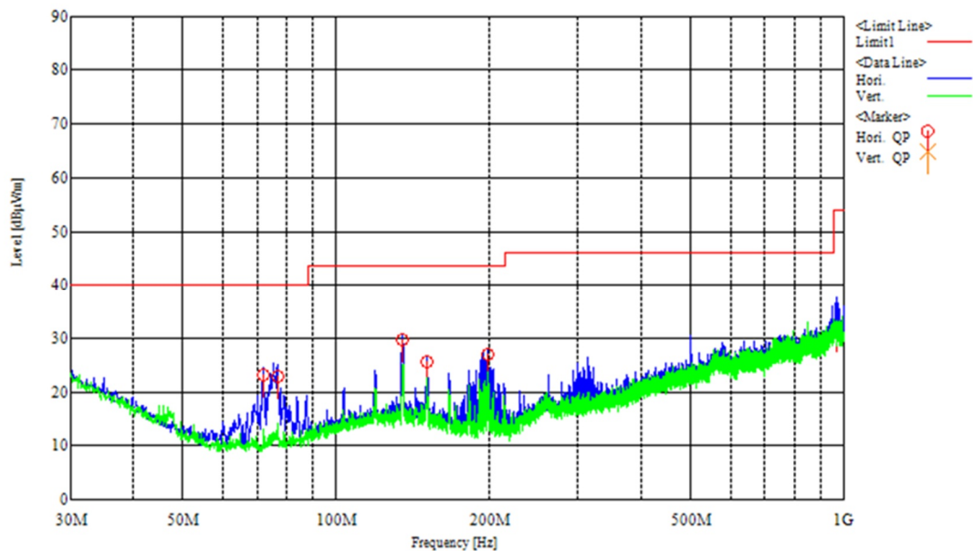
[Chart (2480MHz, Y-plane)]
