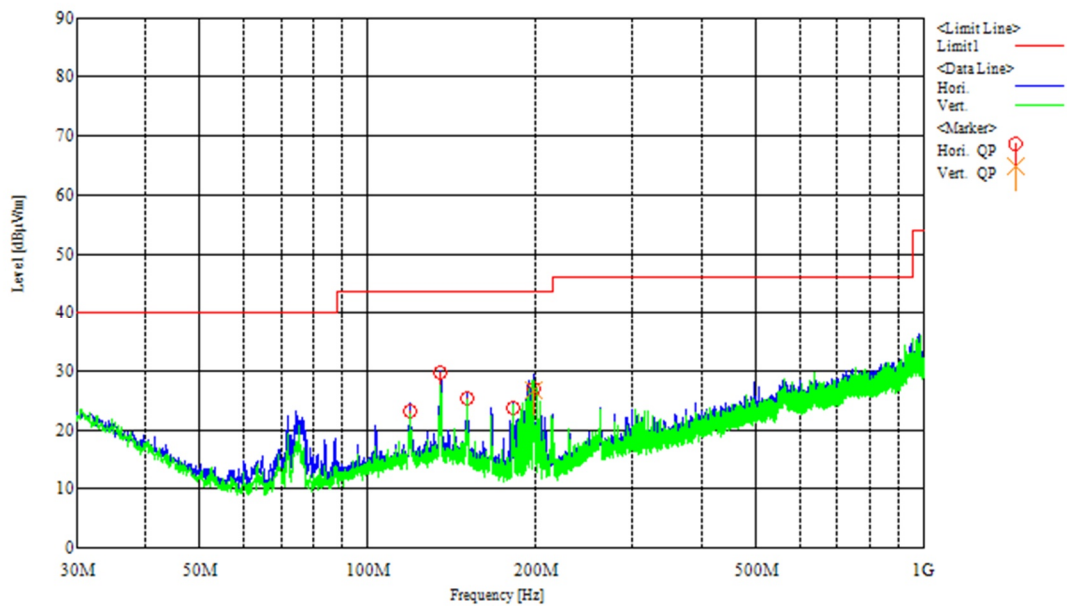
[Chart (2480MHz, 2Mbps, Y-plane)]
