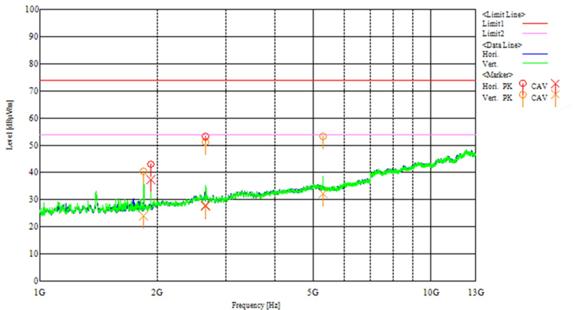
[Chart (2402MHz, Z-plane)]
