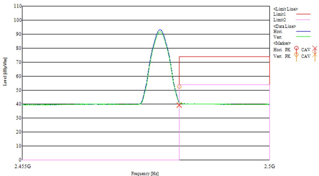
[Chart (2480MHz, 2Mbps, Y-plane)]
