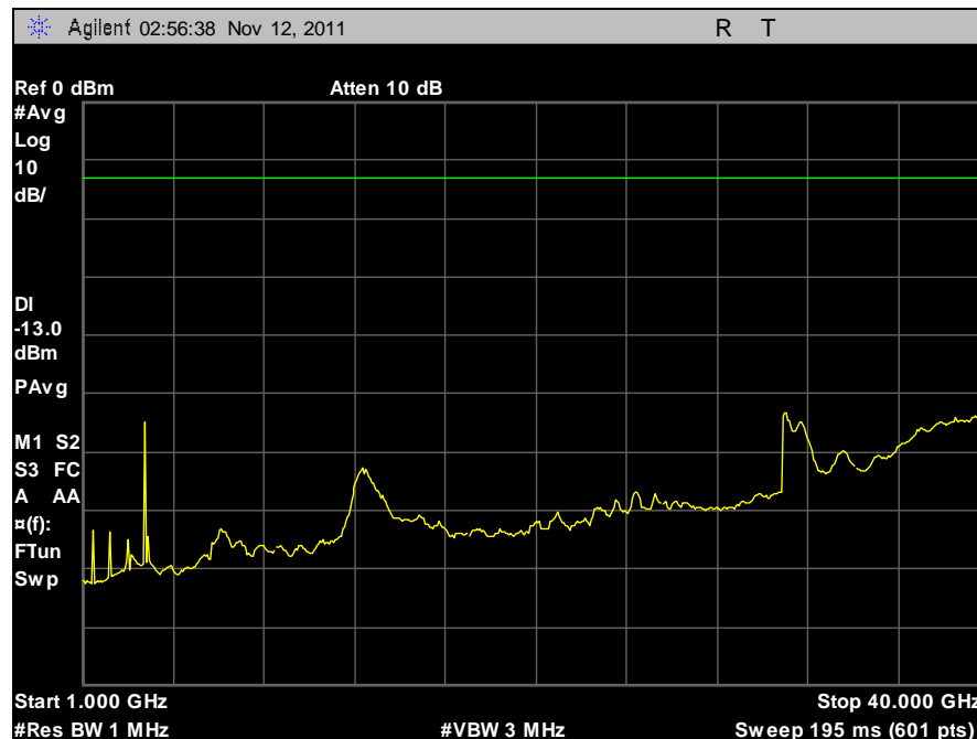
Plot 43. Conducted Spurious Emissions, 5 MHz, Low Channel, Horizontal,, 1 GHz – 40 GHz
