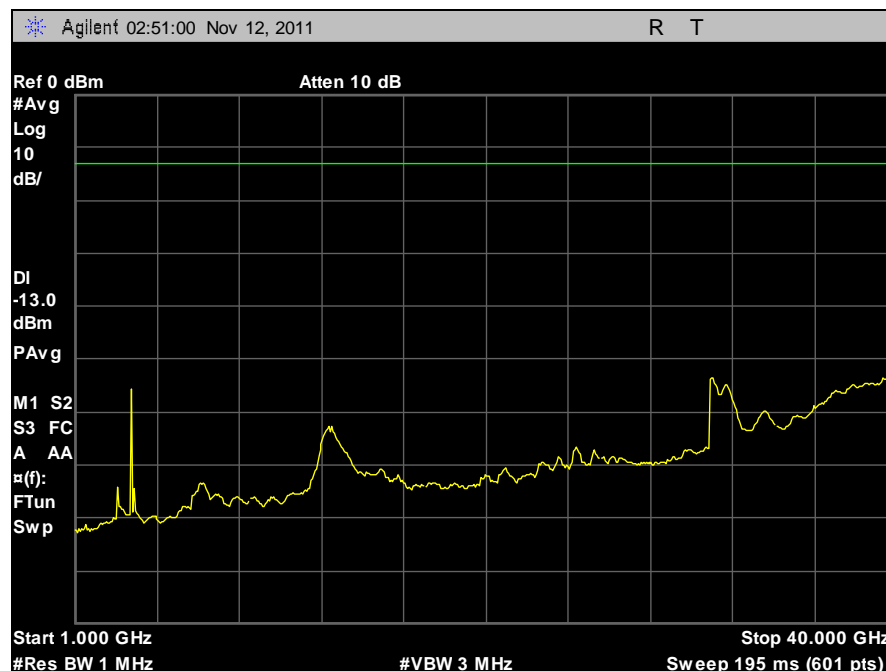
Plot 61. Conducted Spurious Emissions, 20 MHz, Low Channel, Vertical, 1 GHz – 40 GHz
