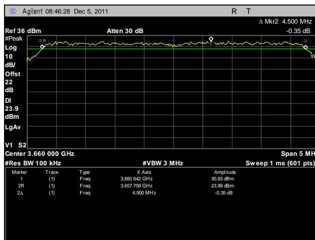
Plot 91. Frequency Stability, 3660 MHz, 120V, 30°C
