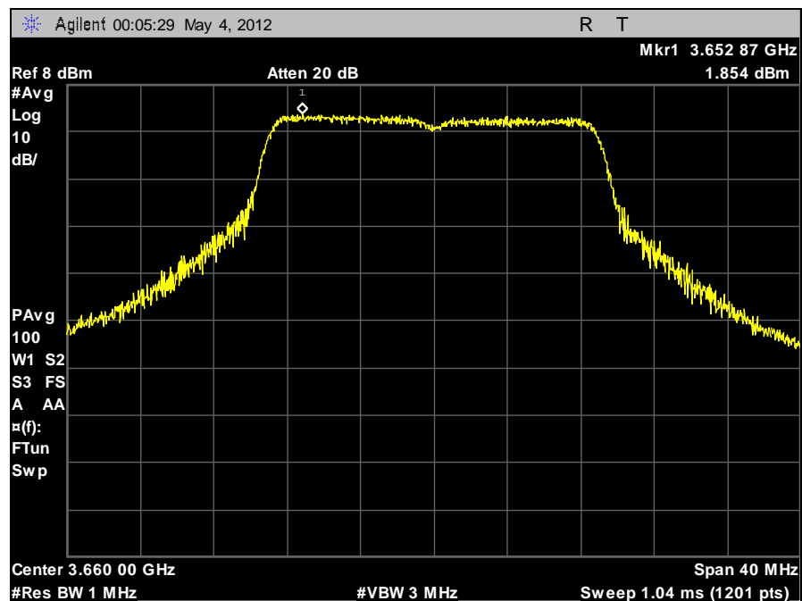
Plot 27. Peak Power Spectral Density, 20 MHz, Low Channel, Vertical
