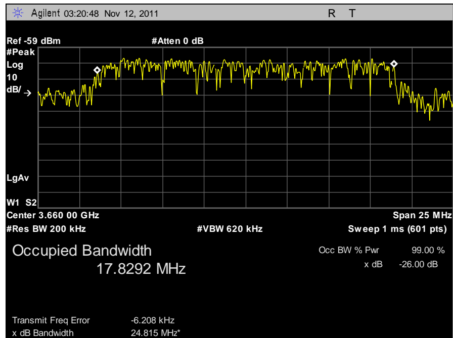
Plot 38. 99% Occupied Bandwidth, 20 MHz, Low Channel, Horizontal
