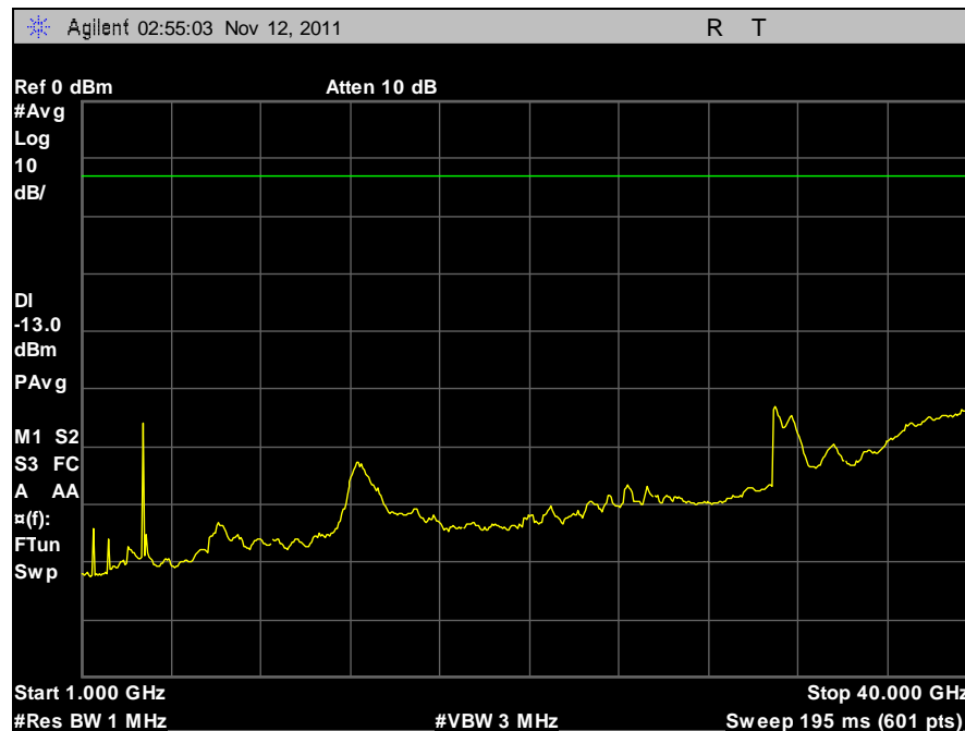
Plot 55. Conducted Spurious Emissions, 10 MHz, High Channel, Horizontal, 1 GHz – 40 GHz
