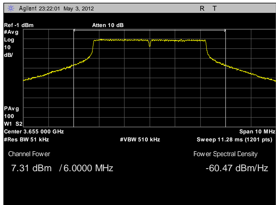
Plot 7. RF Channel Power, 5 MHz, Low Channel, Vertical
