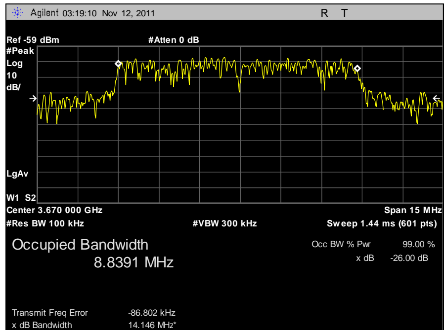
Plot 36. 99% Occupied Bandwidth, 10 MHz, High Channel, Horizontal
