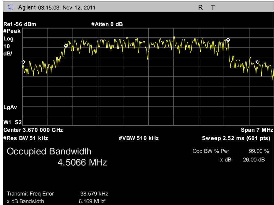
Plot 32. 99% Occupied Bandwidth, 5 MHz, High Channel, Horizontal
