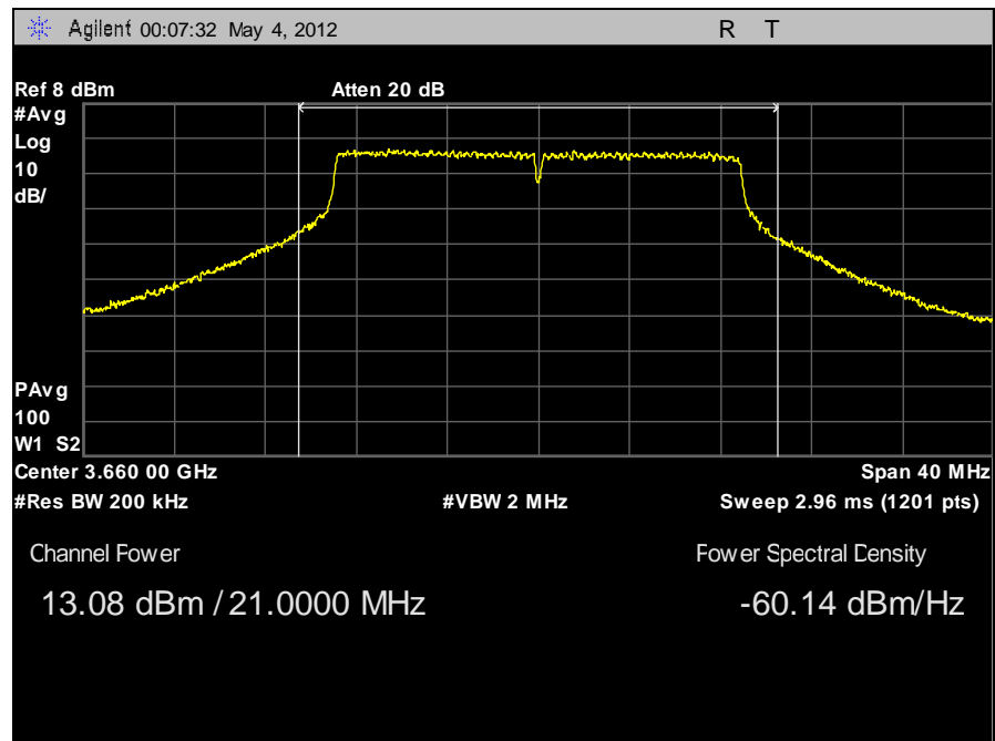
Plot 14. RF Channel Power, 20 MHz, Low Channel, Horizontal
