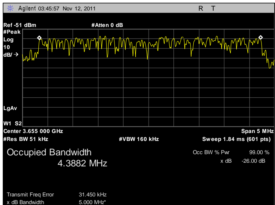
Plot 31. 99% Occupied Bandwidth, 5 MHz, Low Channel, Vertical
