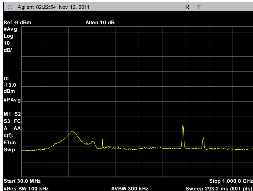
Plot 42. Conducted Spurious Emissions, 5 MHz, Low Channel, Horizontal, 30 MHz – 1 GHz
