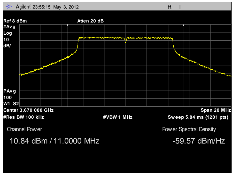
Plot 12. RF Channel Power, 10 MHz, High Channel, Horizontal
