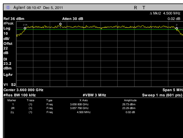
Plot 89. Frequency Stability, 3660 MHz, 120V, 20°C
