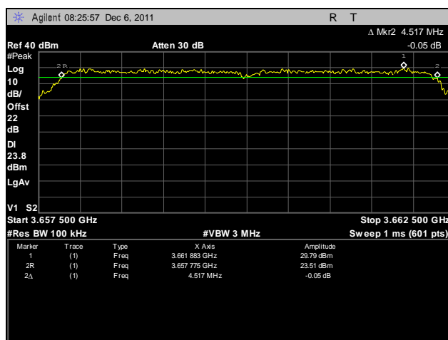
Plot 85. Frequency Stability, 3660 MHz, 120V, -10°C
