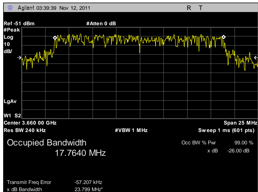
Plot 39. 99% Occupied Bandwidth, 20 MHz, Low Channel, Vertical
