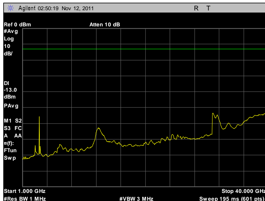
Plot 65. Conducted Spurious Emissions, 20 MHz, High Channel, Vertical, 1 GHz – 40 GHz
