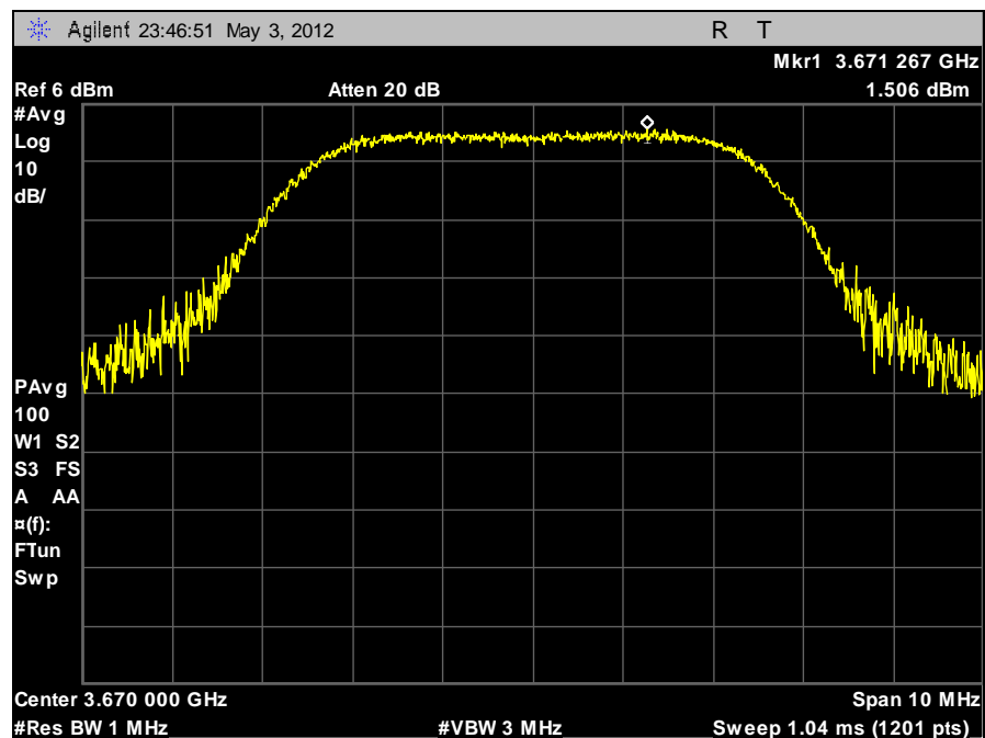
Plot 21. Peak Power Spectral Density, 5 MHz, High Channel, Vertical
