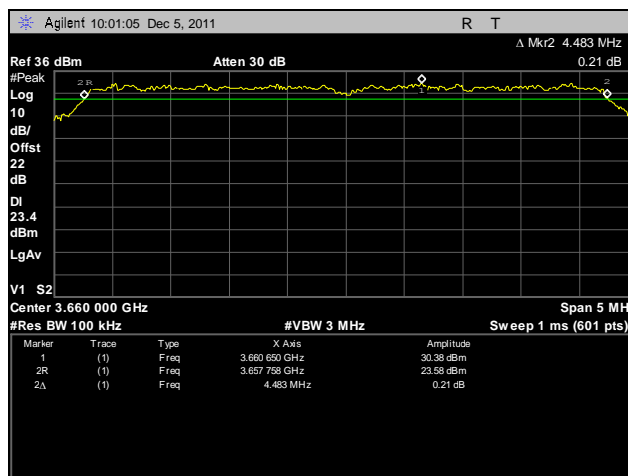
Plot 92. Frequency Stability, 3660 MHz, 120V, 40°C
