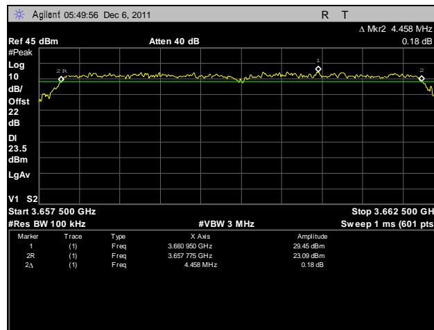
Plot 87. Frequency Stability, 3660 MHz, 120V, 10°C
