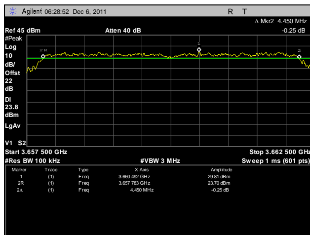
Plot 86. Frequency Stability, 3660 MHz, 120V, 0°C
