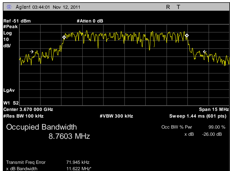
Plot 37. 99% Occupied Bandwidth, 10 MHz, High Channel, Vertical
