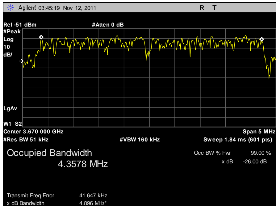
Plot 33. 99% Occupied Bandwidth, 5 MHz, High Channel, Vertical
