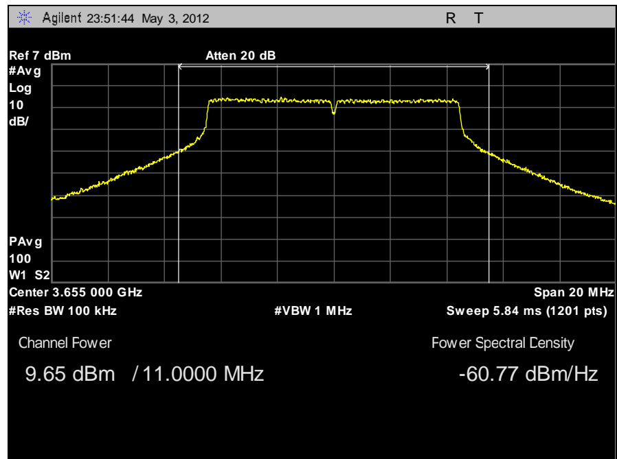
Plot 10. RF Channel Power, 10 MHz, Low Channel, Horizontal
