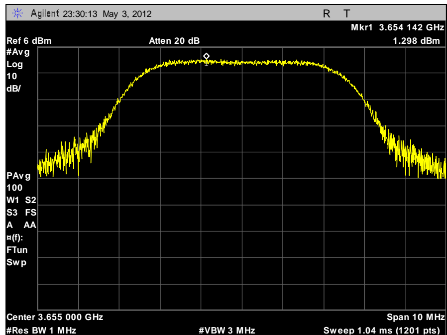
Plot 18. Peak Power Spectral Density, 5 MHz, Low Channel, Horizontal
