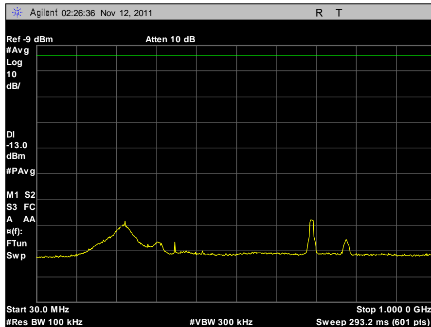
Plot 50. Conducted Spurious Emissions, 10 MHz, Low Channel, Horizontal, 30 MHz – 1 GHz
