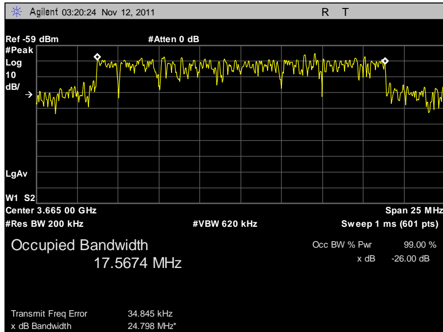
Plot 40. 99% Occupied Bandwidth, 20 MHz, High Channel, Horizontal
