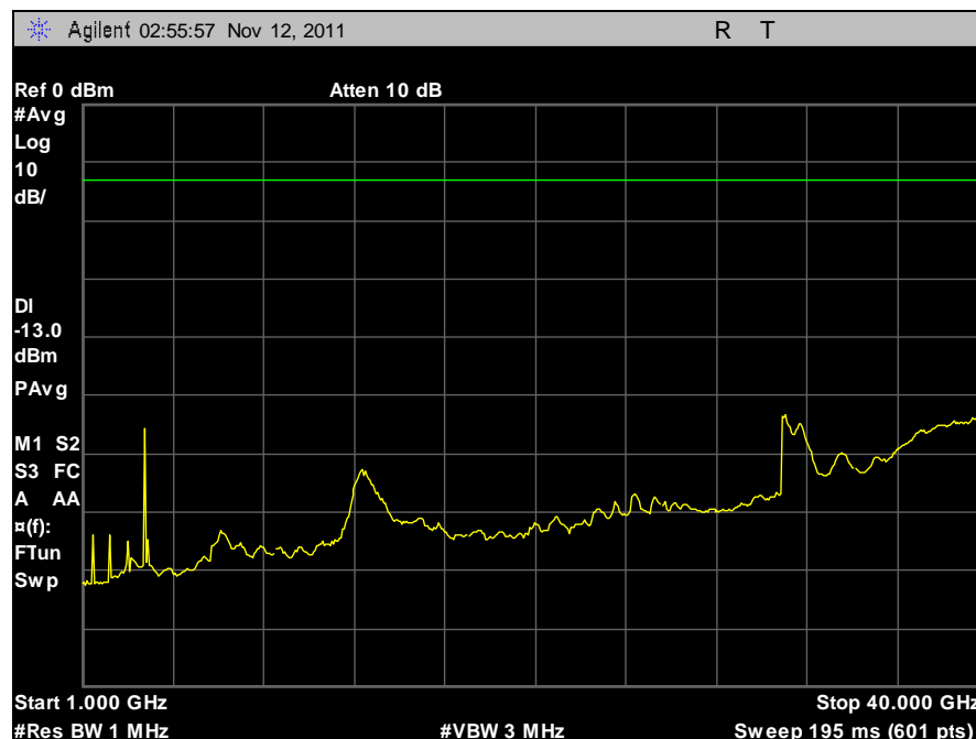
Plot 51. Conducted Spurious Emissions, 10 MHz, Low Channel, Horizontal, 1 GHz – 40 GHz
