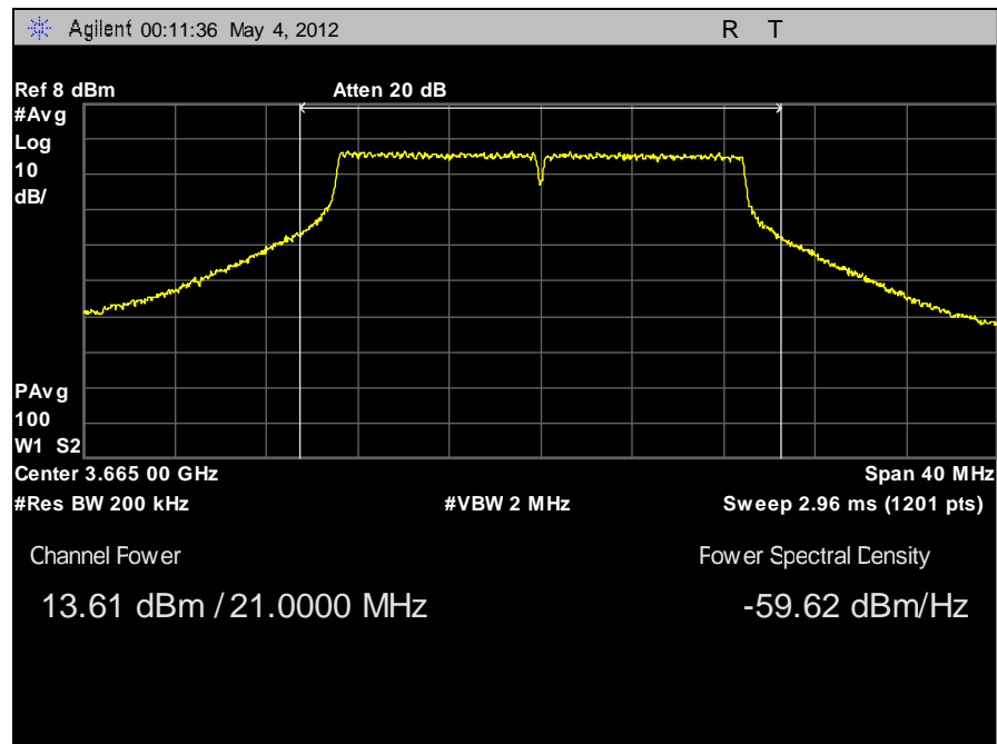
Plot 16. RF Channel Power, 20 MHz, High Channel, Horizontal
