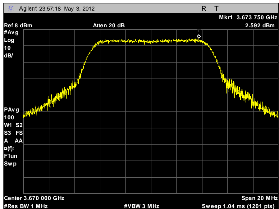
Plot 25. Peak Power Spectral Density, 10 MHz, High Channel, Vertical
