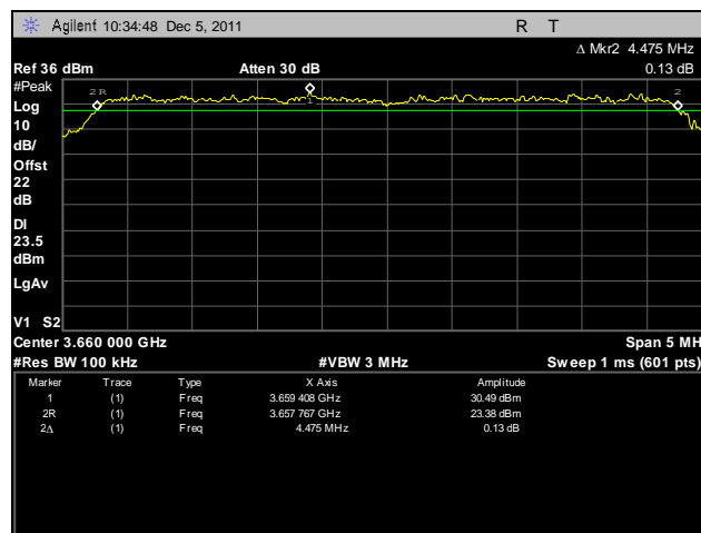
Plot 93. Frequency Stability, 3660 MHz, 120V, 50°C
