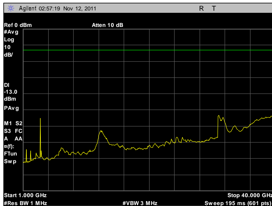
Plot 47. Conducted Spurious Emissions, 5 MHz, High Channel, Horizontal, 1 GHz – 40 GHz
