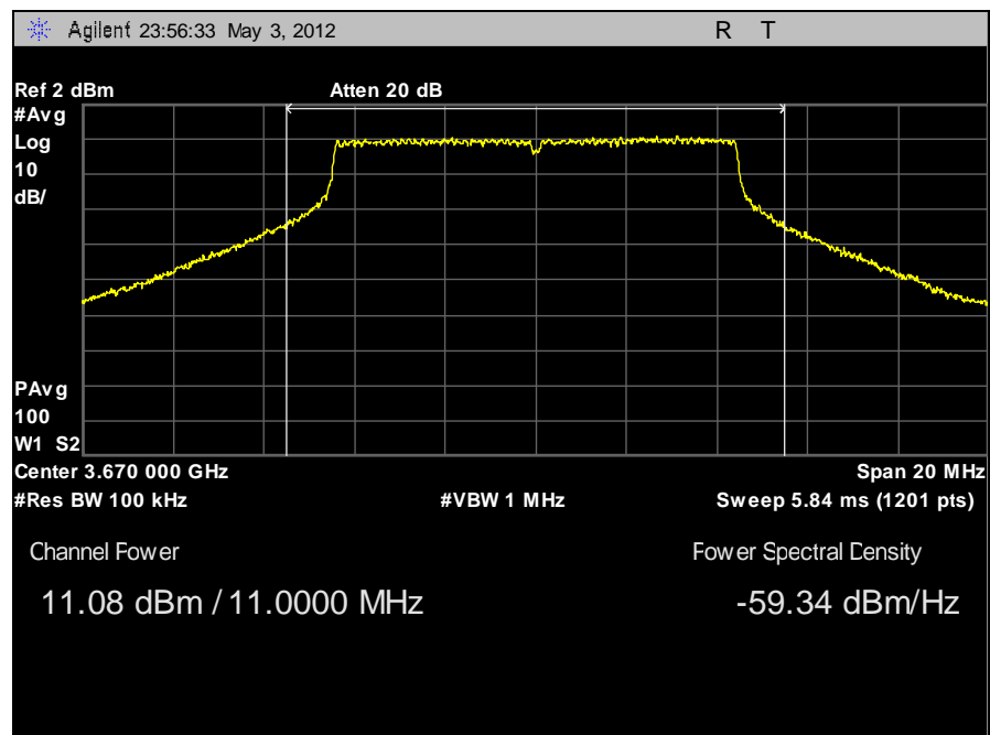
Plot 13. RF Channel Power, 10 MHz, High Channel, Vertical
