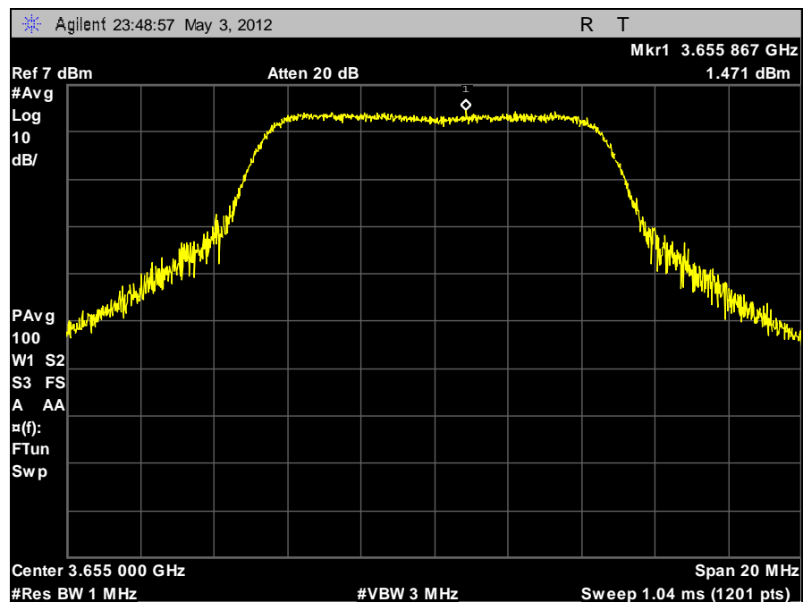
Plot 23. Peak Power Spectral Density, 10 MHz, Low Channel, Vertical
