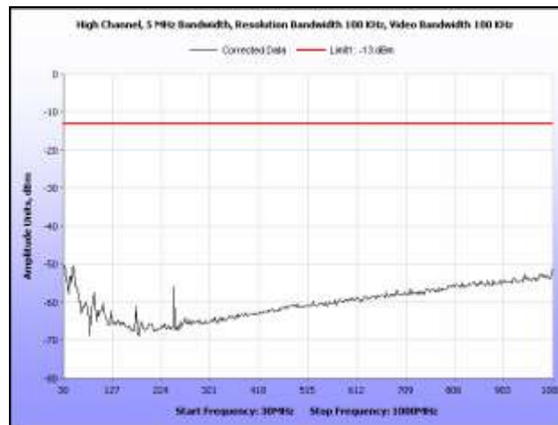
Plot 69. Radiated Spurious Emissions, 5 MHz, High Channel, 30 MHz – 1 GHz
