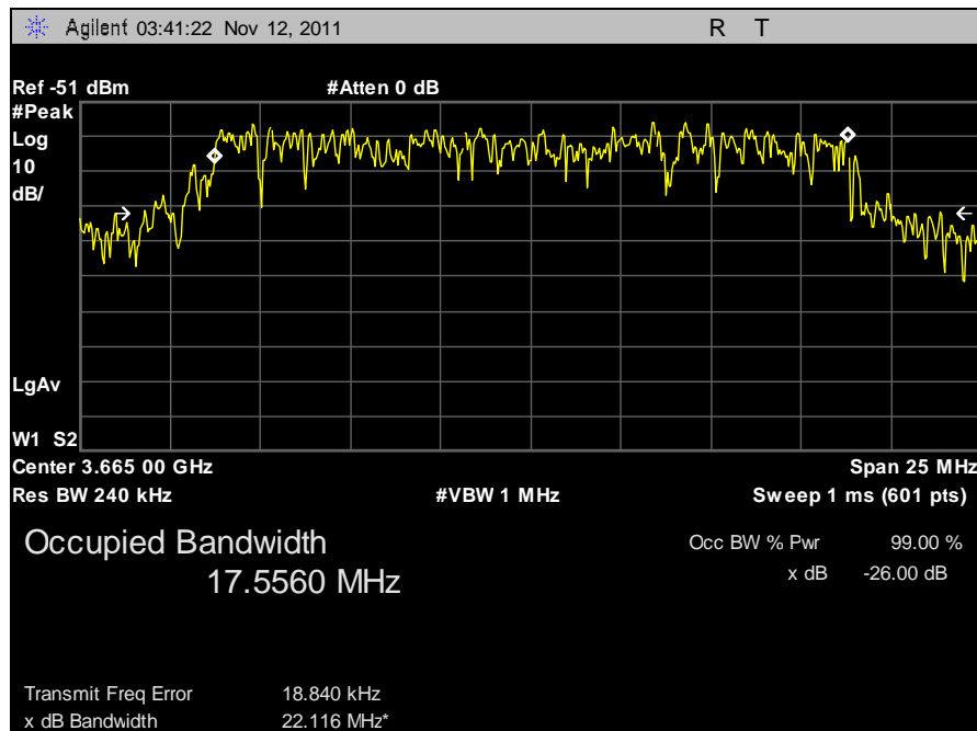
Plot 41. 99% Occupied Bandwidth, 20 MHz, High Channel, Vertical
