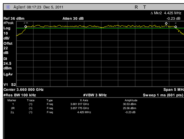
Plot 88. Frequency Stability, 3660 MHz, 102V, 20°C
