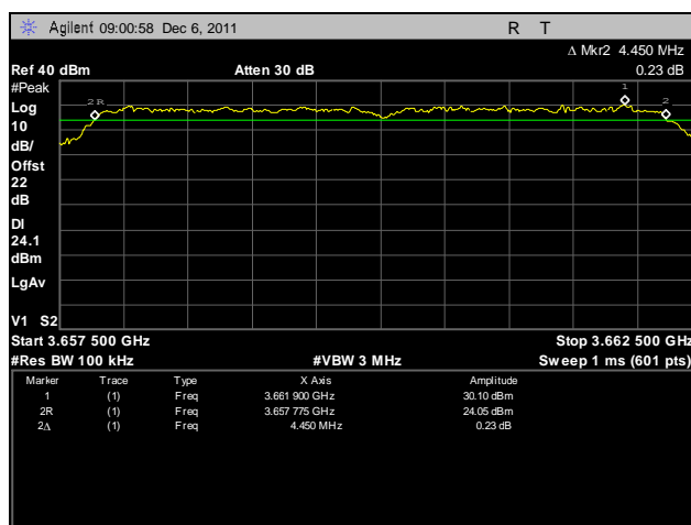
Plot 84. Frequency Stability, 3660 MHz, 120V, -20°C
