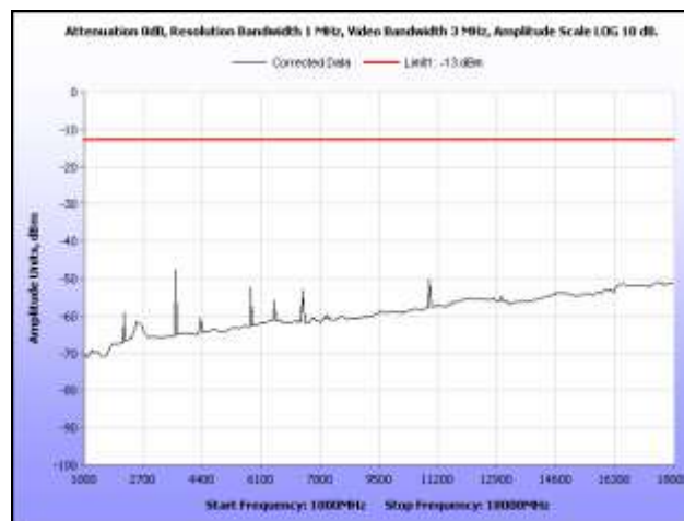
Plot 67. Radiated Spurious Emissions, 5 MHz, Low Channel, 1 GHz – 18 GHz
