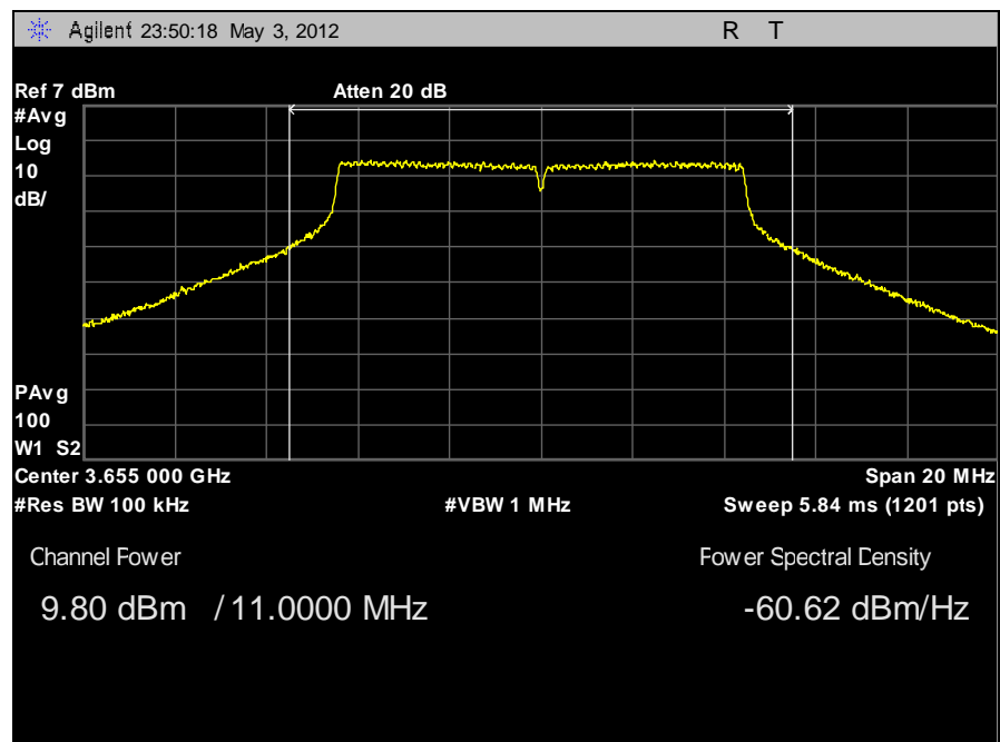
Plot 11. RF Channel Power, 10 MHz, Low Channel, Vertical
