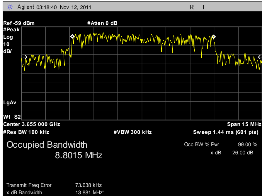
Plot 34. 99% Occupied Bandwidth, 10 MHz, Low Channel, Horizontal
