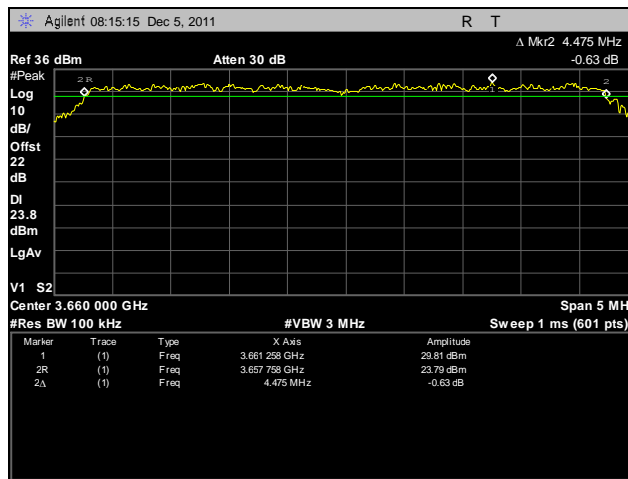
Plot 90. Frequency Stability, 3660 MHz, 138V, 20°C
