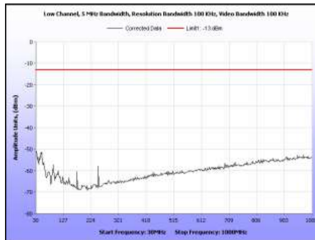
Plot 66. Radiated Spurious Emissions, 5 MHz, Low Channel, 30 MHz – 1 GHz
