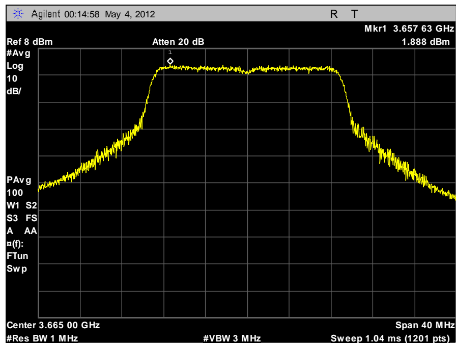
Plot 29. Peak Power Spectral Density, 20 MHz, High Channel, Vertical
