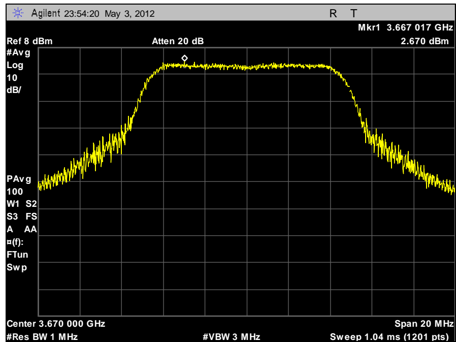
Plot 24. Peak Power Spectral Density, 10 MHz, High Channel, Horizontal
