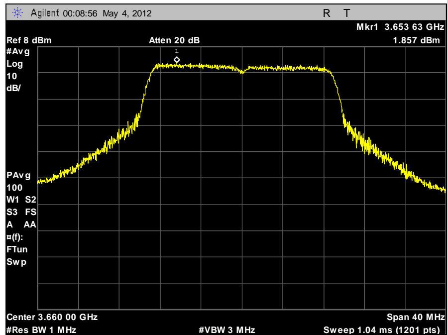
Plot 26. Peak Power Spectral Density, 20 MHz, Low Channel, Horizontal
