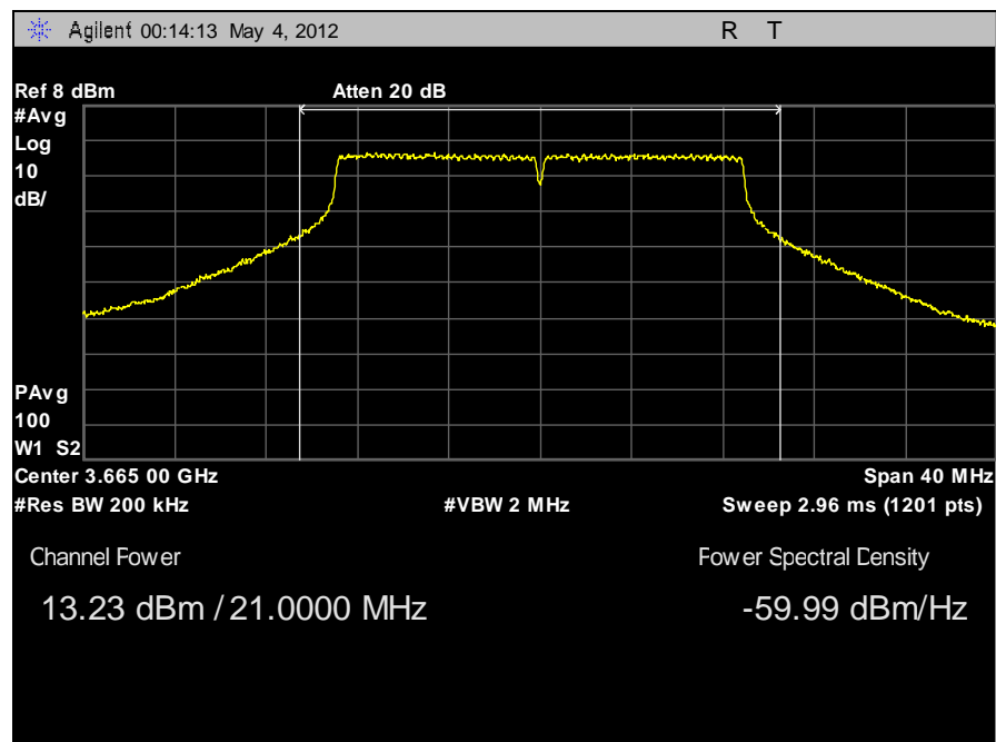
Plot 17. RF Channel Power, 20 MHz, High Channel, Vertical
