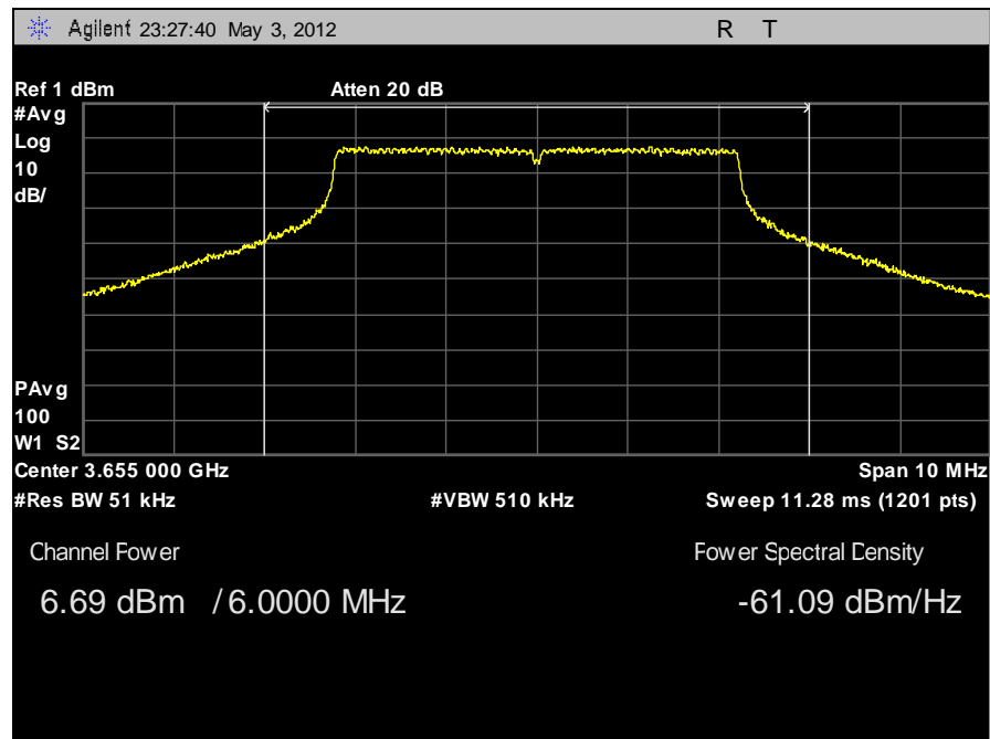
Plot 6. RF Channel Power, 5 MHz, Low Channel, Horizontal
