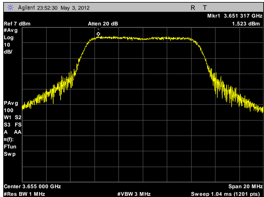
Plot 22. Peak Power Spectral Density, 10 MHz, Low Channel, Horizontal
