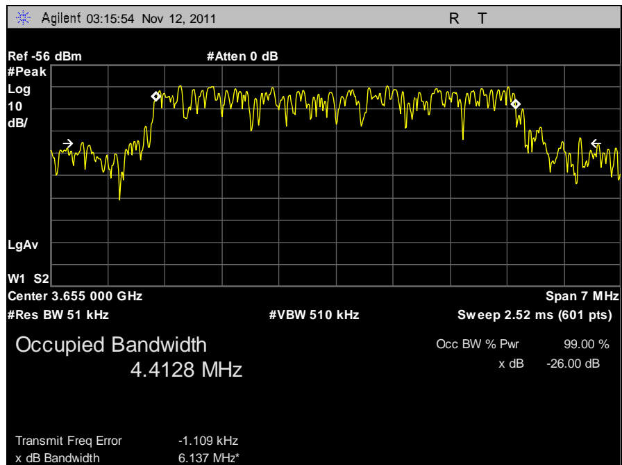
Plot 30. 99% Occupied Bandwidth, 5 MHz, Low Channel, Horizontal
