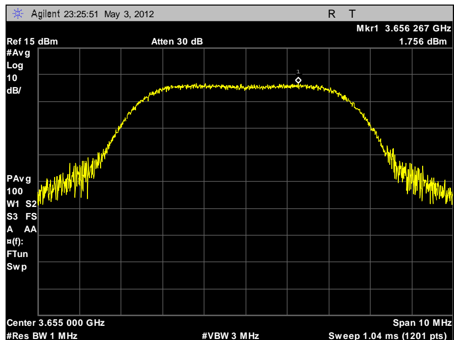
Plot 19. Peak Power Spectral Density, 5 MHz, Low Channel, Vertical
