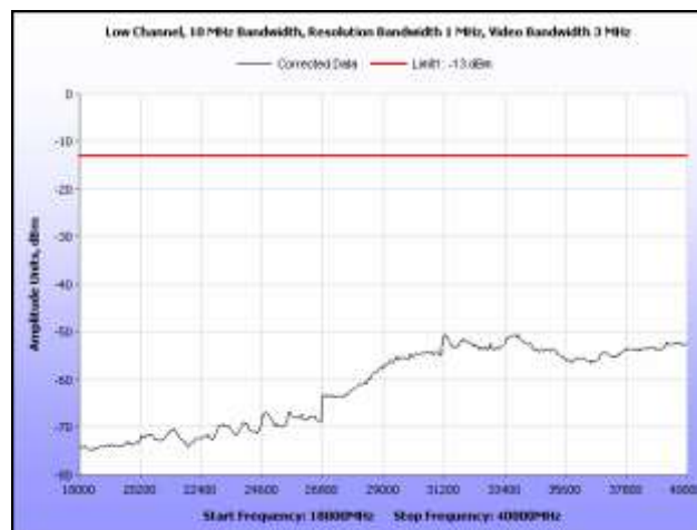
Plot 74. Radiated Spurious Emissions, 10 MHz, Low Channel, 18 GHz – 40 GHz
