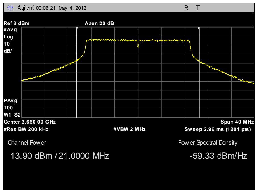
Plot 15. RF Channel Power, 20 MHz, Low Channel, Vertical
