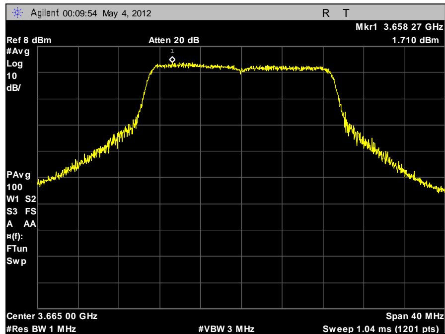
Plot 28. Peak Power Spectral Density, 20 MHz, High Channel, Horizontal
