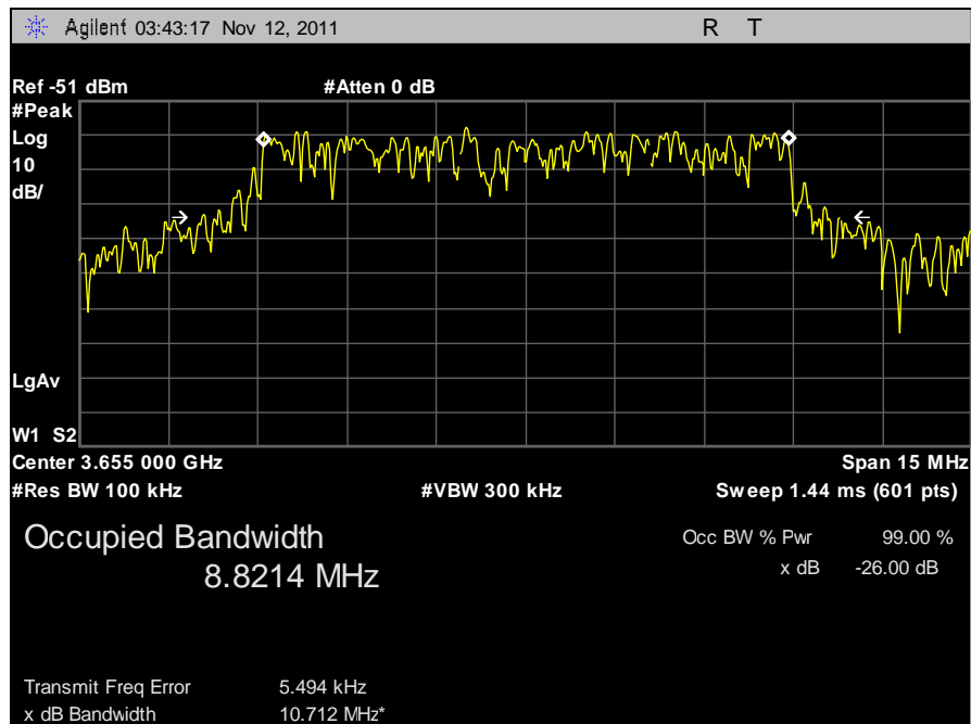
Plot 35. 99% Occupied Bandwidth, 10 MHz, Low Channel, Vertical
