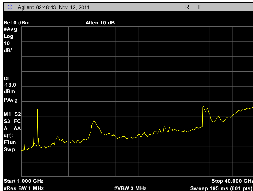
Plot 53. Conducted Spurious Emissions, 10 MHz, Low Channel, Vertical, 1 GHz – 40 GHz
