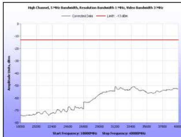
Plot 71. Radiated Spurious Emissions, 5 MHz, High Channel, 18 GHz – 40 GHz
