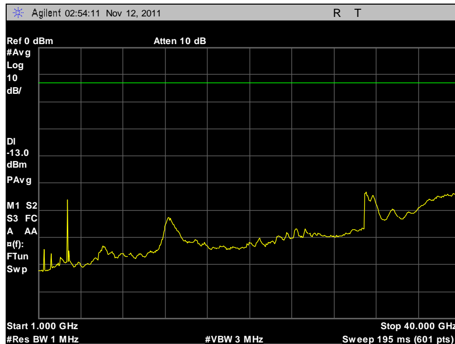
Plot 63. Conducted Spurious Emissions, 20 MHz, High Channel, Horizontal, 1 GHz – 40 GHz
