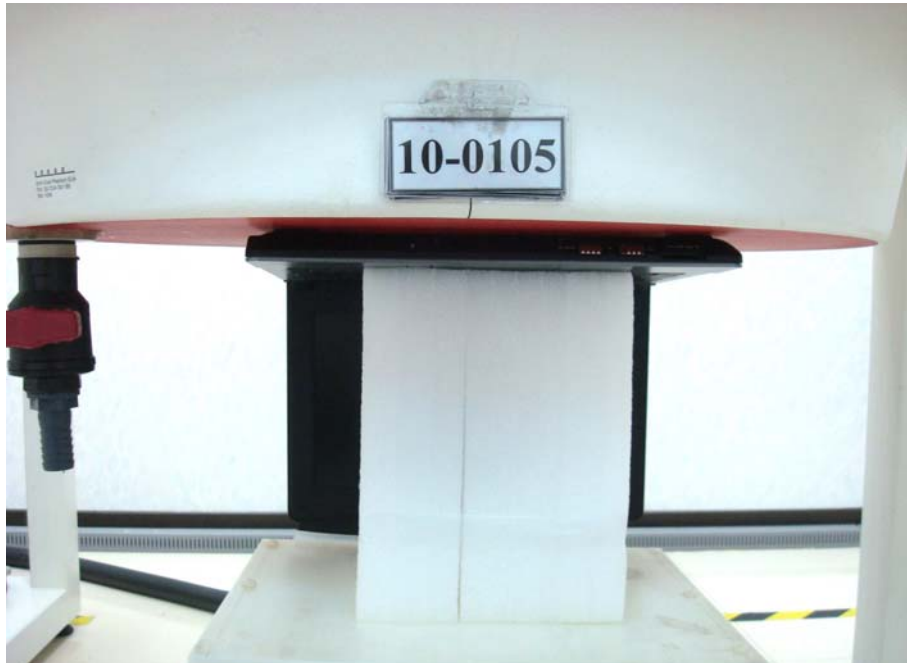
Figure 1. Body SAR Test Setup (Flat Section) Host: LCD Open 90° Bottom Close Body
