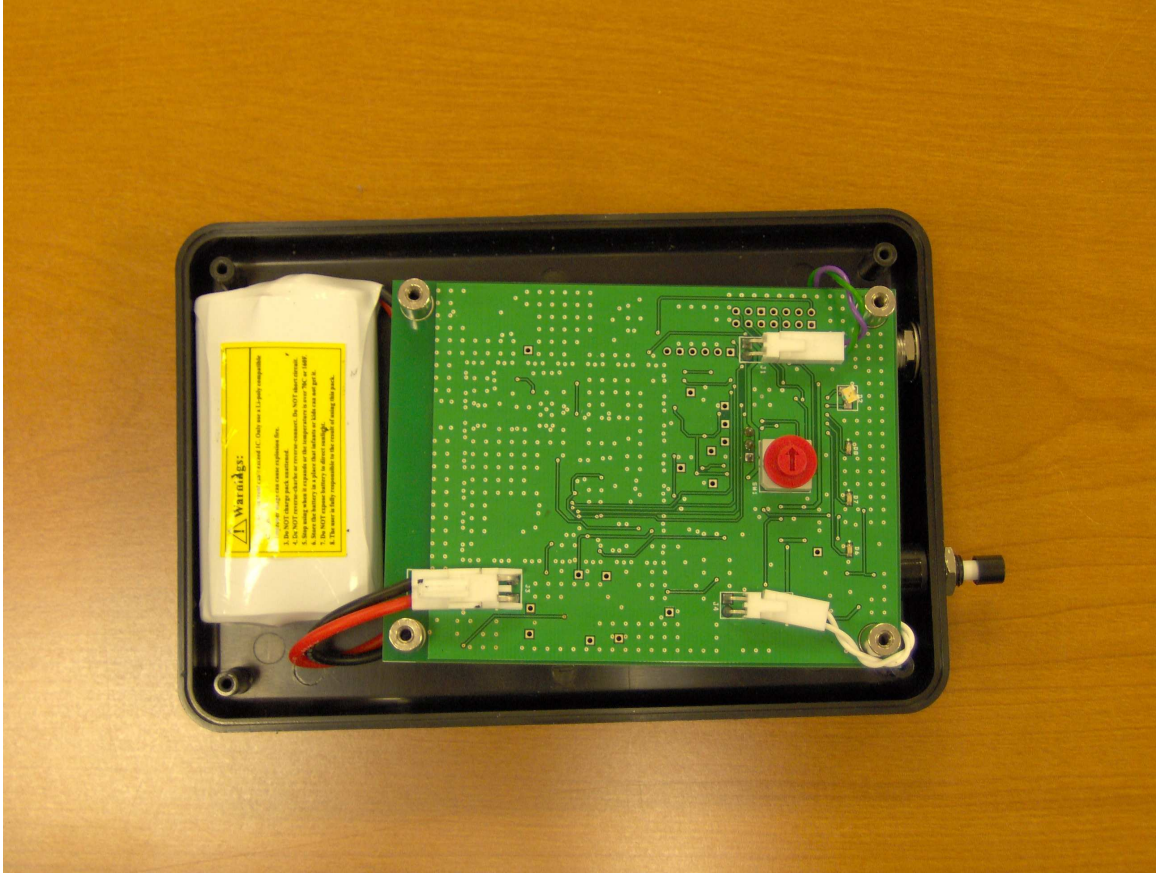
Interior Picture – Back Side of Board
