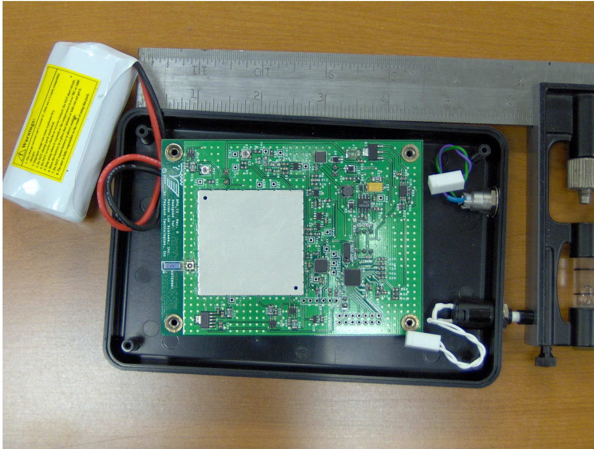
Interior Picture – Component Side of Board
