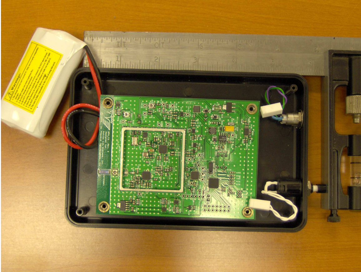
Interior Picture – Component Side with Shield Removed
