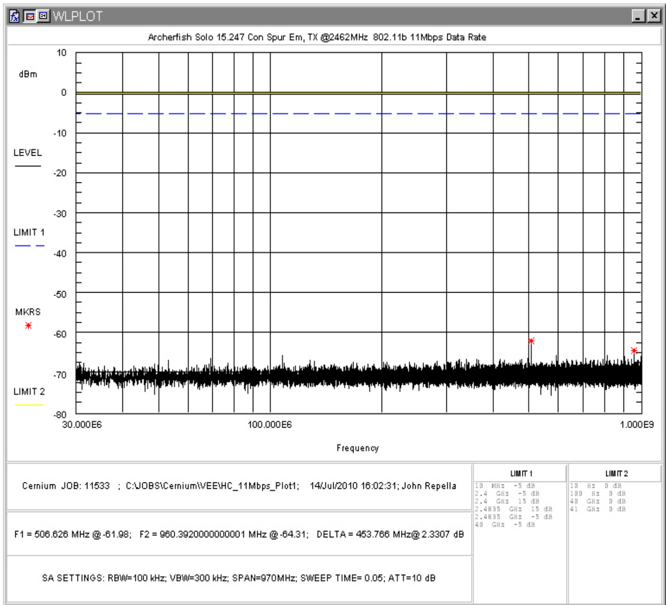
Figure 65: Conducted Spurious Emissions, 802.11b 11Mbps, High Channel 30 - 1000MHz
