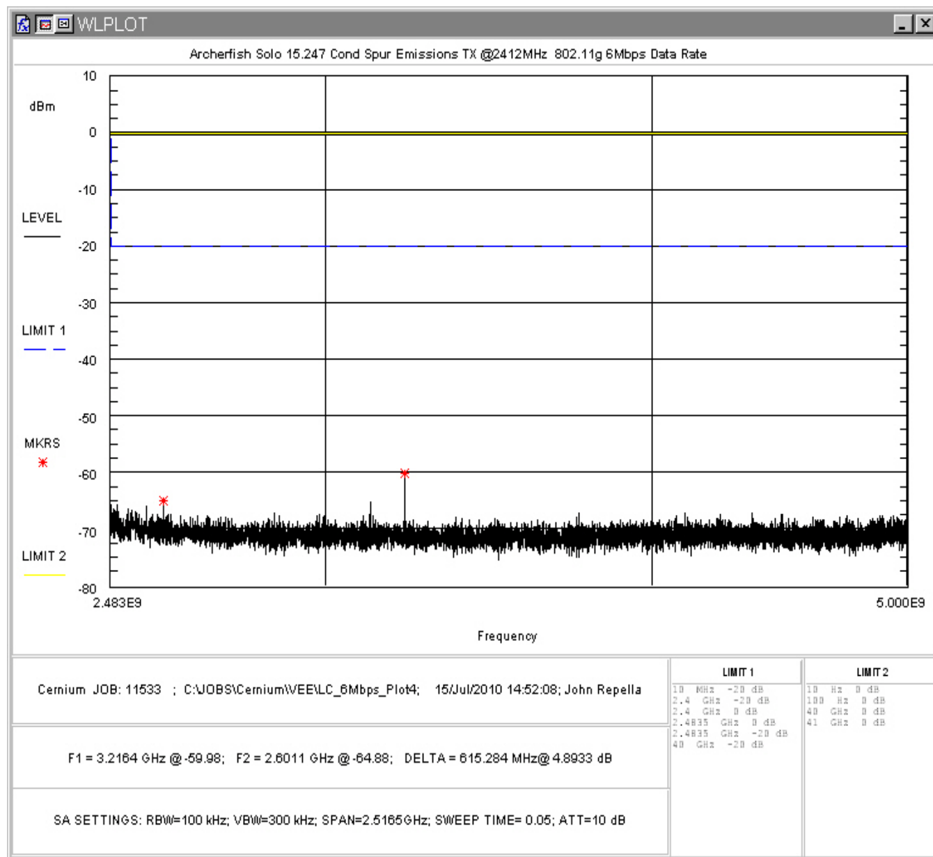
Figure 76: Conducted Spurious Emissions, 802.11g 6Mbps Low Channel, 2.483 - 5GHz
