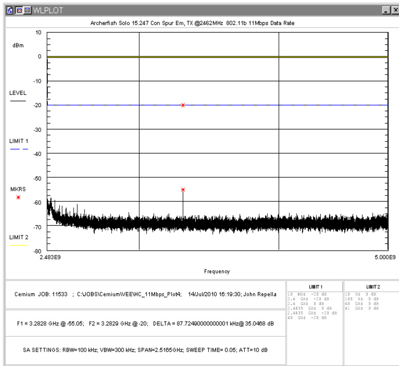
Figure 68: Conducted Spurious Emissions, 802.11b 11Mbps, High Channel 2.483 - 5GHz
