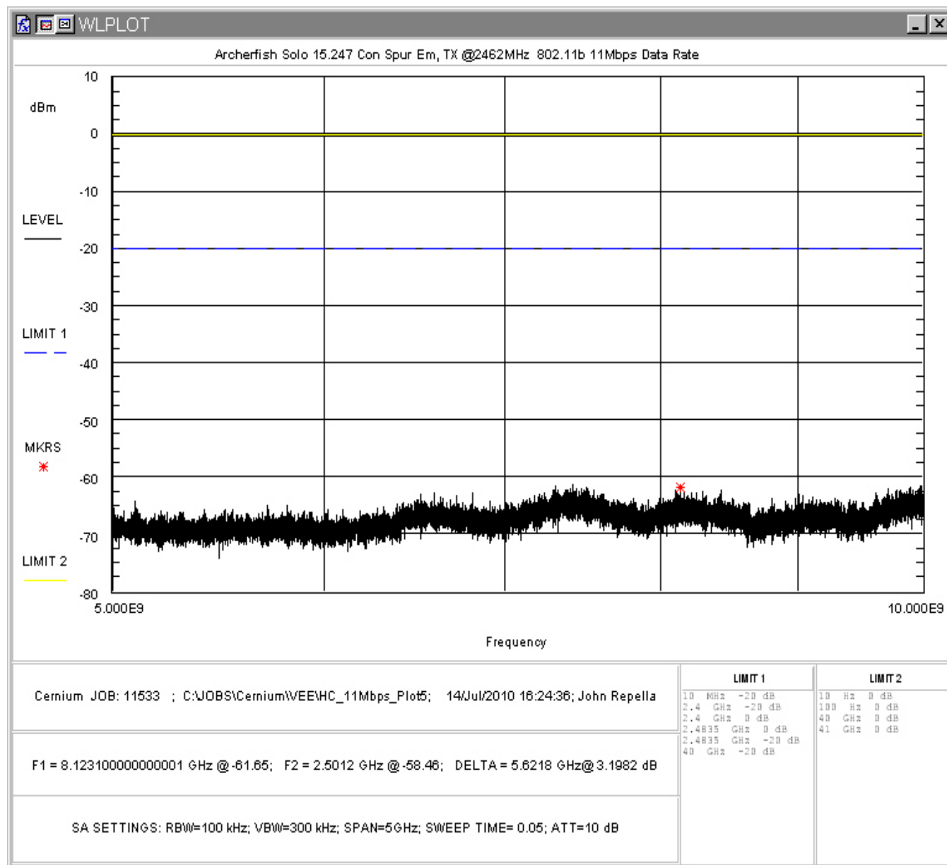
Figure 69: Conducted Spurious Emissions, 802.11b 11Mbps, High Channel 5 - 10GHz
