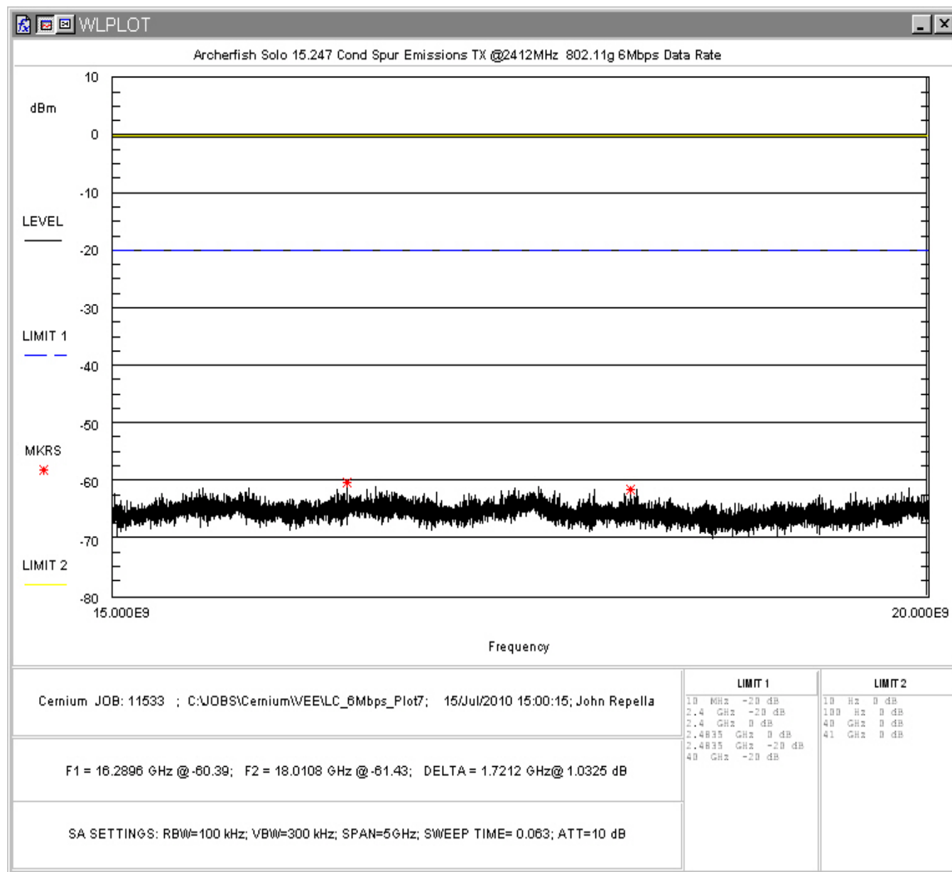
Figure 79: Conducted Spurious Emissions, 802.11g 6Mbps Low Channel, 15 - 20GHz
