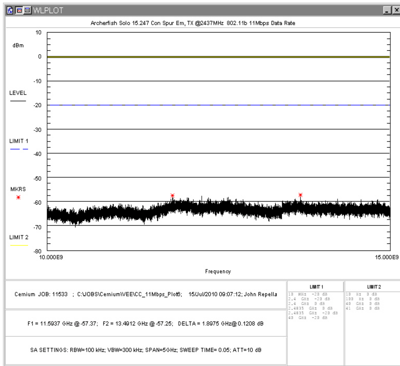
Figure 62: Conducted Spurious Emissions, 802.11b 11Mbps, Mid Channel 10 - 15GHz
