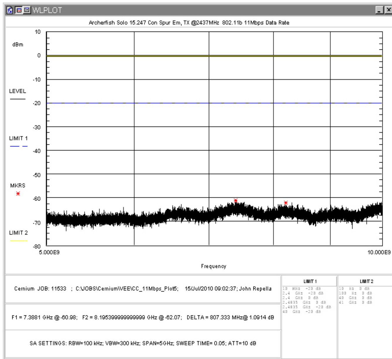
Figure 61: Conducted Spurious Emissions, 802.11b 11Mbps, Mid Channel 5 - 10GHz
