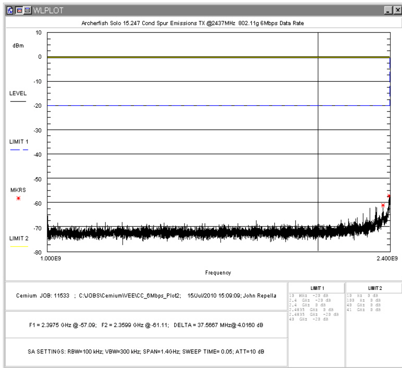
Figure 82: Conducted Spurious Emissions, 802.11g 6Mbps, Mid Channel 1 – 2.4GHz
