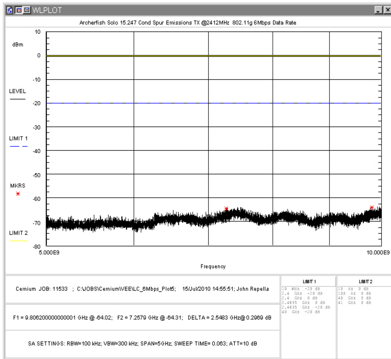
Figure 77: Conducted Spurious Emissions, 802.11g 6Mbps Low Channel, 5 - 10GHz
