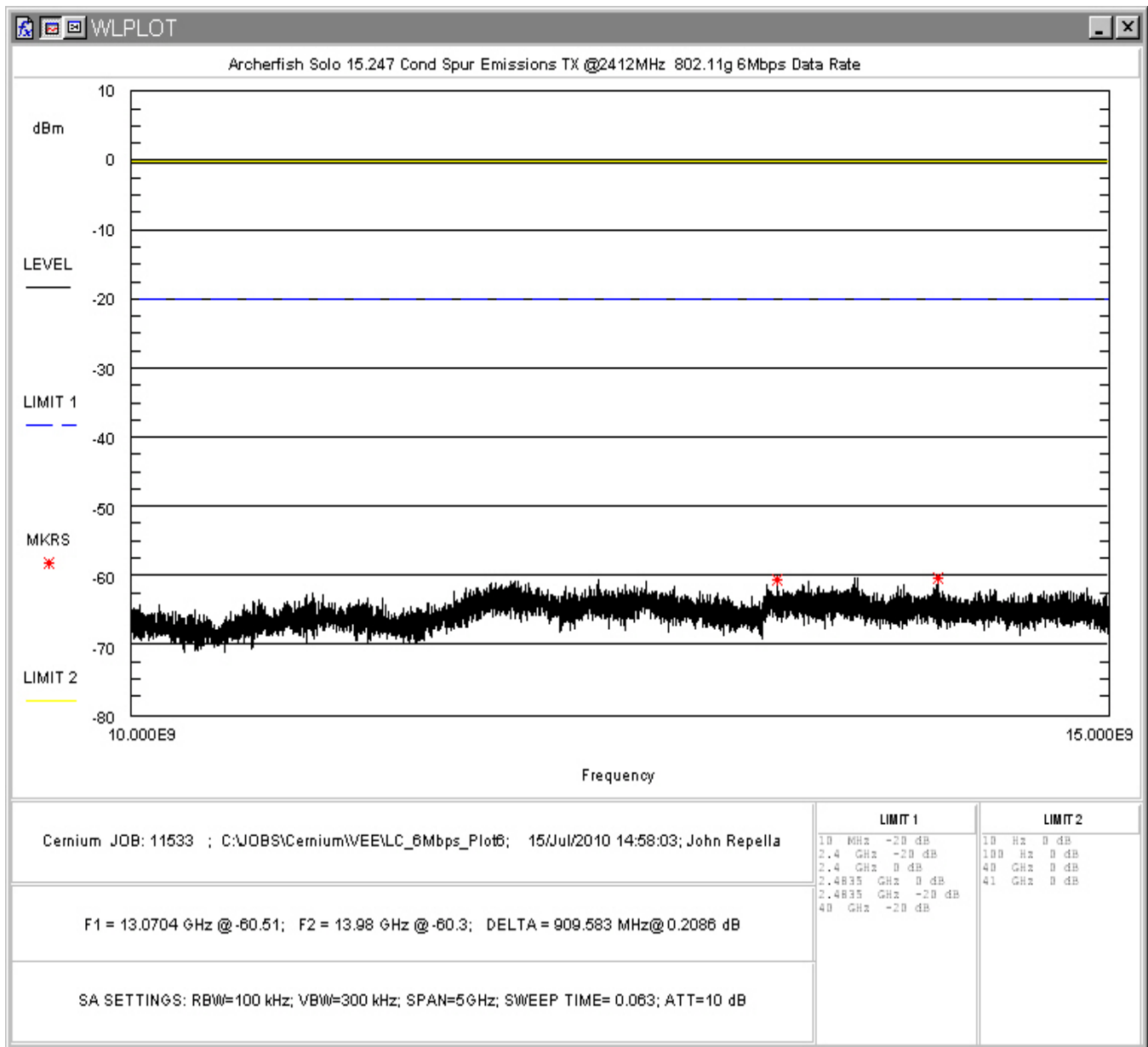
Figure 78: Conducted Spurious Emissions, 802.11g 6Mbps Low Channel, 10 - 15GHz
