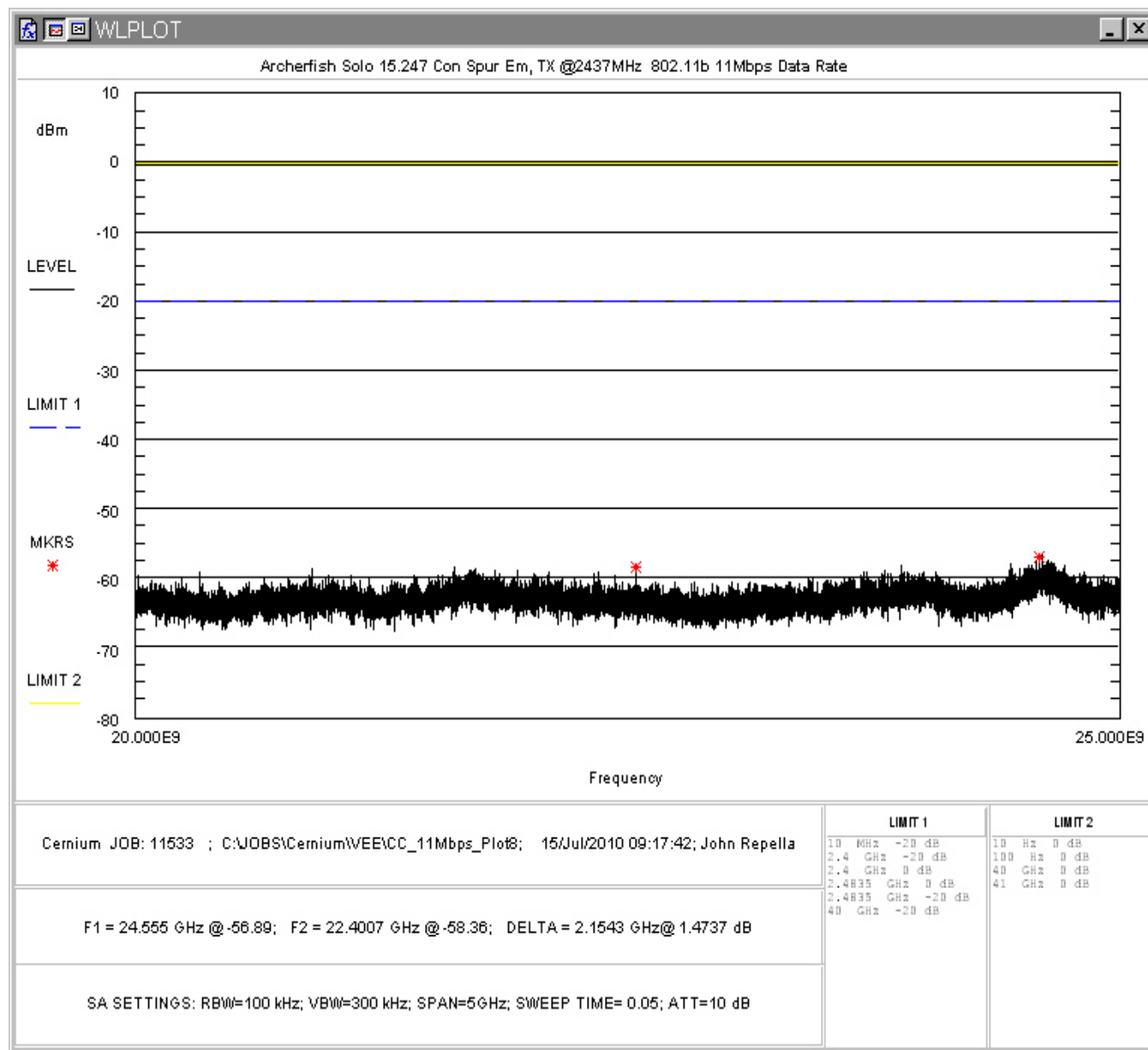
Figure 64: Conducted Spurious Emissions, 802.11b 11Mbps, Mid Channel 20 - 25GHz
