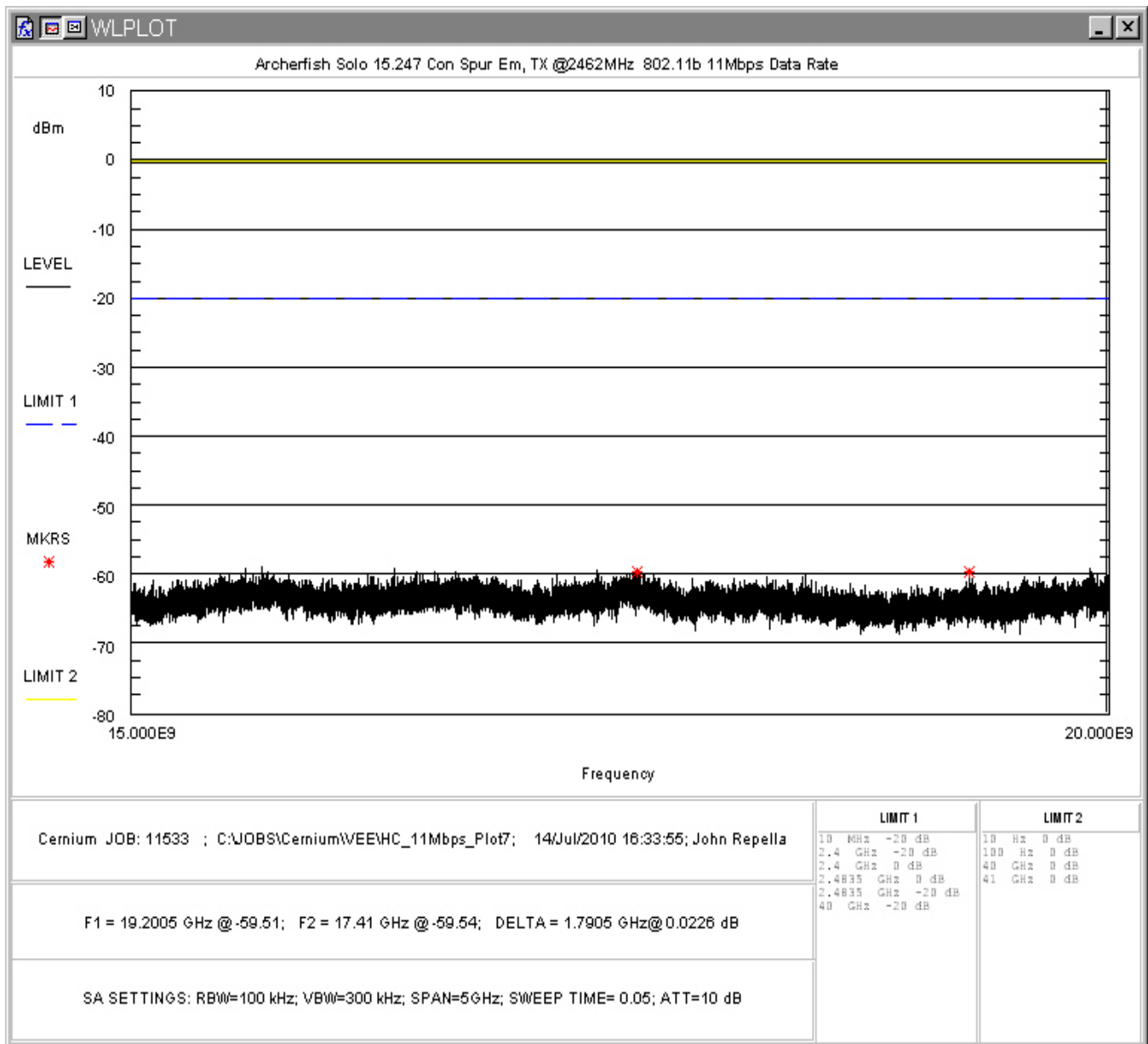
Figure 71: Conducted Spurious Emissions, 802.11b 11Mbps, High Channel 15 - 20GHz
