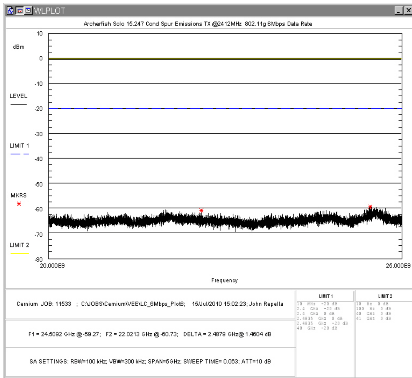
Figure 80: Conducted Spurious Emissions, 802.11g 6Mbps Low Channel, 20 - 25GHz
