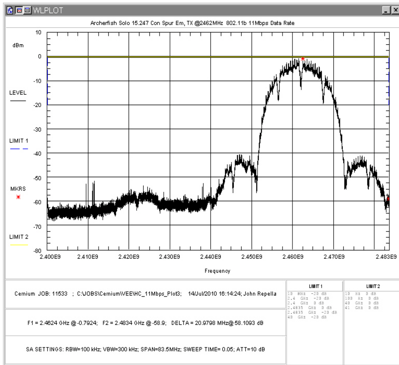
Figure 67: Conducted Spurious Emissions, 802.11b 11Mbps, High Channel 2.4 – 2.483GHz
