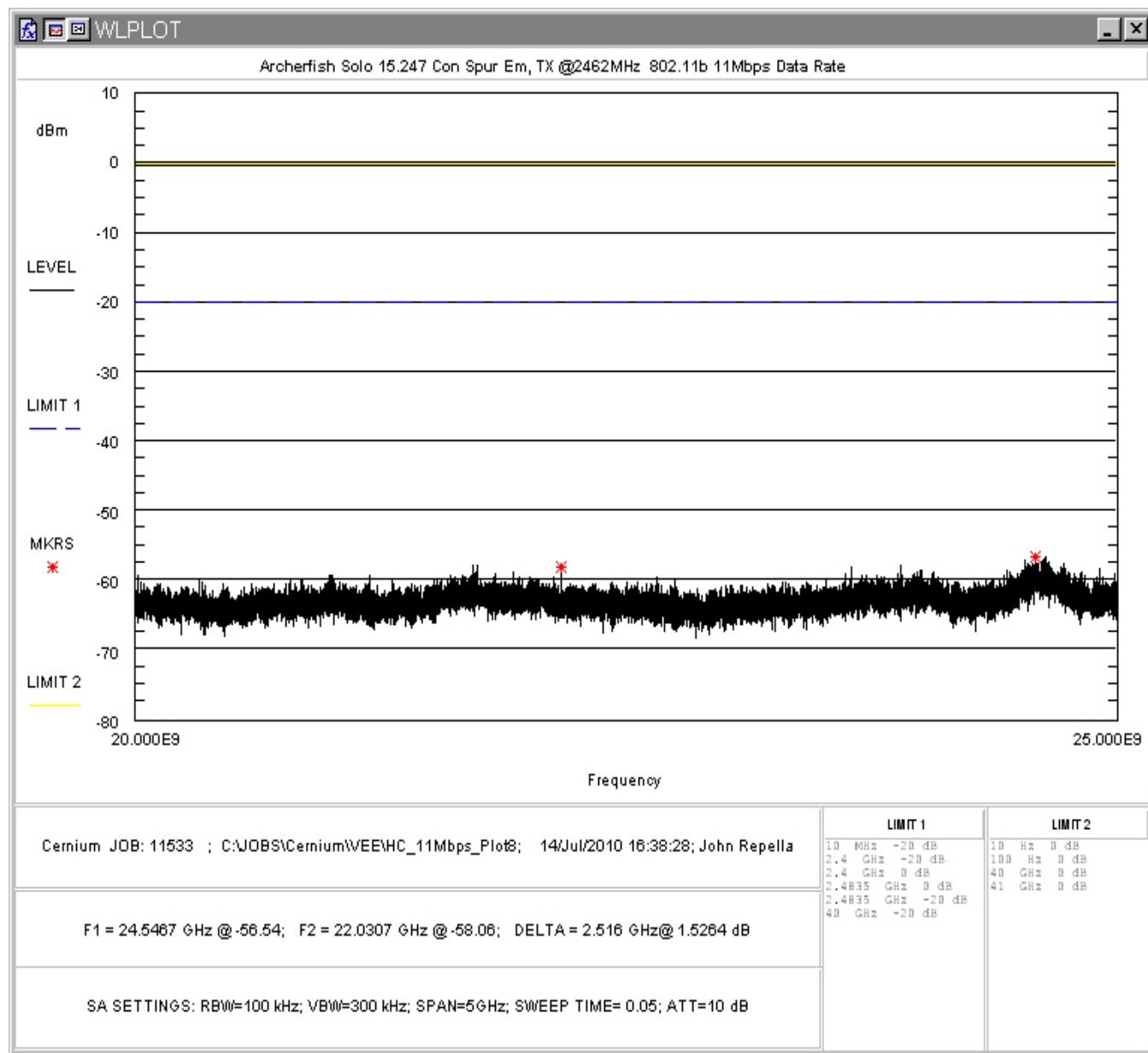
Figure 72: Conducted Spurious Emissions, 802.11b 11Mbps, High Channel 20 - 25GHz
