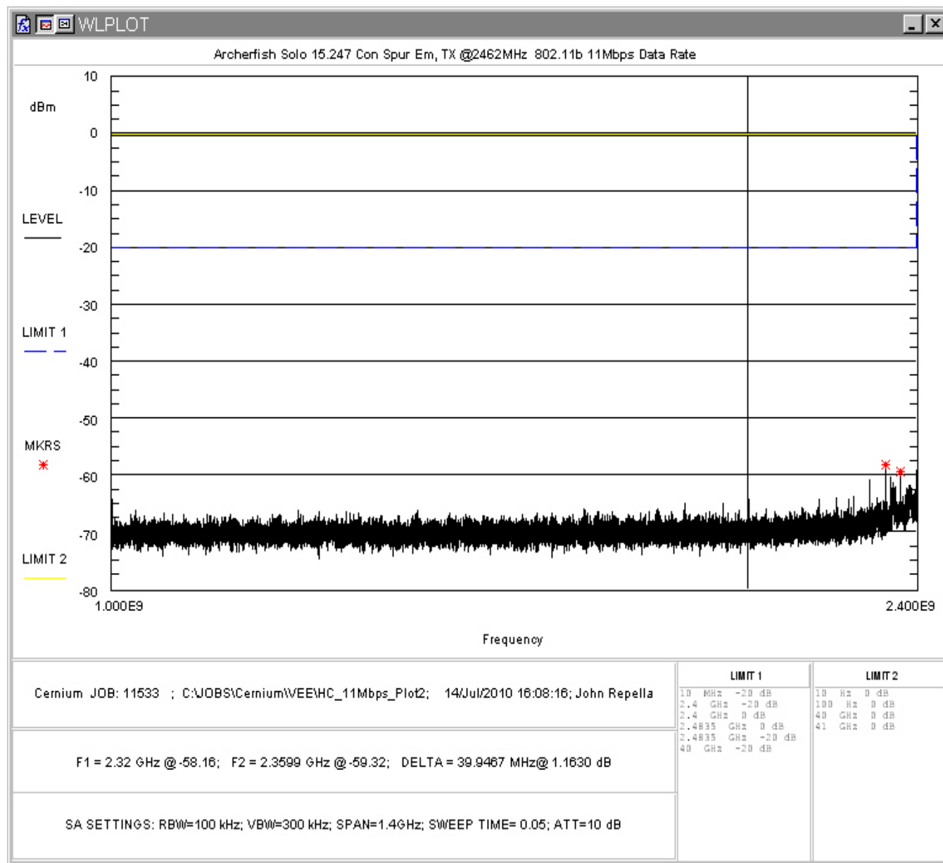
Figure 66: Conducted Spurious Emissions, 802.11b 11Mbps, High Channel 1 – 2.4GHz
