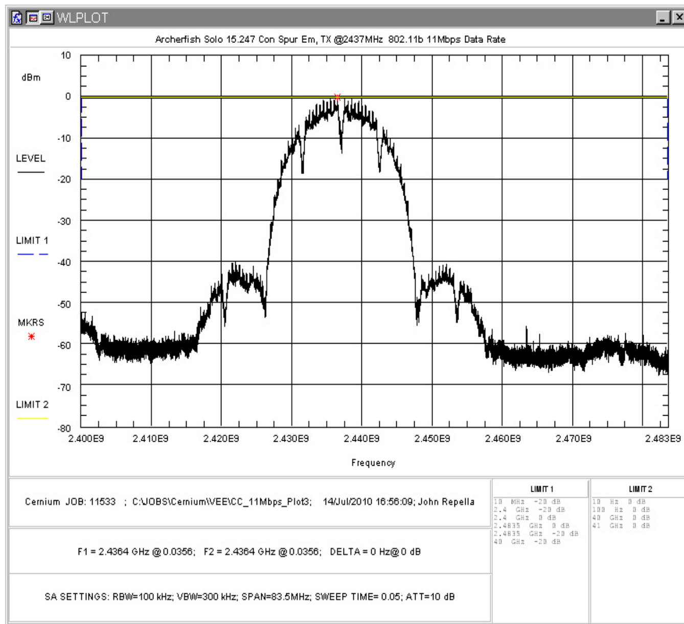
Figure 59: Conducted Spurious Emissions, 802.11b 11Mbps, Mid Channel 2.4 – 2.483GHz
