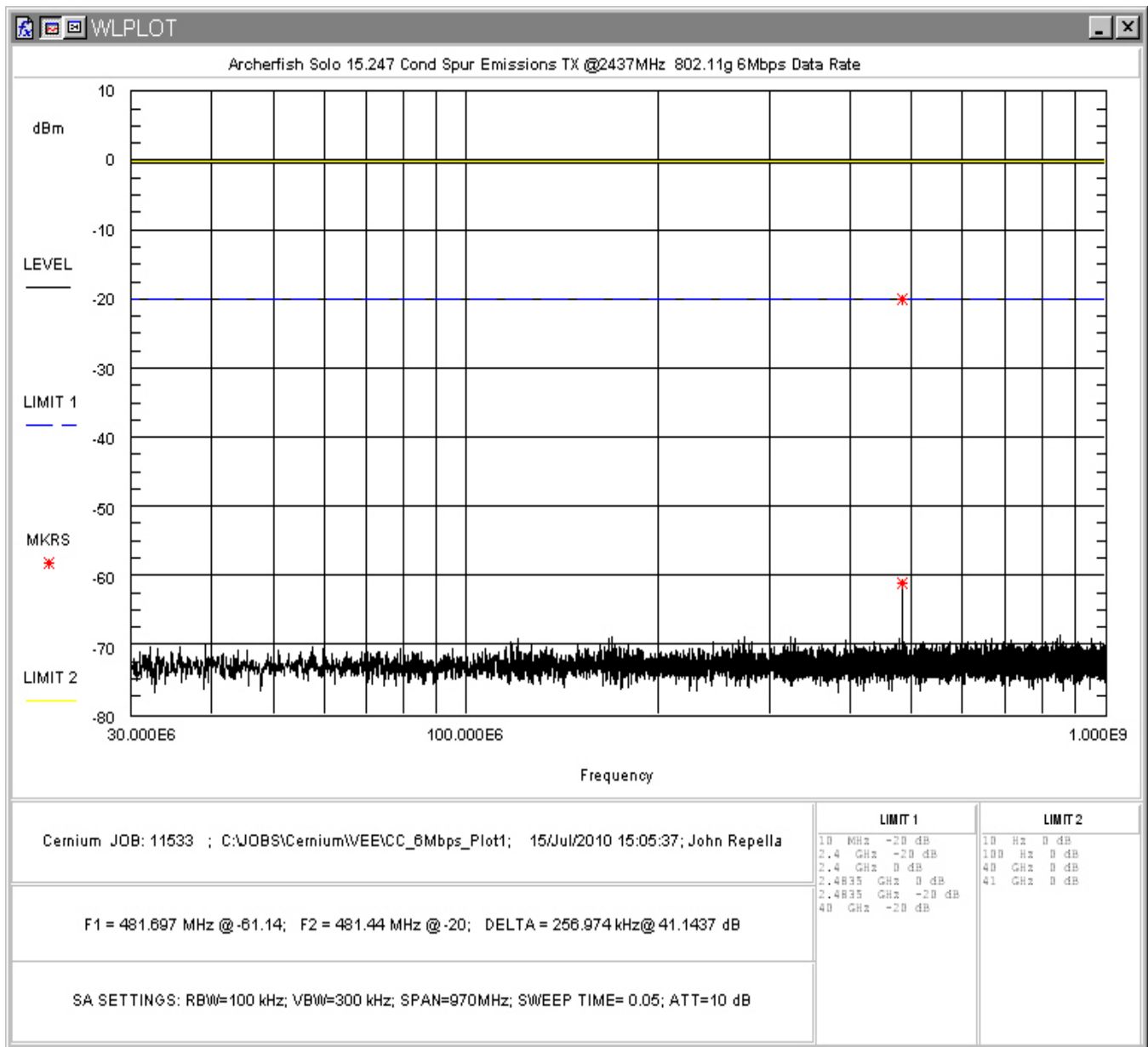
Figure 81: Conducted Spurious Emissions, 802.11g 6Mbps, Mid Channel 30 - 1000MHz
