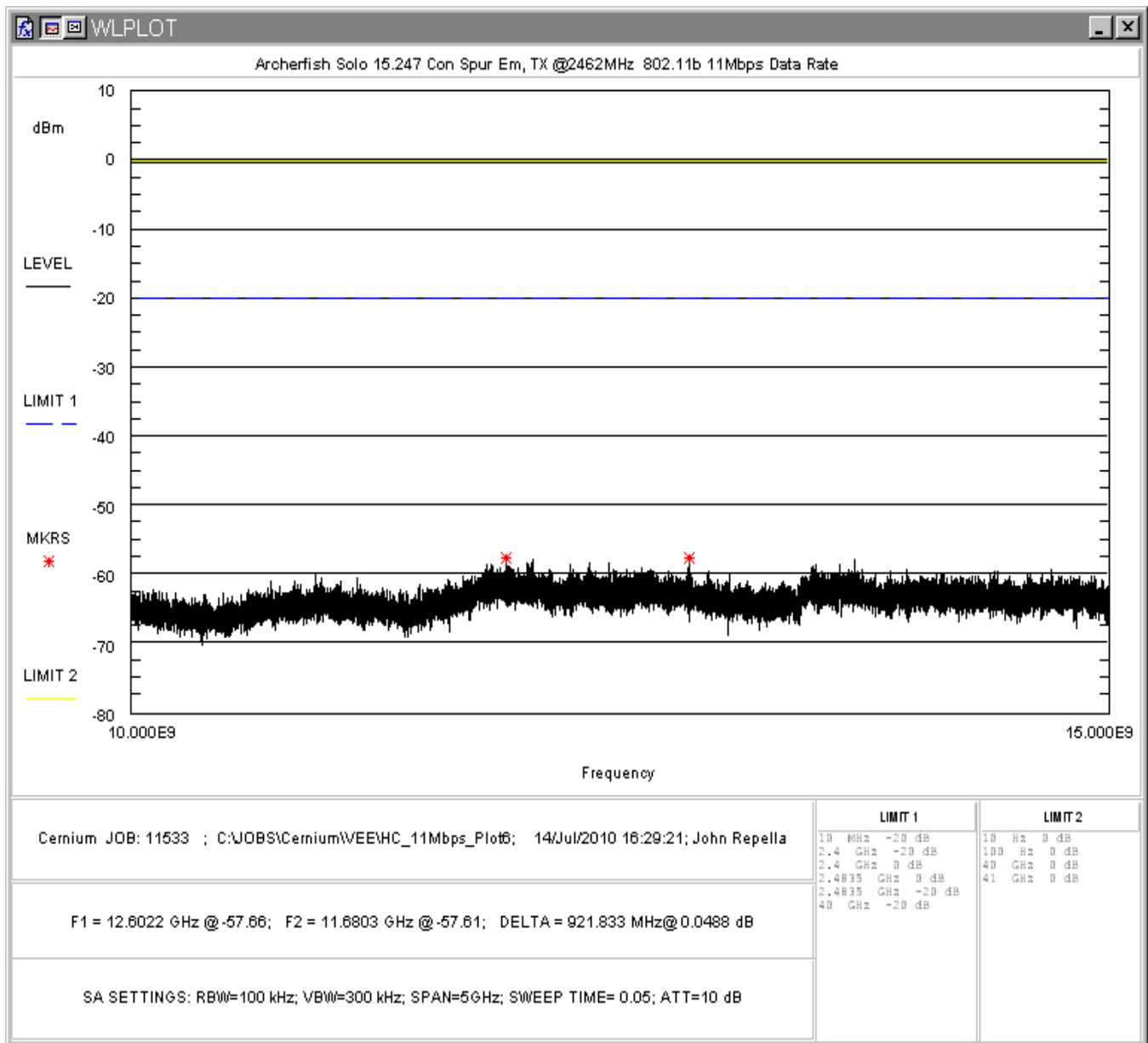
Figure 70: Conducted Spurious Emissions, 802.11b 11Mbps, High Channel 10 - 15GHz
