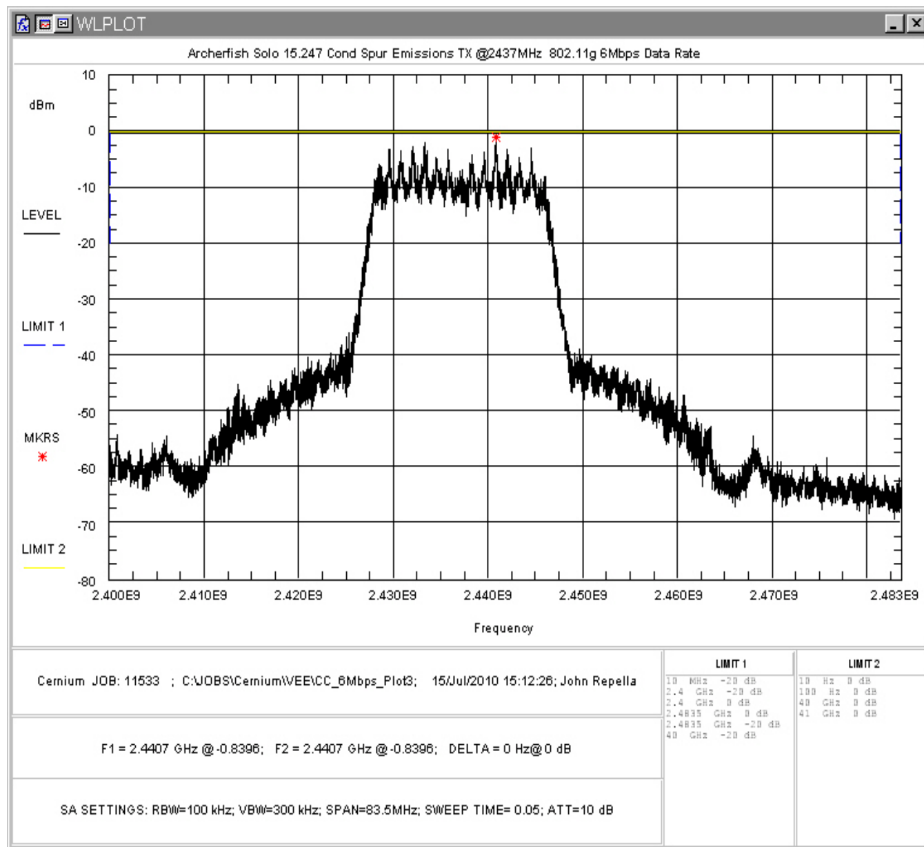
Figure 83: Conducted Spurious Emissions, 802.11g 6Mbps, Mid Channel 2.4 – 2.483GHz
