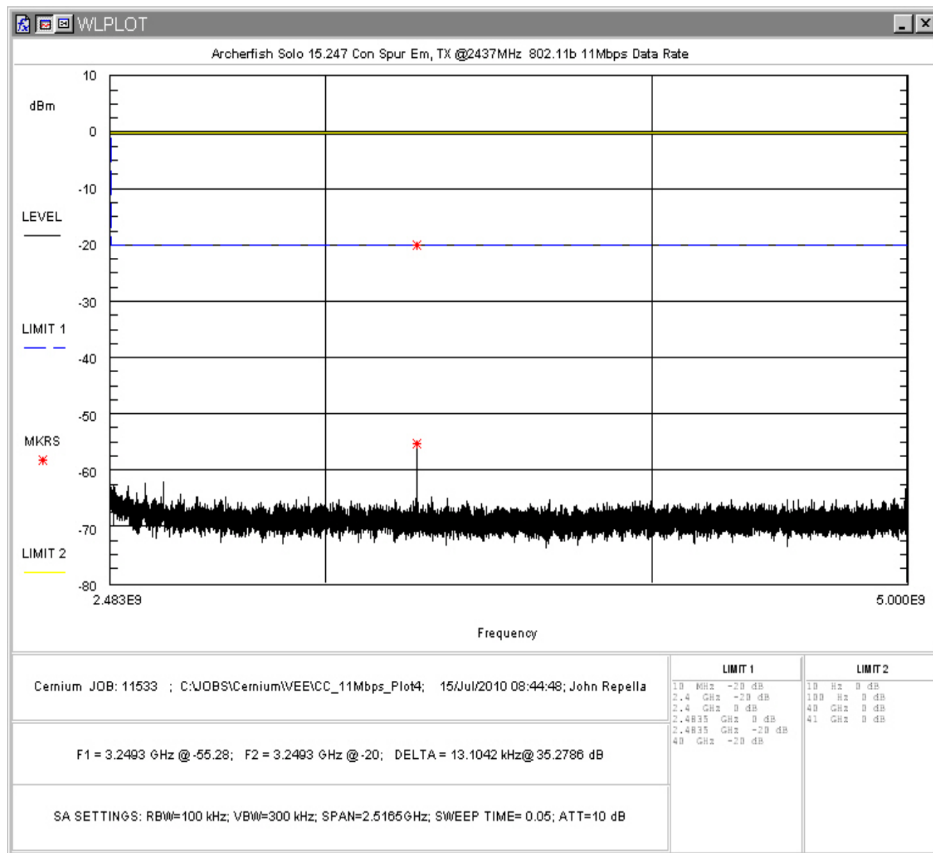
Figure 60: Conducted Spurious Emissions, 802.11b 11Mbps, Mid Channel 2.483 - 5GHz
