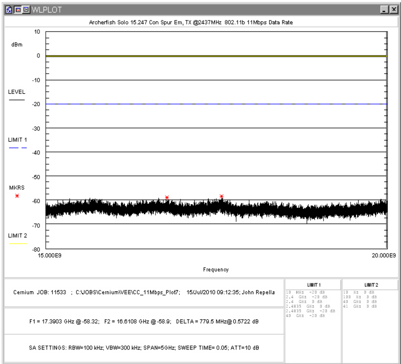
Figure 63: Conducted Spurious Emissions, 802.11b 11Mbps, Mid Channel 15 - 20GHz
