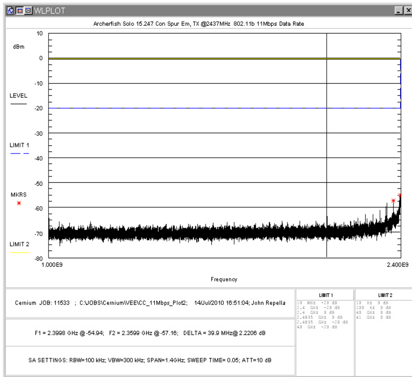
Figure 58: Conducted Spurious Emissions, 802.11b 11Mbps, Mid Channel 1 – 2.4GHz
