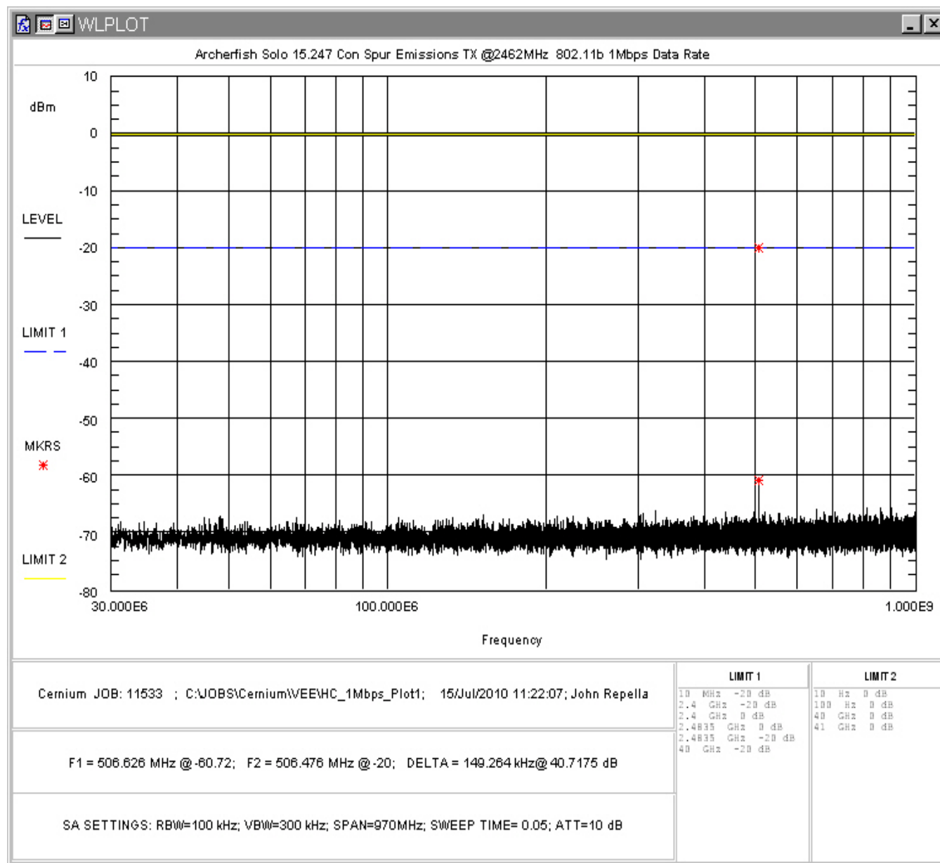
Figure 41: Conducted Spurious Emissions, 802.11b 1Mbps, High Channel 30 - 1000MHz
