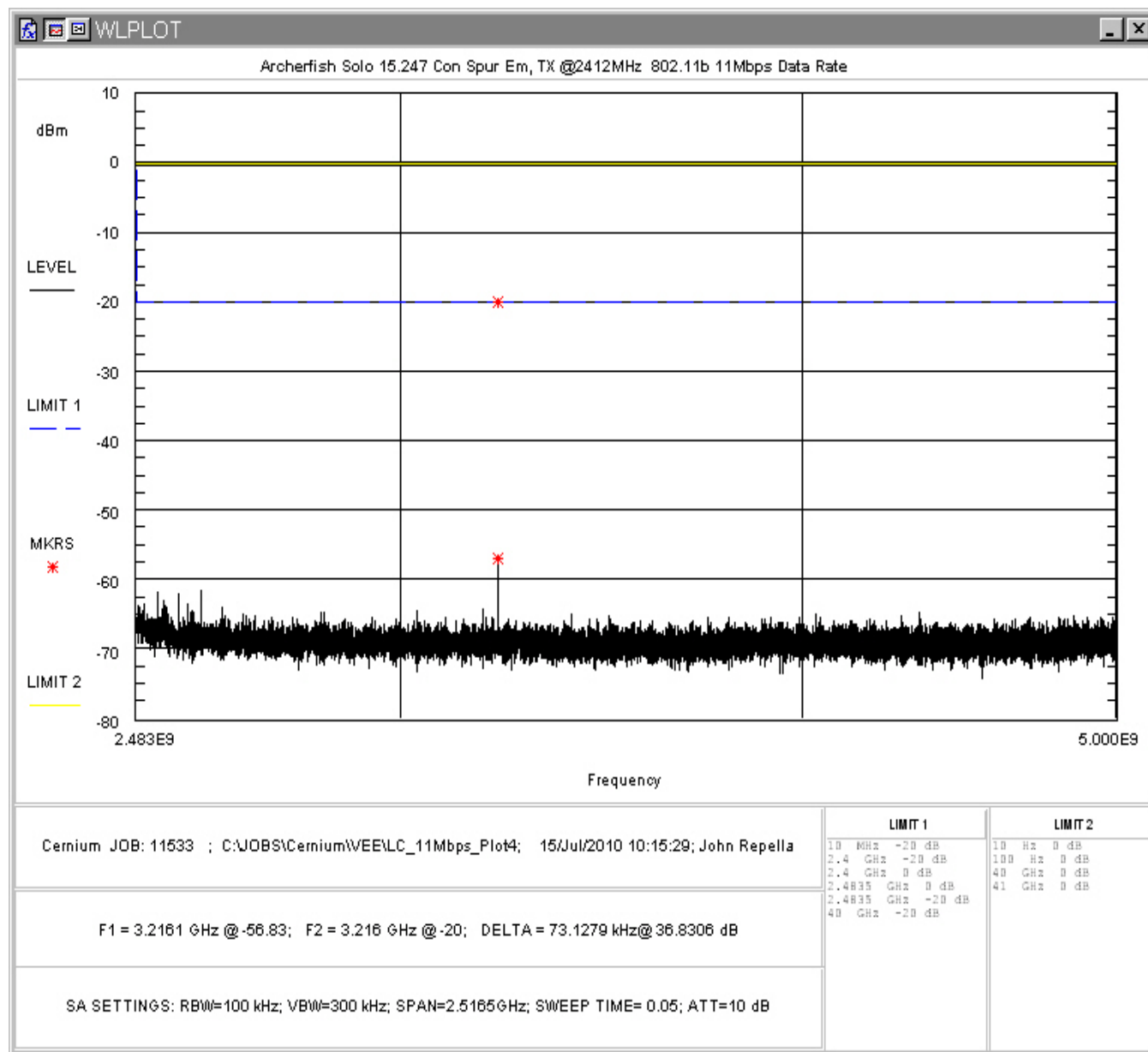
Figure 52: Conducted Spurious Emissions, 802.11b 11Mbps Low Channel, 2.483 - 5GHz
