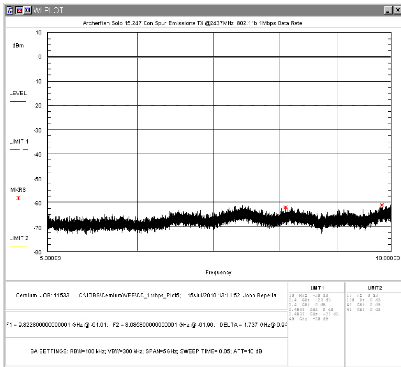
Figure 37: Conducted Spurious Emissions, 802.11b 1Mbps, Mid Channel 5 - 10GHz
