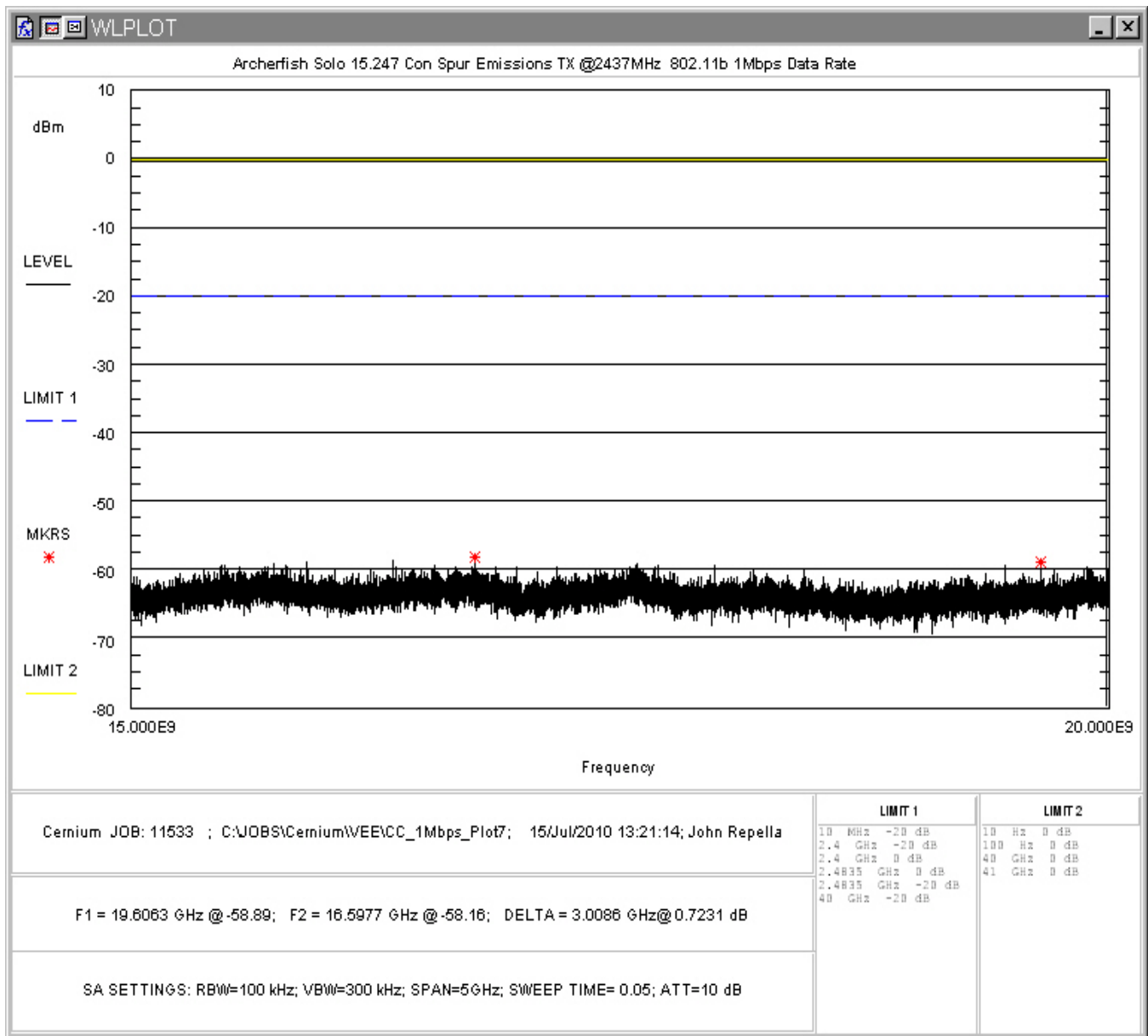
Figure 39: Conducted Spurious Emissions, 802.11b 1Mbps, Mid Channel 15 - 20GHz
