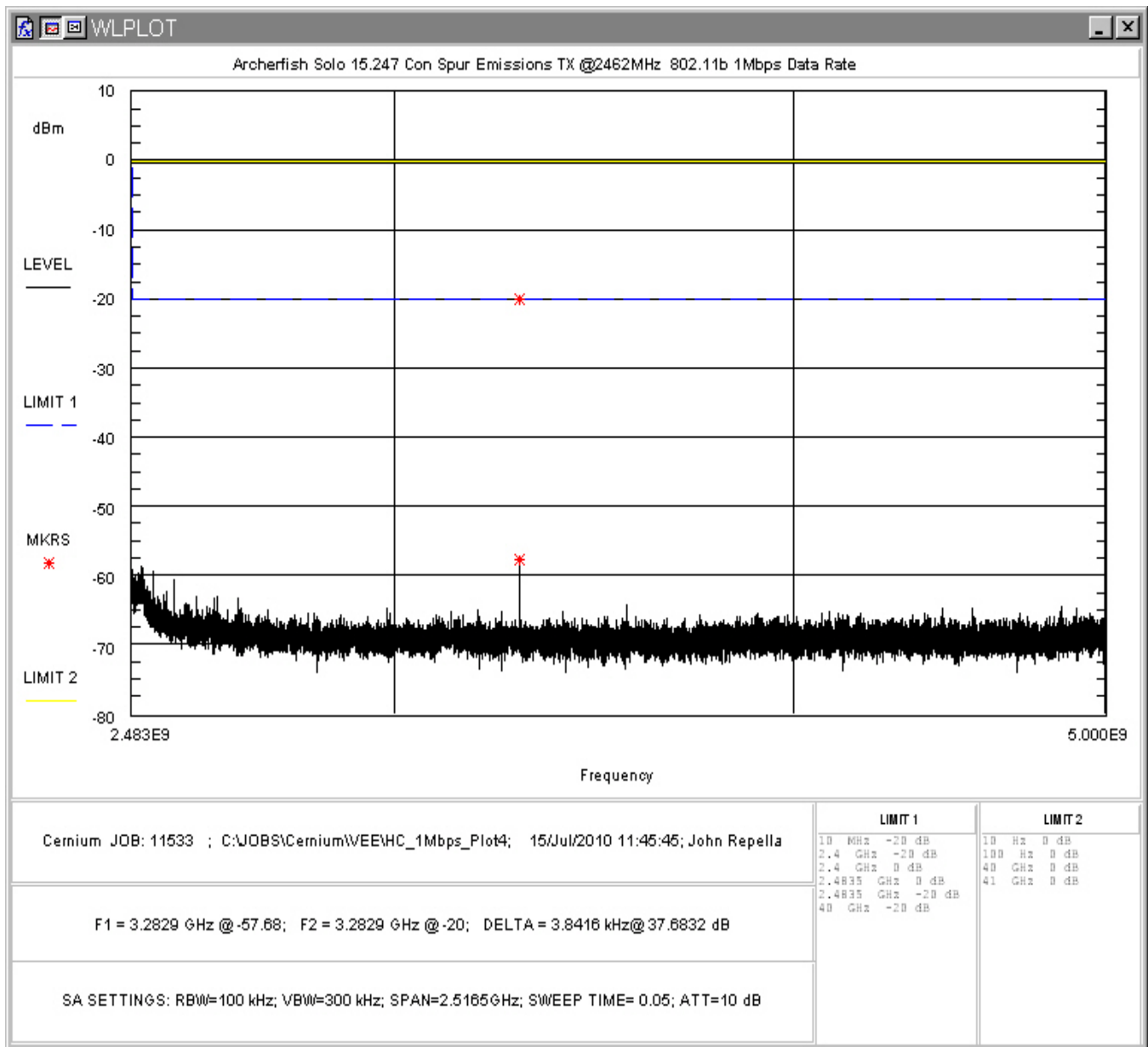
Figure 44: Conducted Spurious Emissions, 802.11b 1Mbps, High Channel 2.483 - 5GHz
