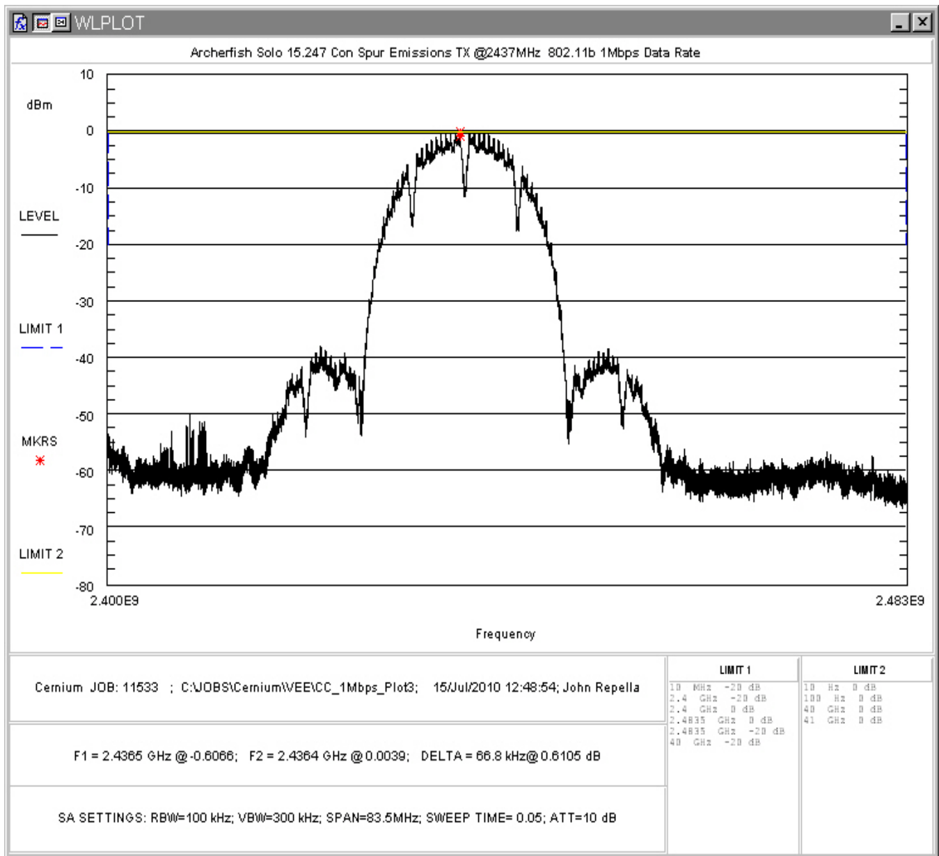
Figure 35: Conducted Spurious Emissions, 802.11b 1Mbps, Mid Channel 2.4 – 2.483GHz
