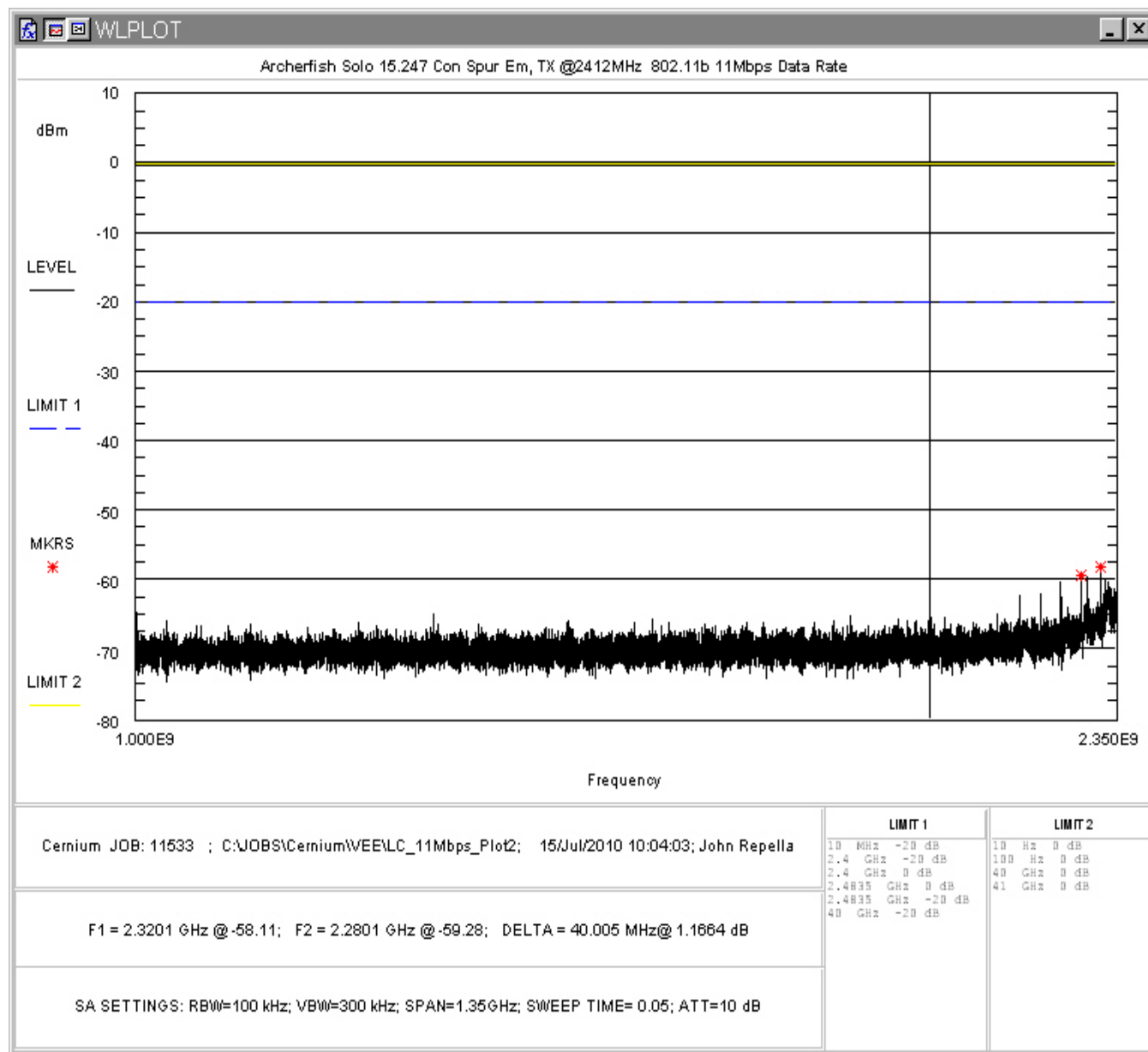
Figure 50: Conducted Spurious Emissions, 802.11b 11Mbps Low Channel, 1 – 2.35GHz
