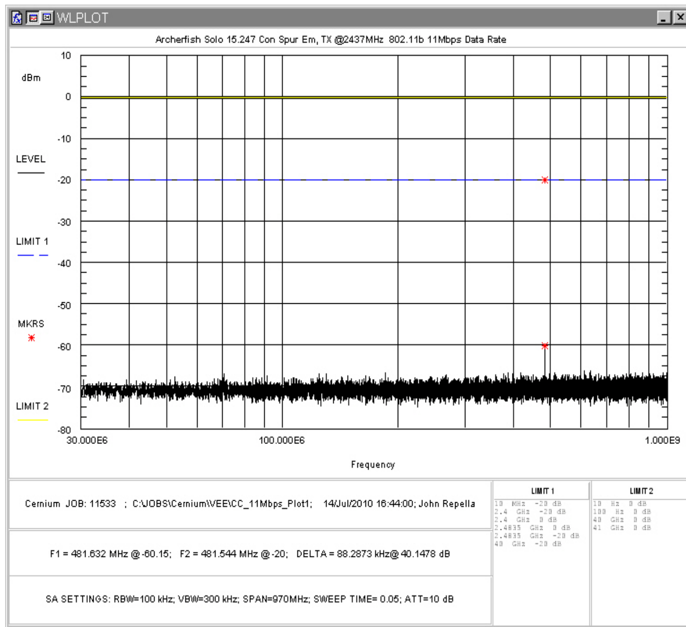
Figure 57: Conducted Spurious Emissions, 802.11b 11Mbps, Mid Channel 30 - 1000MHz
