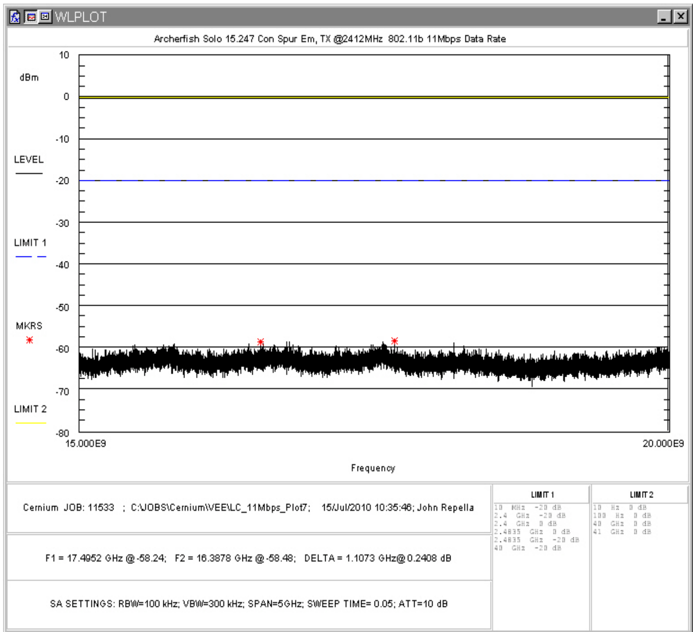
Figure 55: Conducted Spurious Emissions, 802.11b 11Mbps Low Channel, 15 - 20GHz
