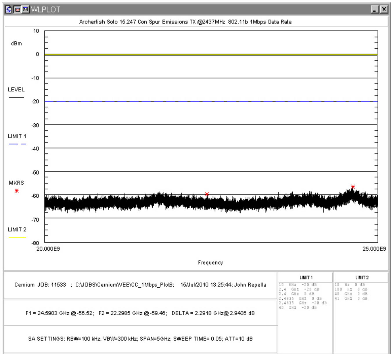
Figure 40: Conducted Spurious Emissions, 802.11b 1Mbps, Mid Channel 20 - 25GHz
