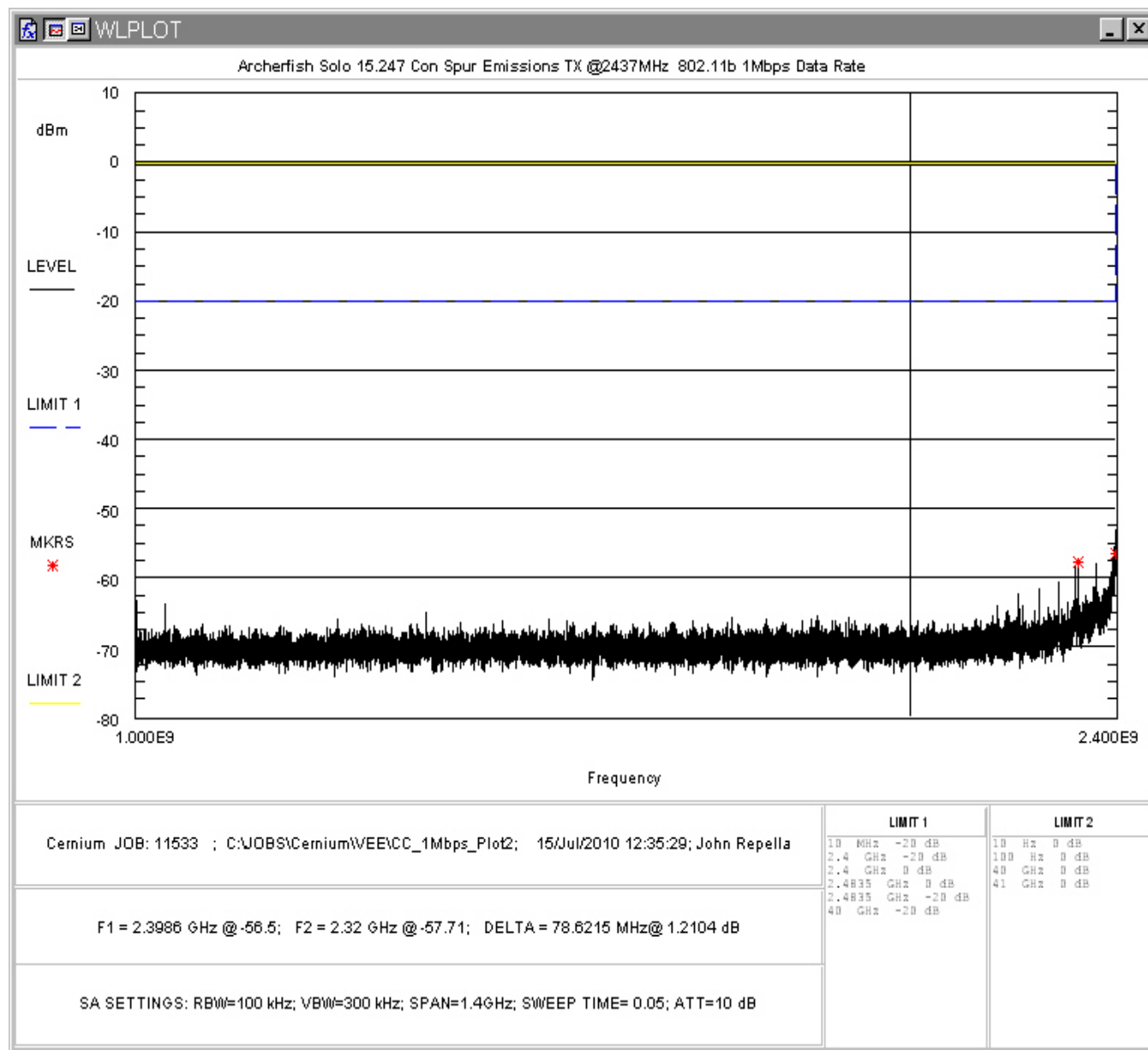
Figure 34: Conducted Spurious Emissions, 802.11b 1Mbps, Mid Channel 1 – 2.4GHz
