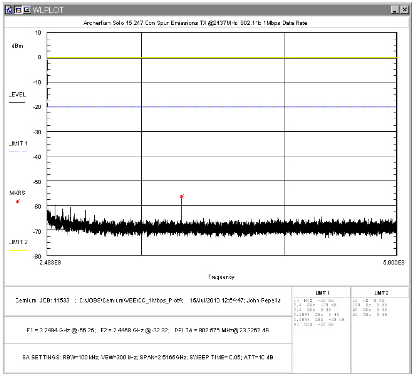
Figure 36: Conducted Spurious Emissions, 802.11b 1Mbps, Mid Channel 2.483 - 5GHz
