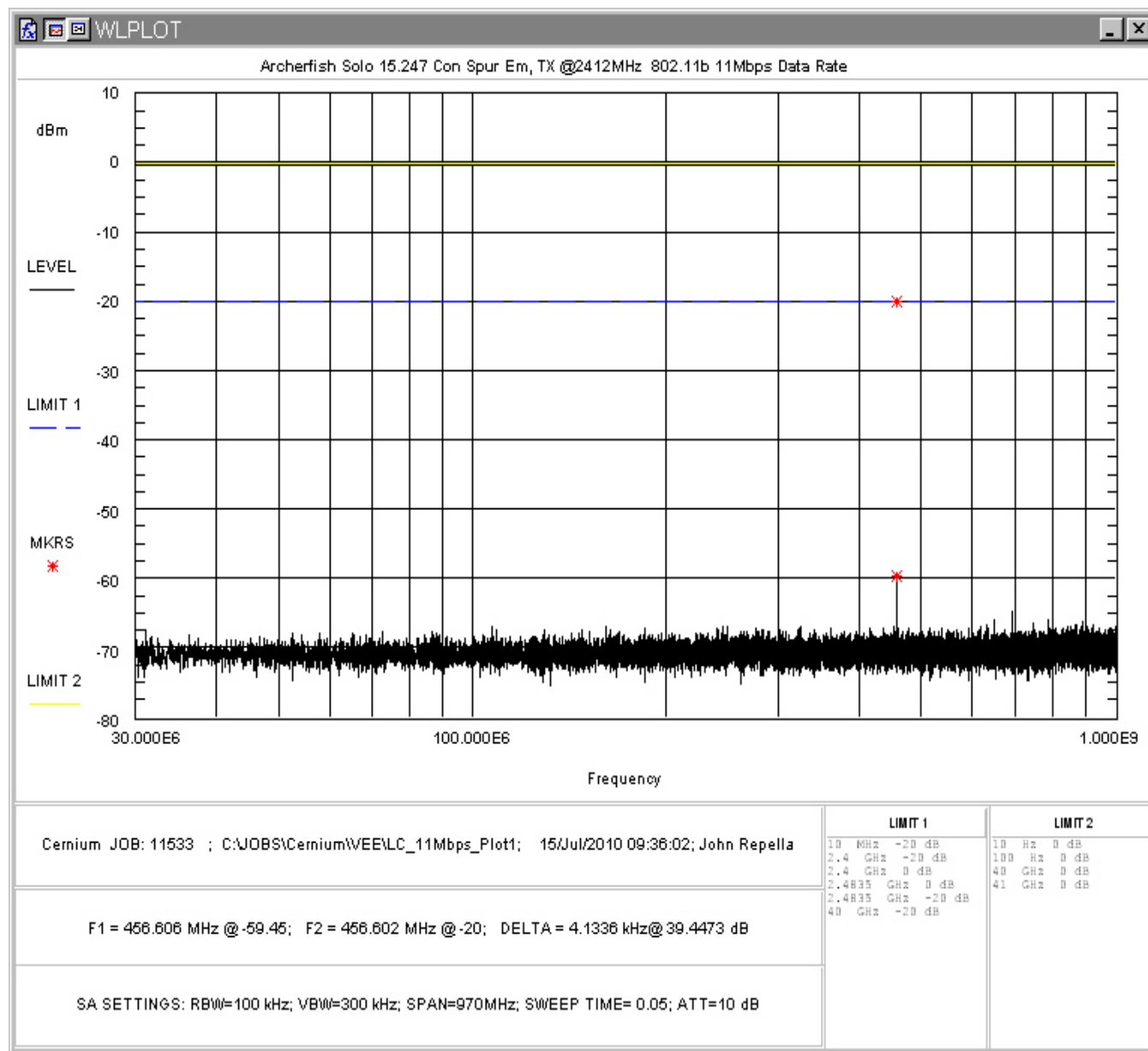
Figure 49: Conducted Spurious Emissions, 802.11b 11Mbps Low Channel, 30 - 1000MHz
