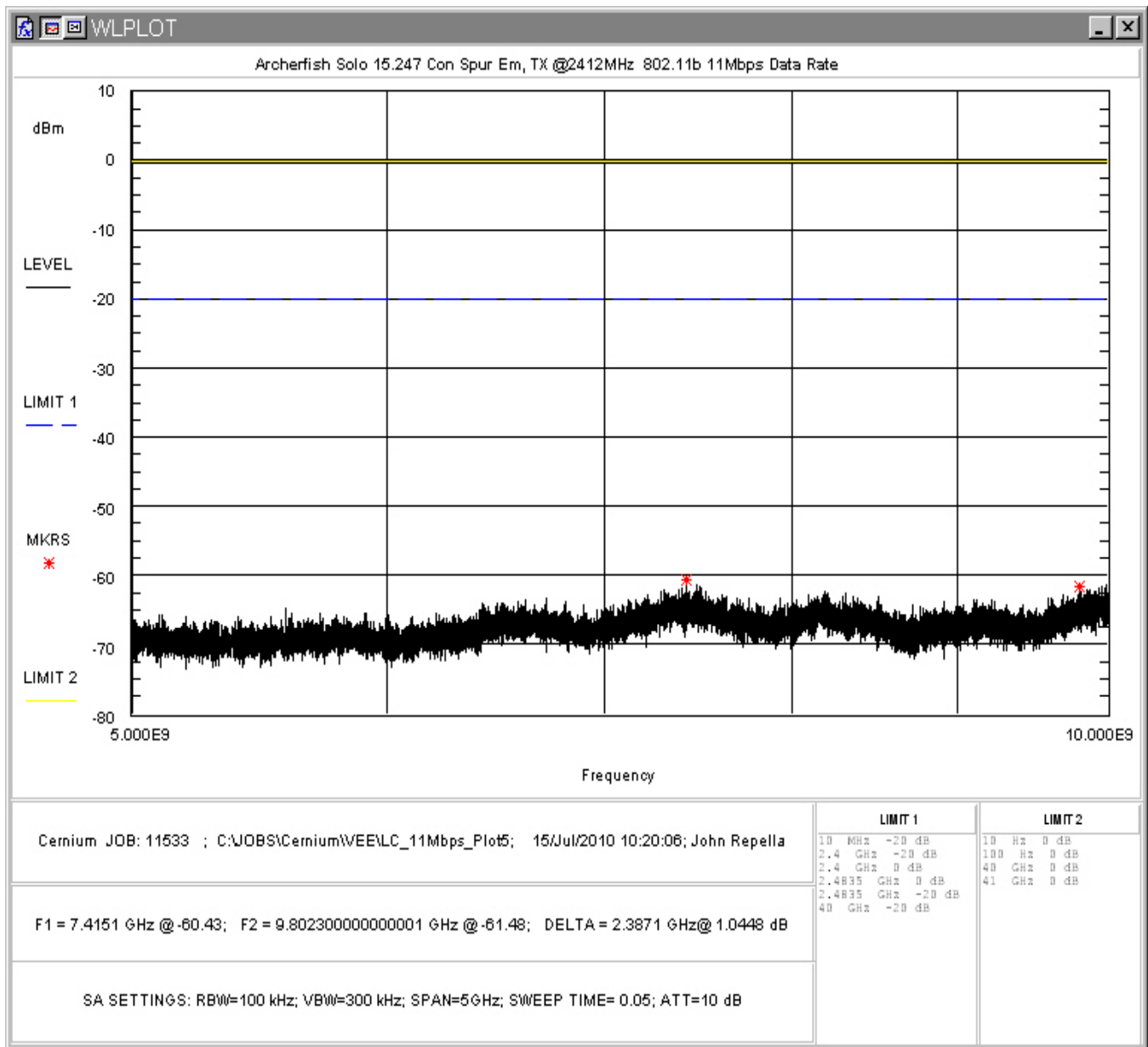
Figure 53: Conducted Spurious Emissions, 802.11b 11Mbps Low Channel, 5 - 10GHz
