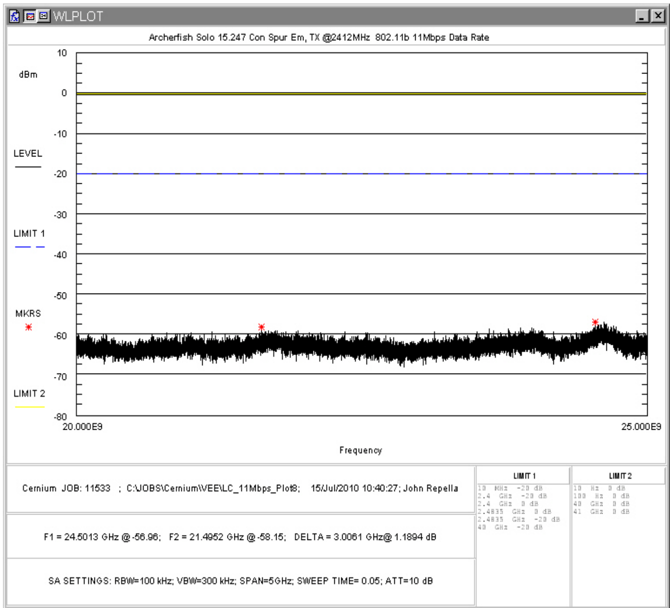
Figure 56: Conducted Spurious Emissions, 802.11b 11Mbps Low Channel, 20 - 25GHz
