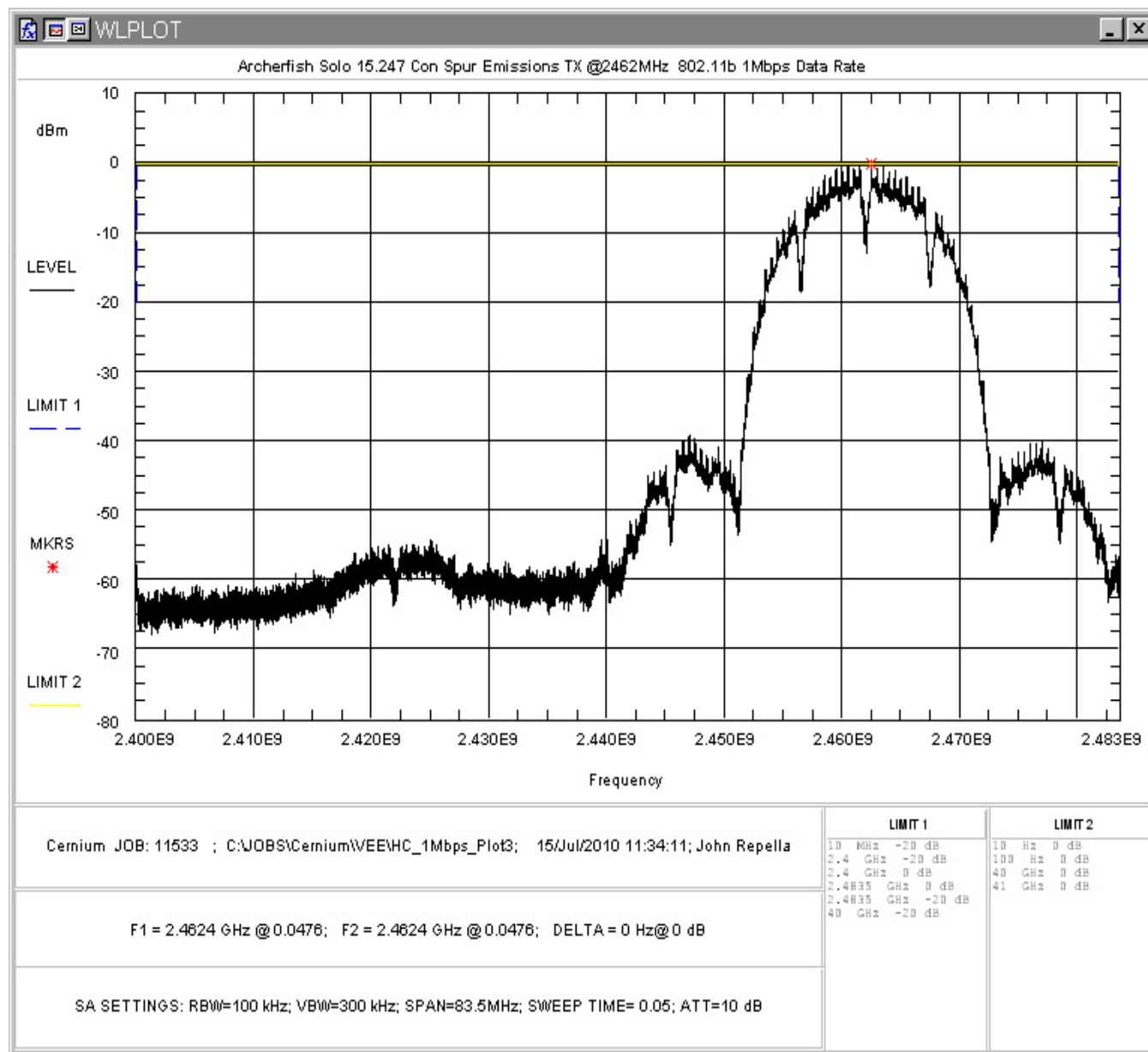
Figure 43: Conducted Spurious Emissions, 802.11b 1Mbps, High Channel 2.4 – 2.483GHz
