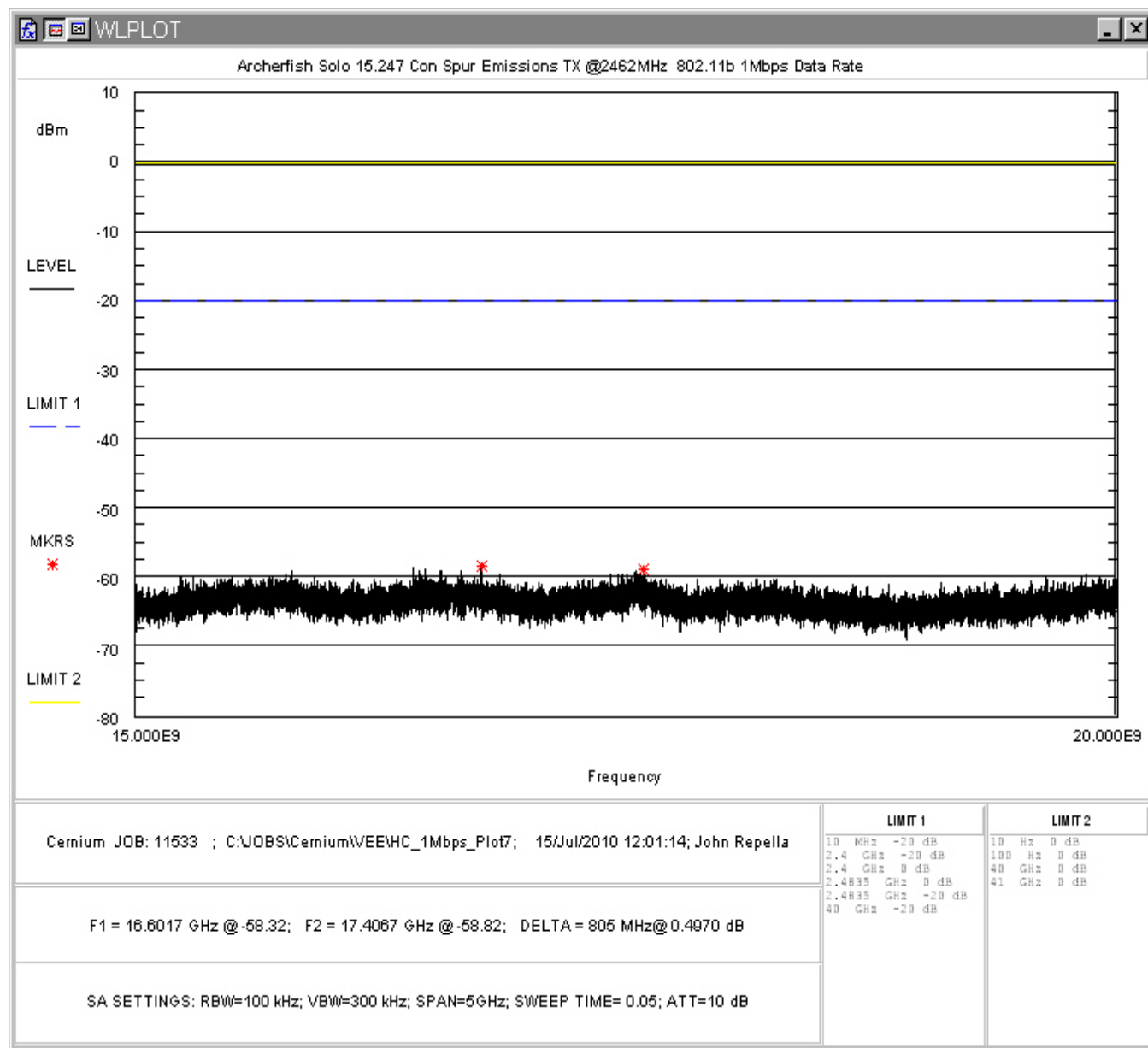
Figure 47: Conducted Spurious Emissions, 802.11b 1Mbps, High Channel 15 - 20GHz
