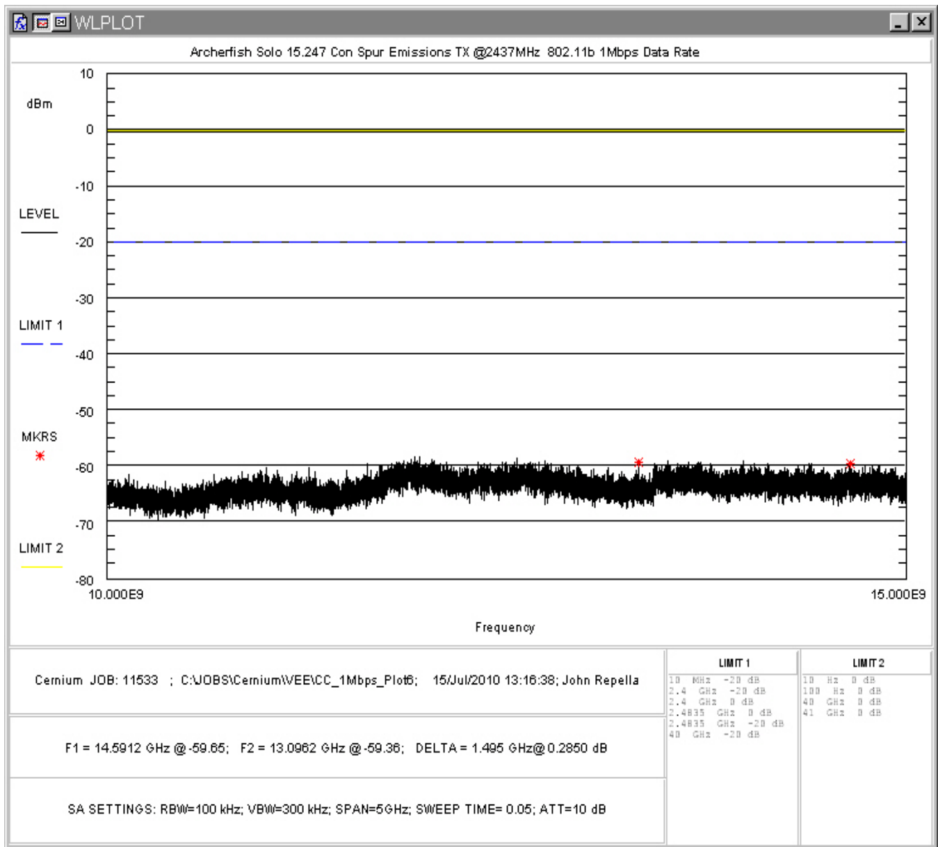
Figure 38: Conducted Spurious Emissions, 802.11b 1Mbps, Mid Channel 10 - 15GHz
