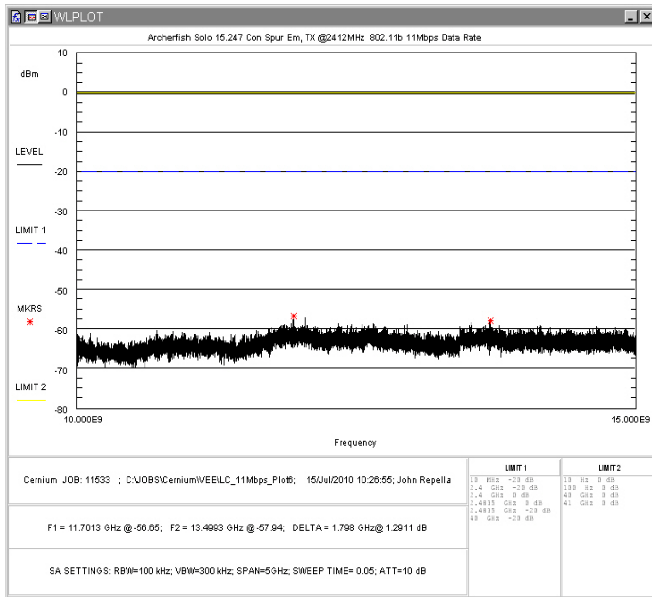
Figure 54: Conducted Spurious Emissions, 802.11b 11Mbps Low Channel, 10 - 15GHz
