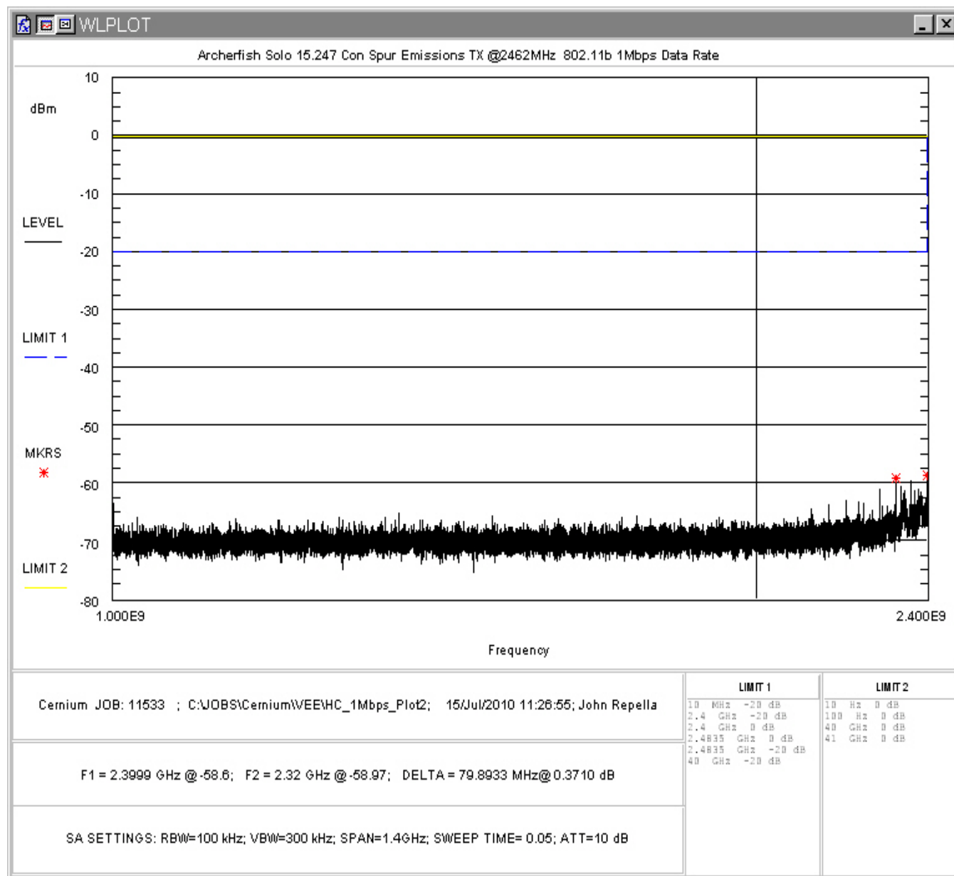
Figure 42: Conducted Spurious Emissions, 802.11b 1Mbps, High Channel 1 – 2.4GHz
