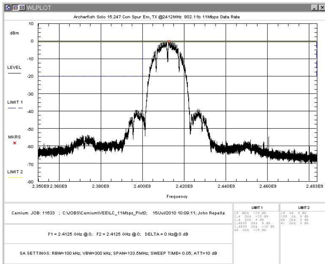
Figure 51: Conducted Spurious Emissions, 802.11b 11Mbps Low Channel, 2.35 – 2.483GHz
