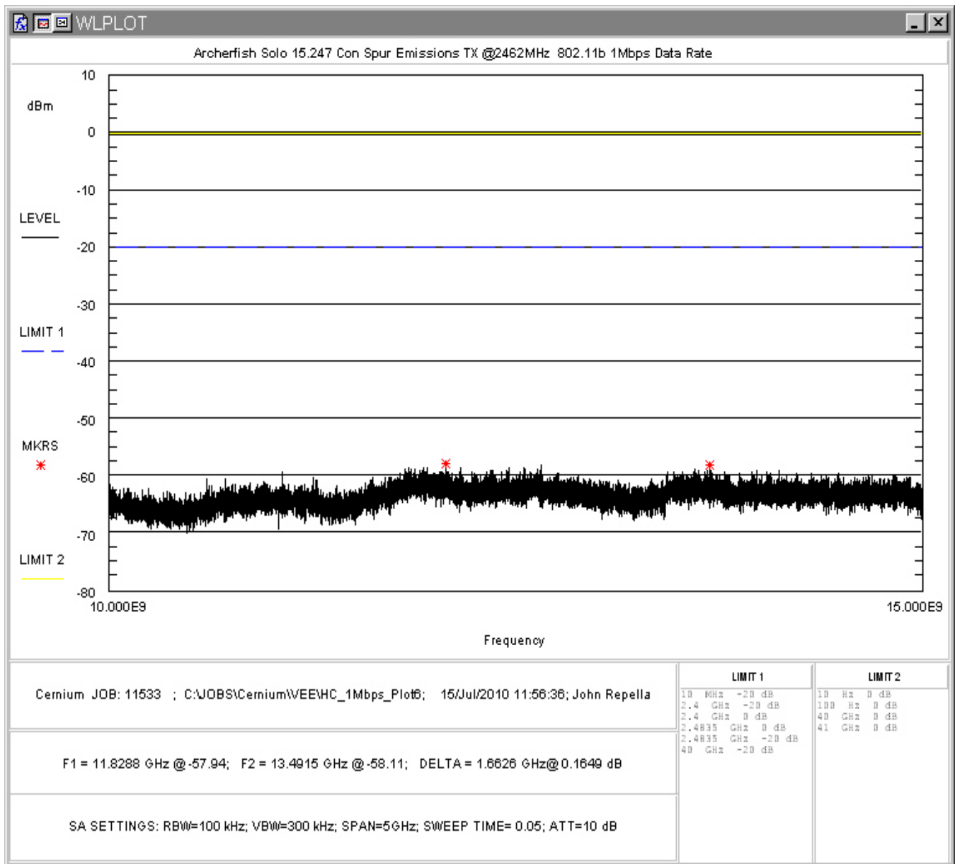
Figure 46: Conducted Spurious Emissions, 802.11b 1Mbps, High Channel 10 - 15GHz
