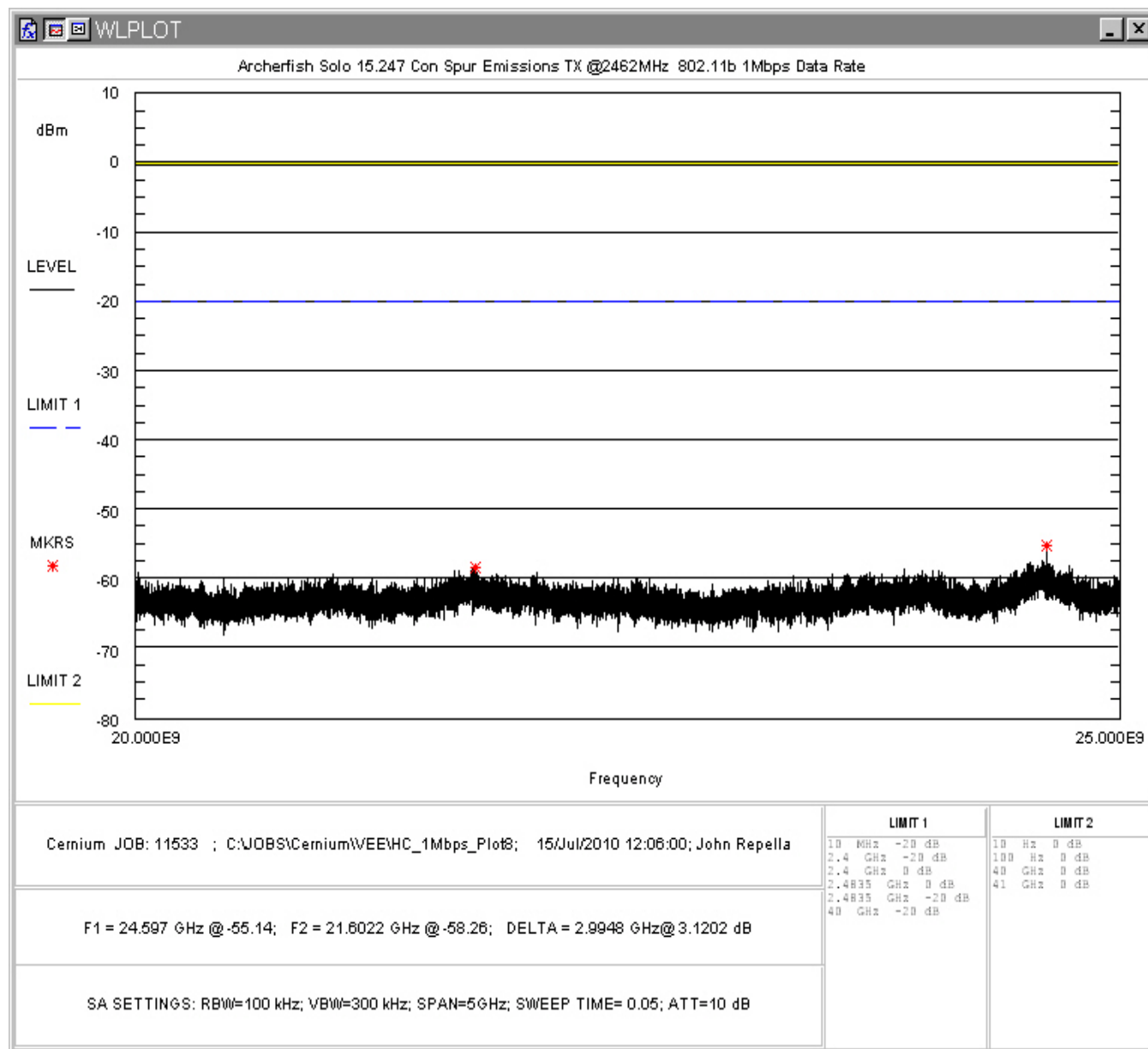
Figure 48: Conducted Spurious Emissions, 802.11b 1Mbps, High Channel 20 - 25GHz
