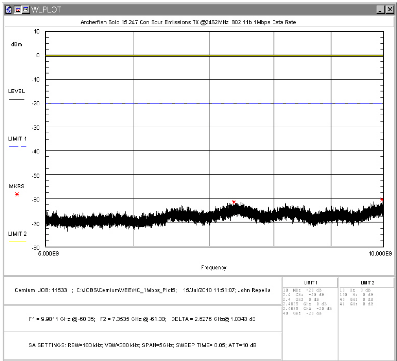
Figure 45: Conducted Spurious Emissions, 802.11b 1Mbps, High Channel 5 - 10GHz
