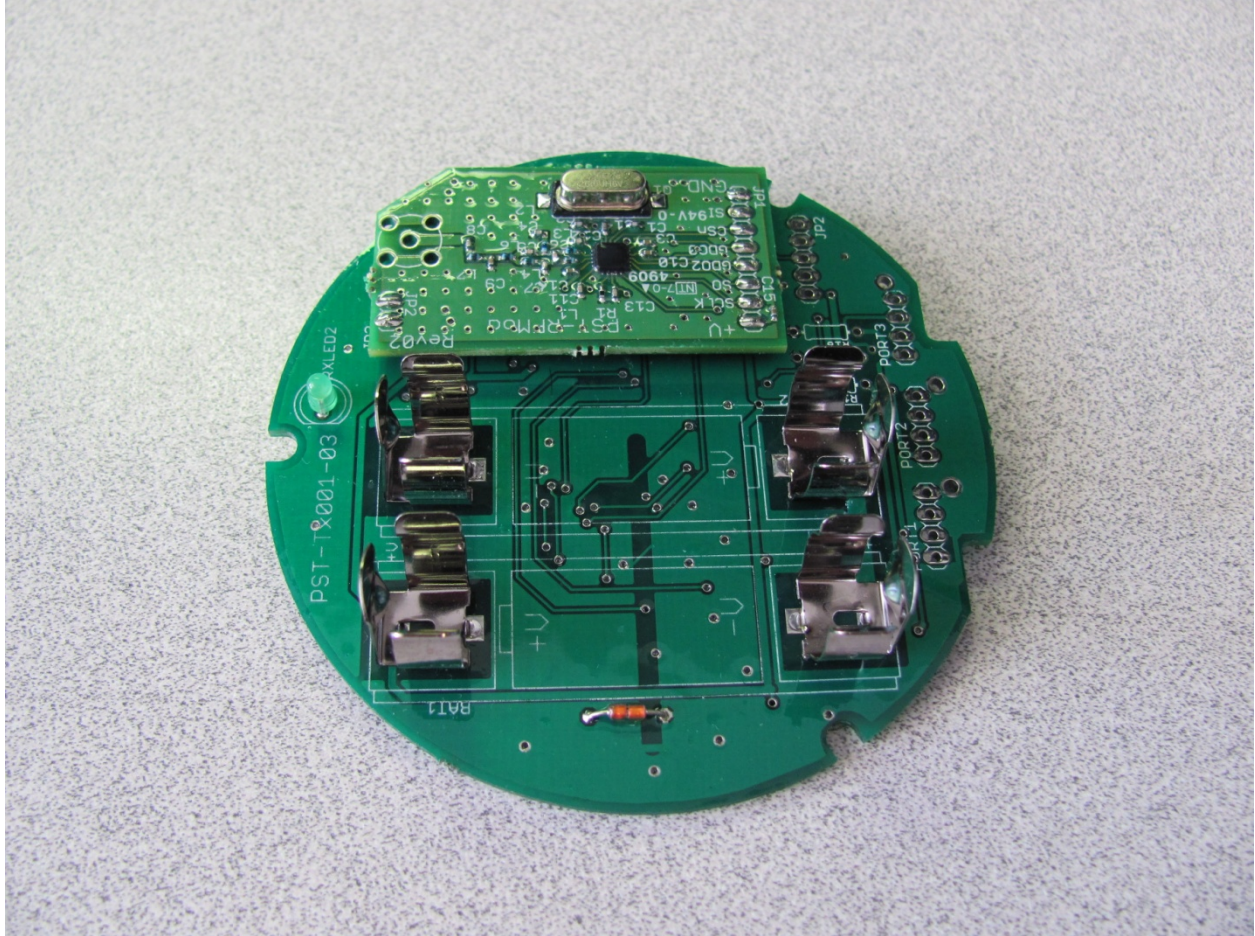
Figure 5 PST-TX001 Assembly
