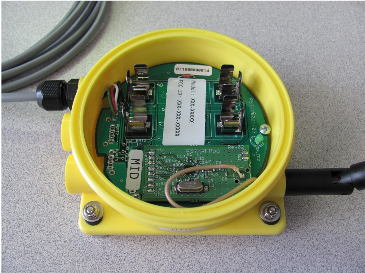
Figure 6 Completed Assembly
