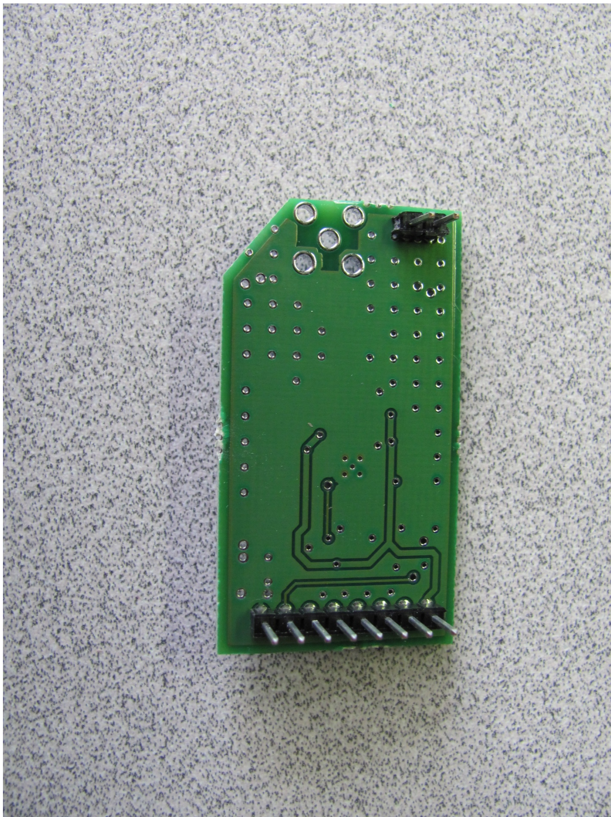
Figure 4 PST RF-MOD Bottom Side
