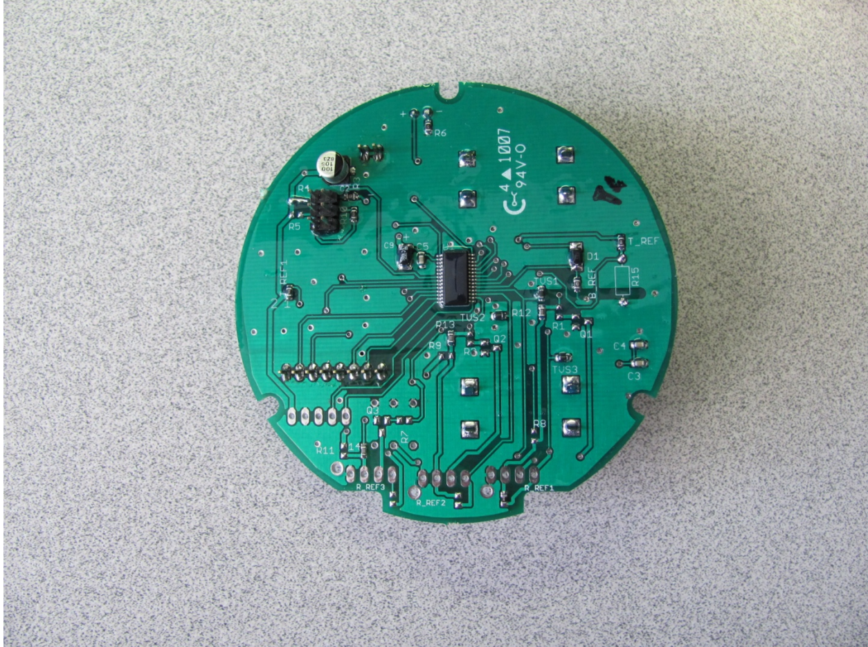
Figure 1 PST-TX001-03 main board bottom
