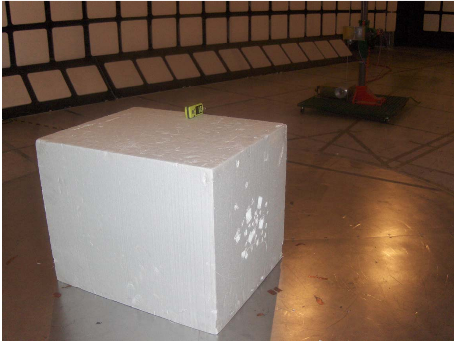
Photo #3: Test Setup for Radiated Emission Measurements @ 3m distance, EUT Orthogonal Position #3
