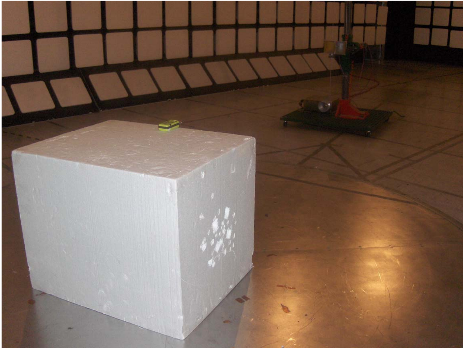
Photo #2: Test Setup for Radiated Emission Measurements @ 3m distance, EUT Orthogonal Position #2
