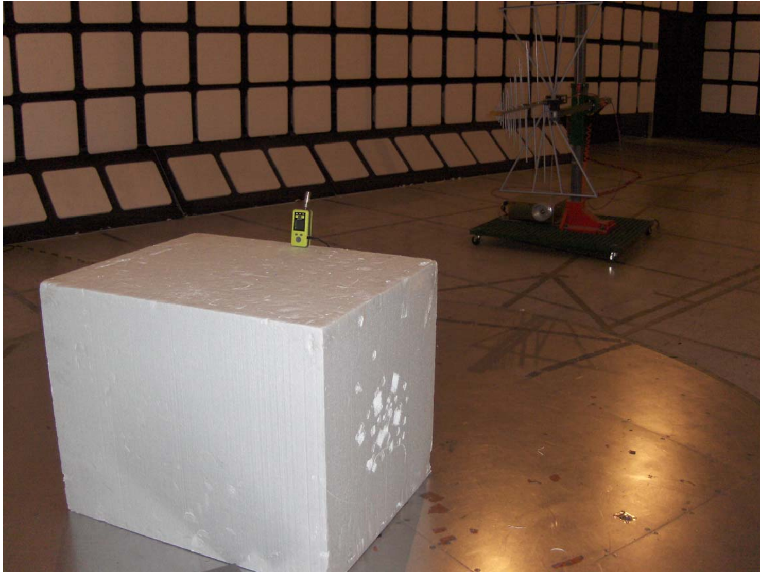
Photo #1: Test Setup for Radiated Emission Measurements @ 3m distance, EUT Orthogonal Position #1
