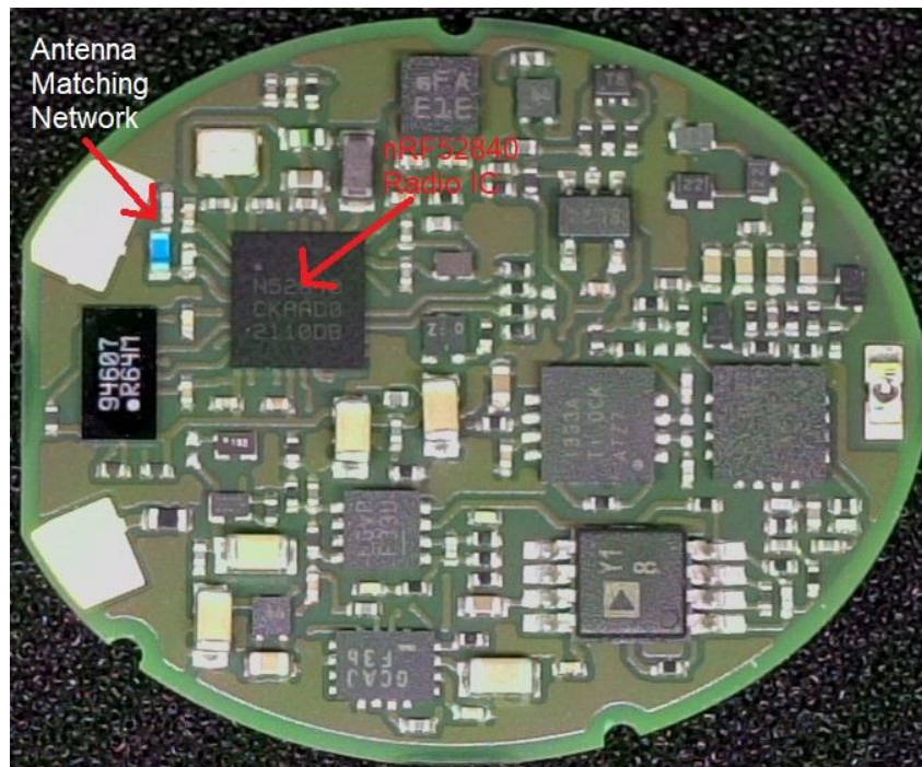
Figure 2: PCBA Top View
