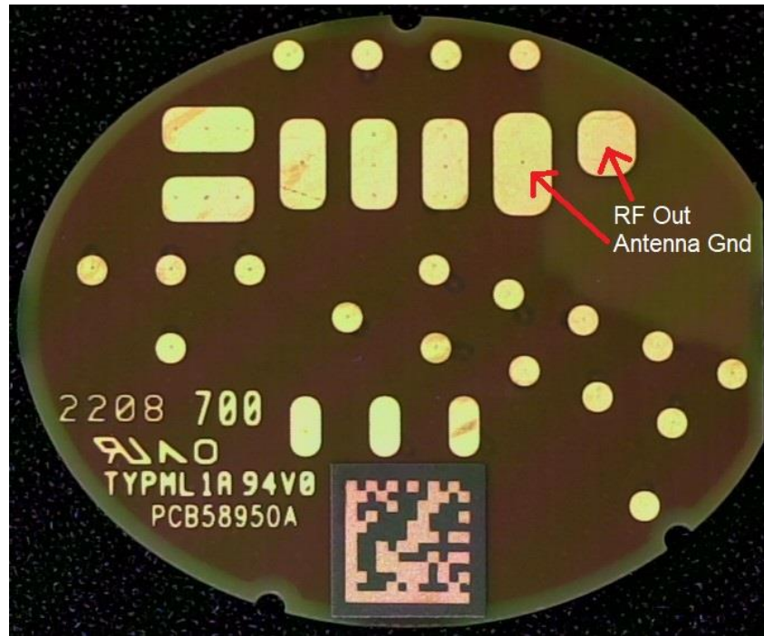
Figure 3: PCBA Bottom View
