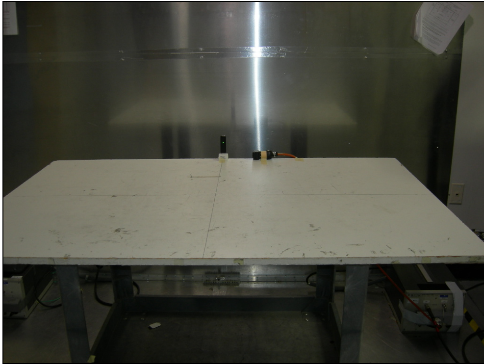
Figure 7: Conducted Emissions – Front View
