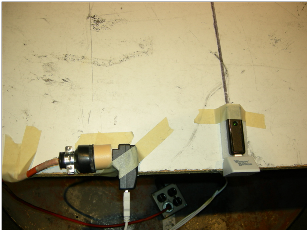
Figure 2: Radiated Emissions – X-Position
