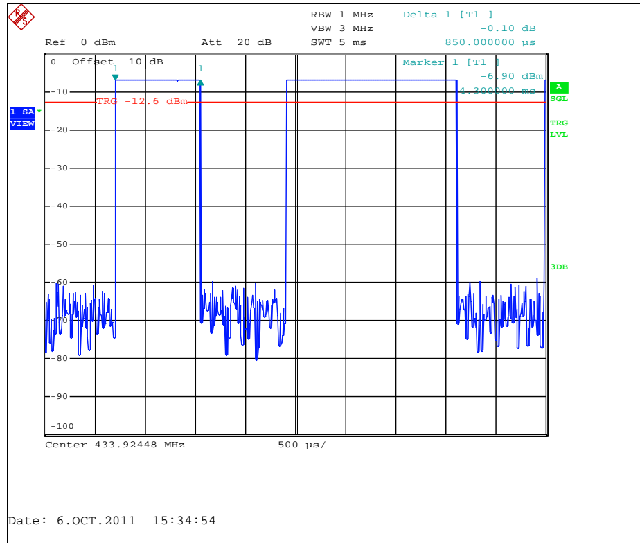
Figure 7.5.2-3: Duty Cycle – Pulse Width
