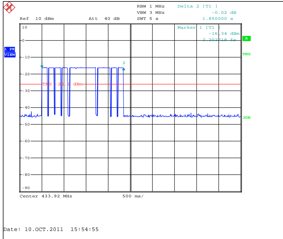
Figure 7.3.2-2: TX Hold Time – Automatically Activated
