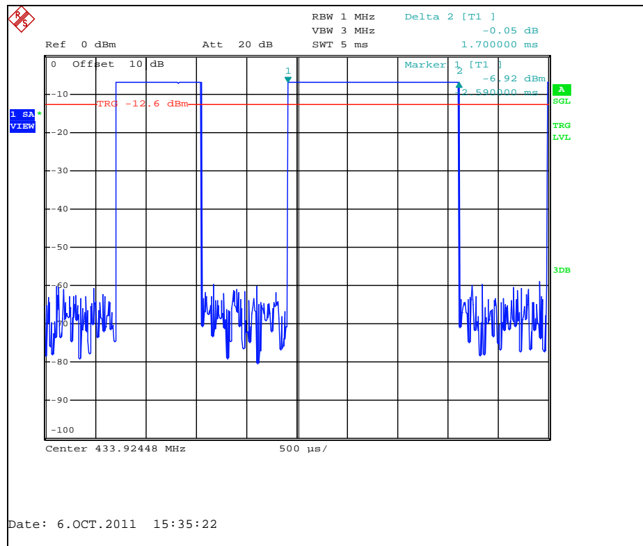
Figure 7.5.2-4: Duty Cycle – Pulse Width
