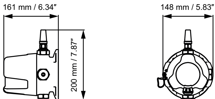
Polytron Repeater ISA with standard antenna
