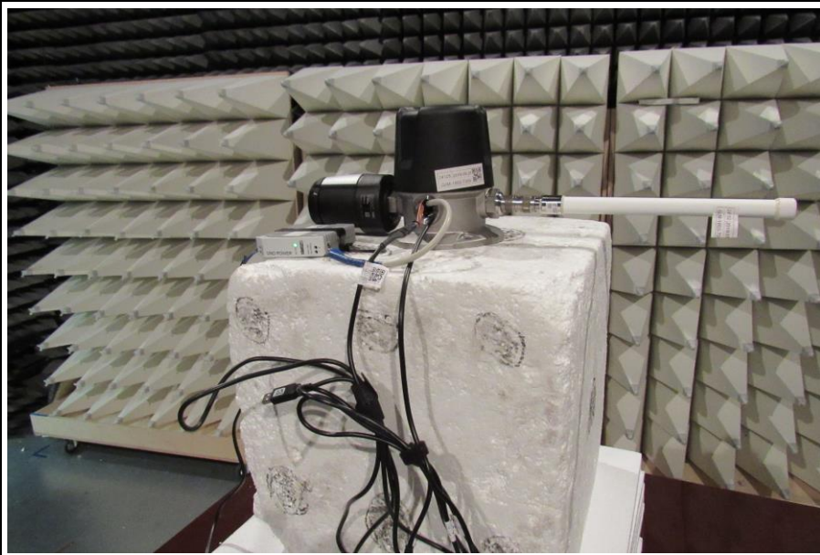
Testsetup above 1GHz EUT view
