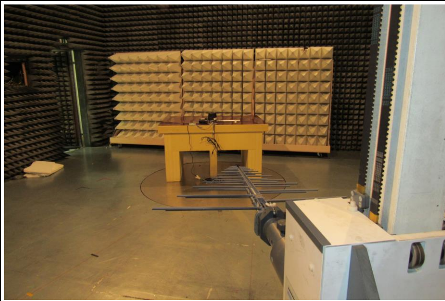
Testsetup above 200M
