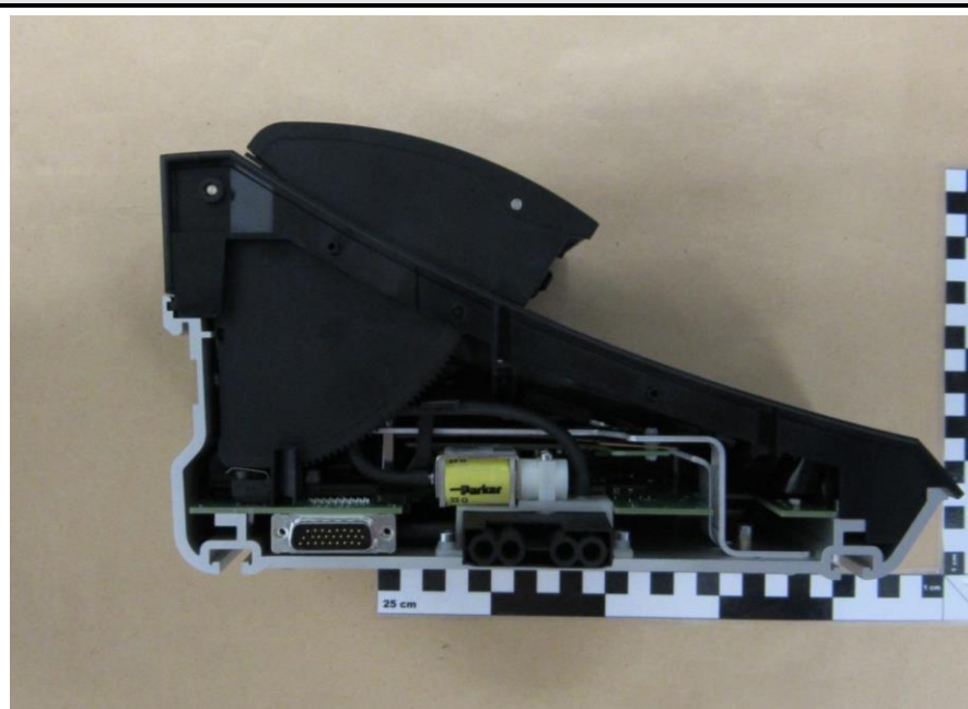
L-Side View
