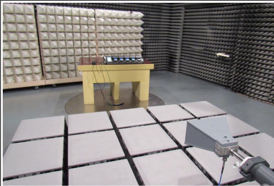
TEST SETUP 3 EUT CONFIGURATION 2 1 RE 1-3.7 GHz
