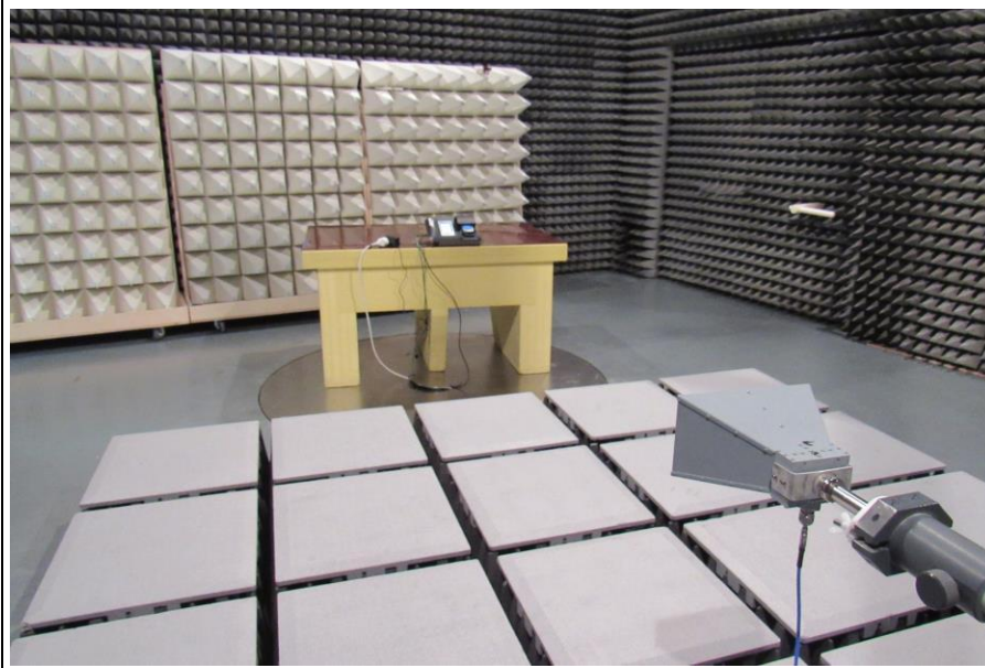
TEST SETUP 3 EUT CONFIGURATION 1 1 RE 1-3.7 GHz
