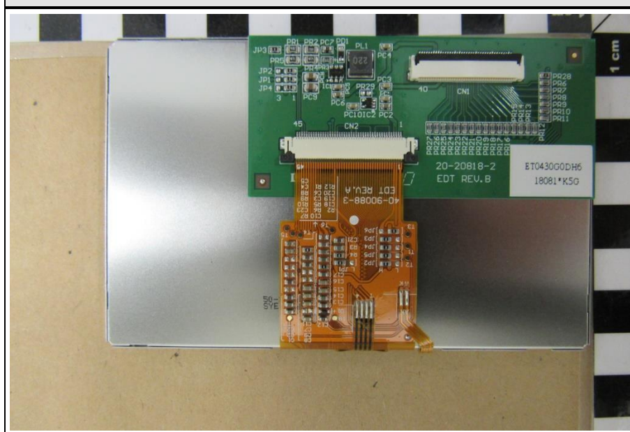
LCD Bottom View
