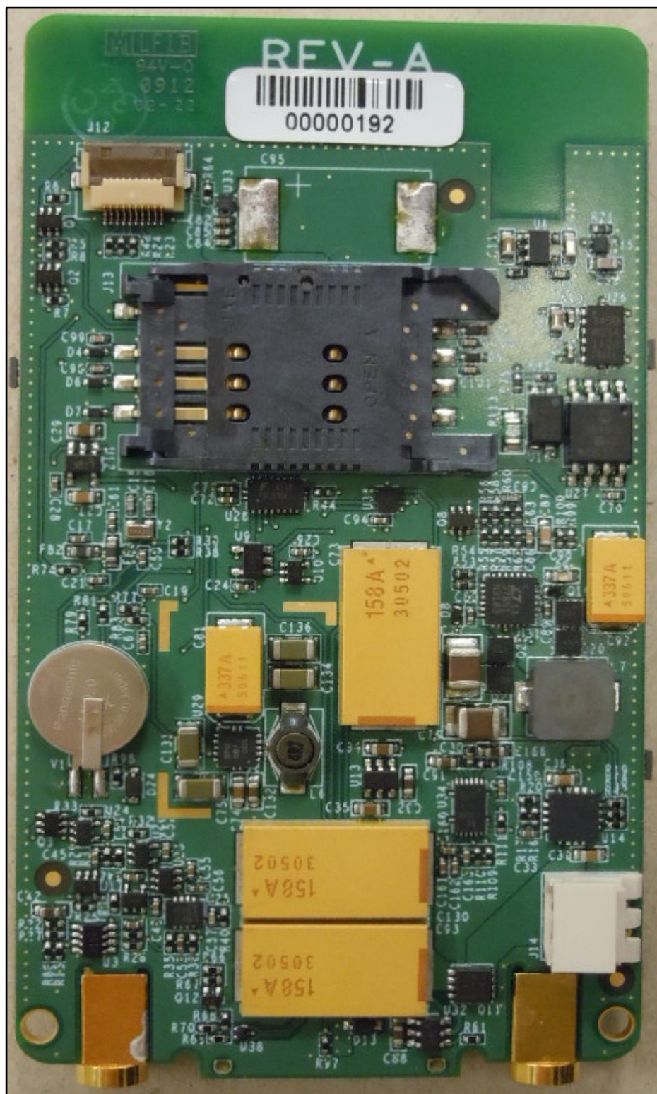
Panther PCB (Bottom Side - RefDes resolution)
