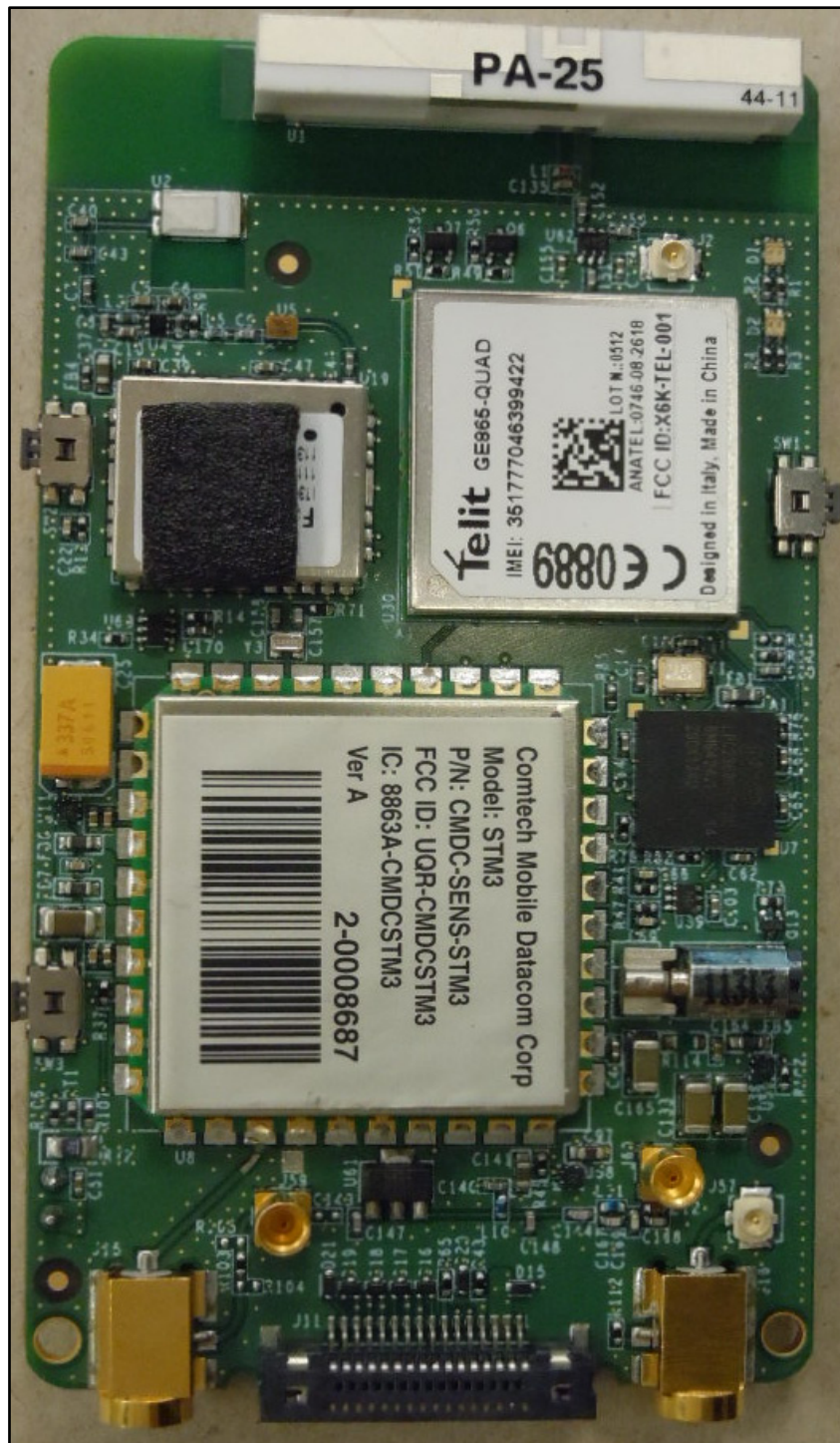
Panther PCB (Top Side – RefDes resolution, Transmitters in place)
