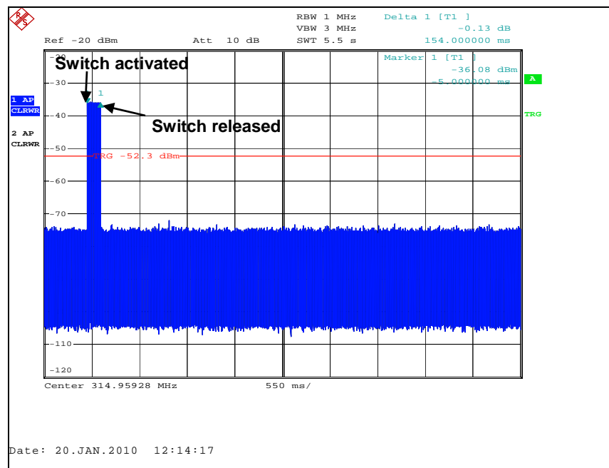
Figure 7.3.2-1: Transmitter Hold Time
