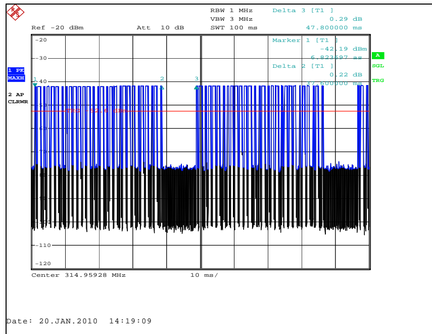
Figure 7.5.2-1: Pulse Train Period (T)
