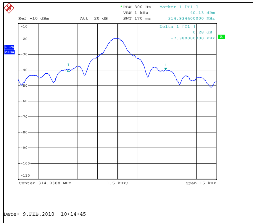
Figure 7.4.2-1: Occupied Bandwidth – 20dB
