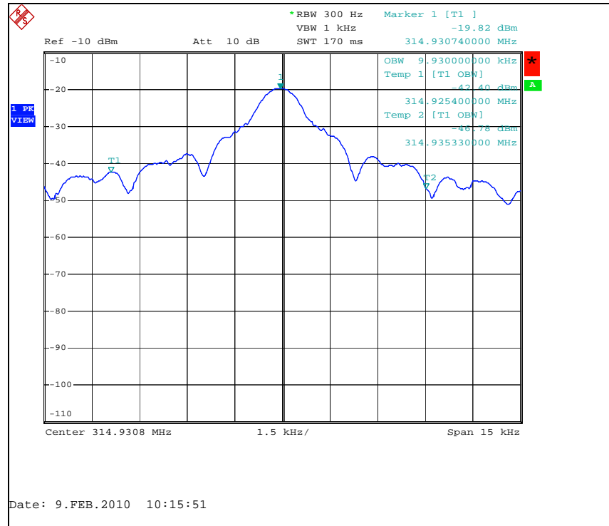
Figure 7.4.2-2: Occupied Bandwidth – 99%
