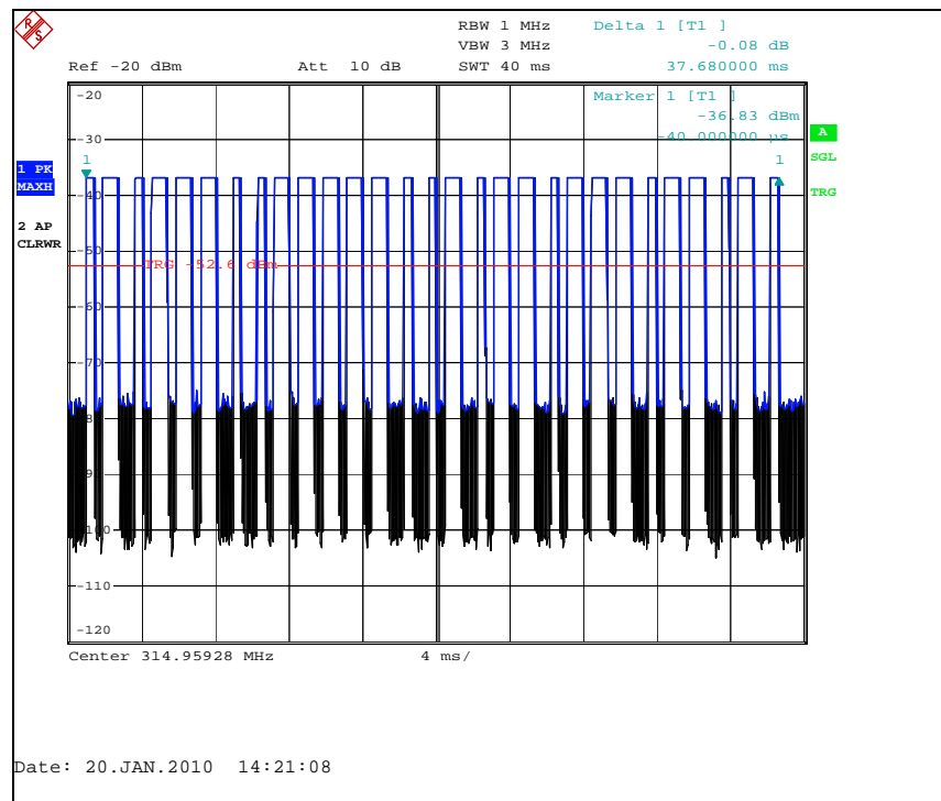
Figure 7.5.2-2: Pulse Train ( N_1 & N_2 )
