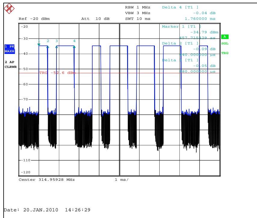
Figure 7.5.2-3: Pulse Width ( T_1 & T_2 )
