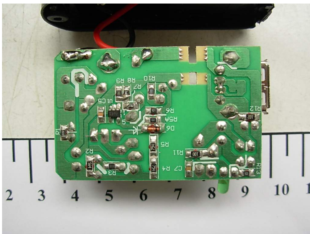
FIGURE 10 SIPOD IP WALKIE TALKIE (M/N: C200) ADAPTER MAIN BOARD (SOLDERED SIDE)
