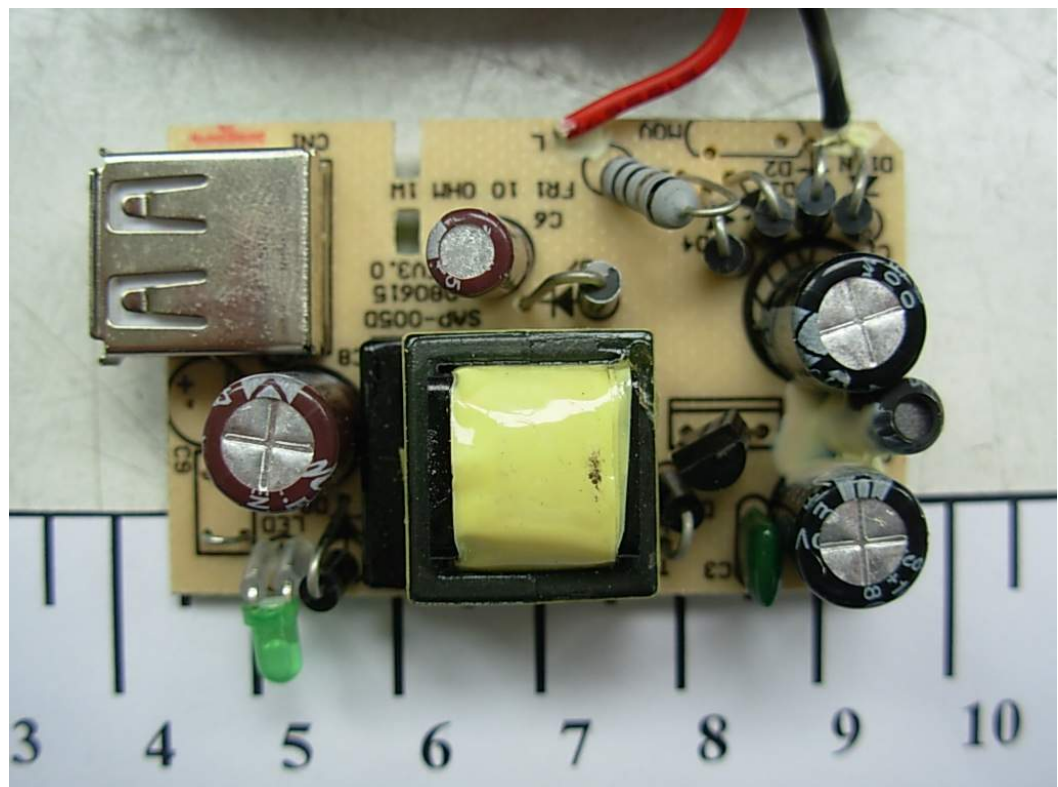
FIGURE 9 SIPOD IP WALKIE TALKIE (M/N: C200) ADAPTER MAIN BOARD (COMPONENT SIDE)
