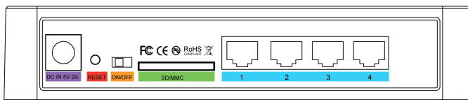
Figure 2: Back Panel of the Gateway
