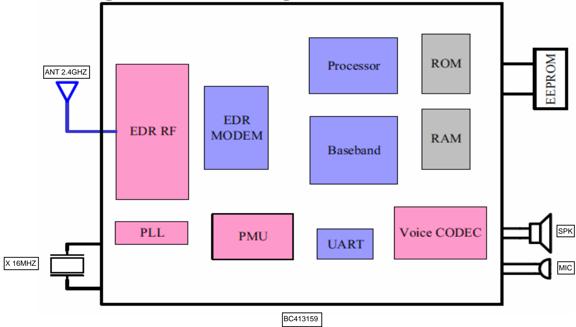
Figure 1: Functional Block Diagram
