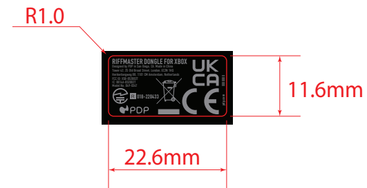
DONGLE LABEL
